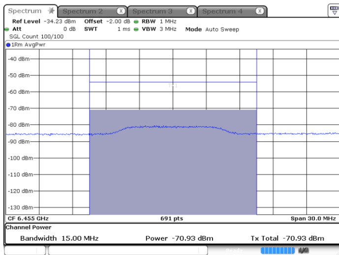
802.11ax (HE20)-Channel 101
