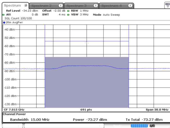
802.11ax (HE20)-Channel 213
