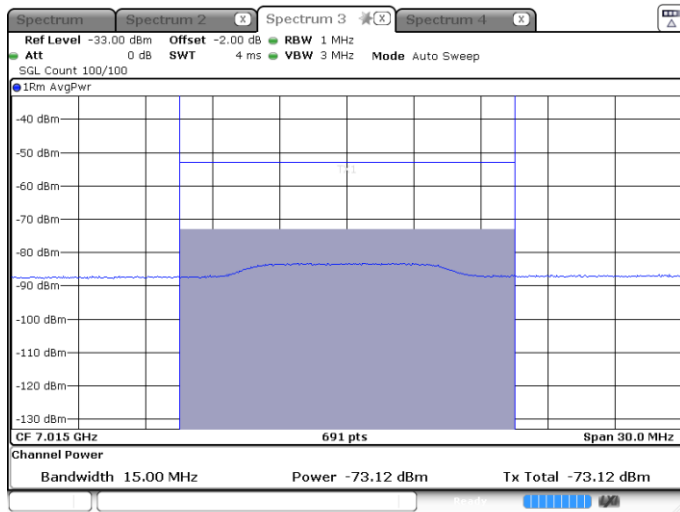
802.11ax (HE20)-Channel 213
