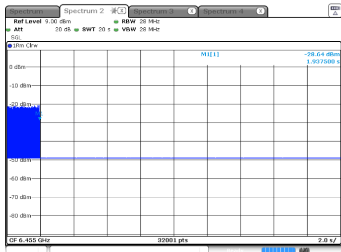
802.11ax (HE20)-Channel 101
