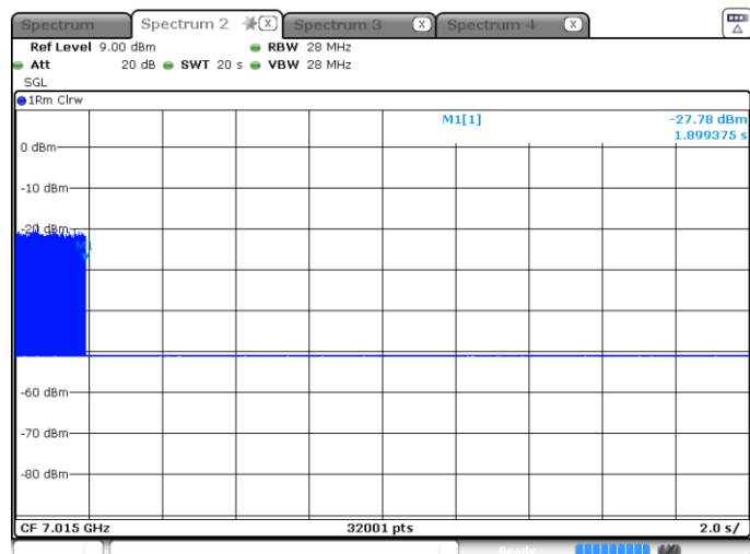
802.11ax (HE20)-Channel 213
