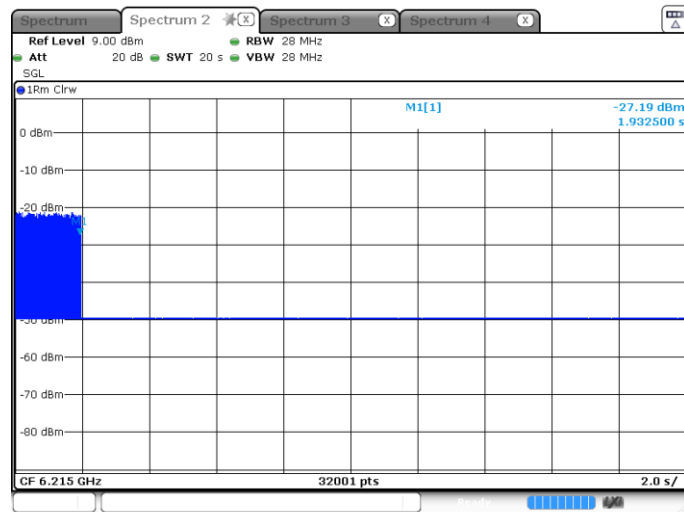
802.11ax (HE20)-Channel 53
