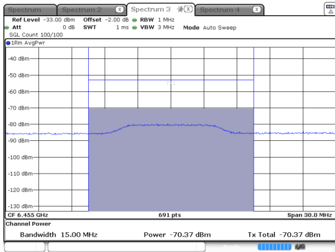
802.11ax (HE20)-Channel 101
