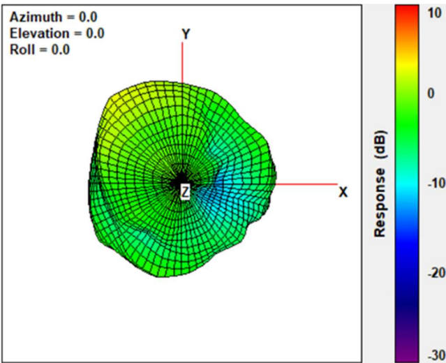
Max Antenna 3D Radiation Pattern 5150-5250 MHz
