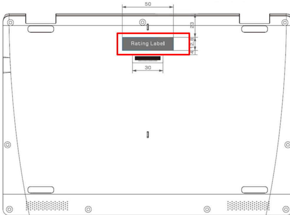
Label Placement Location (EUT Bottom View)
