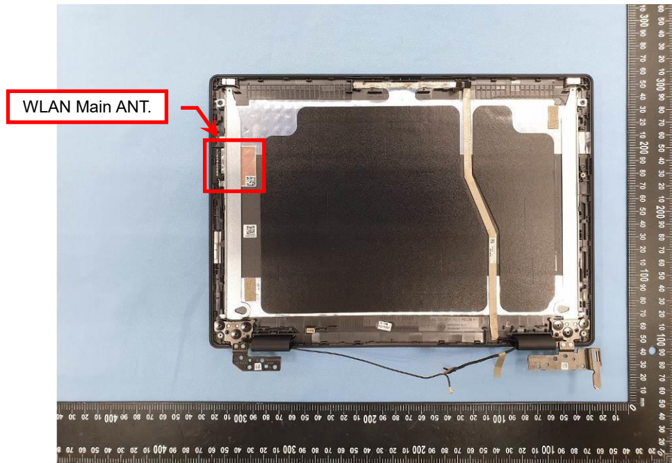
EUT Photo (22) Platform Model Number: CR1104CTA, CR1104FTA, CR1104FG, CR1104CG
