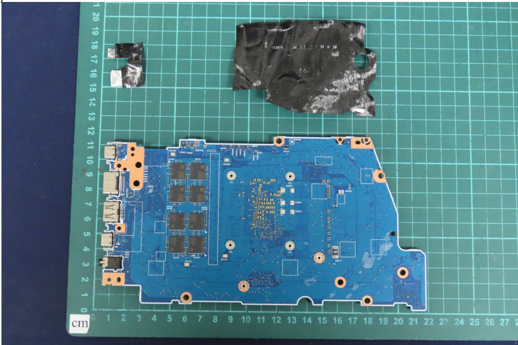
(35)EUT Photo
