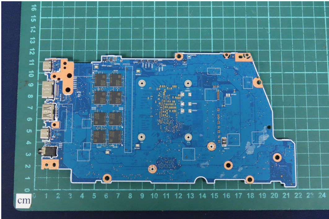
(36)EUT Photo
