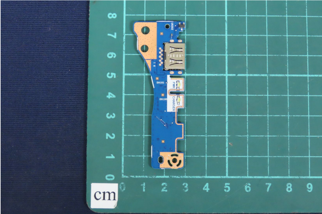
(30)EUT Photo
