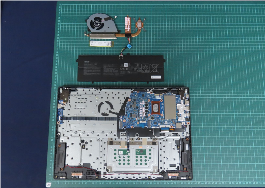
(19)EUT Photo
