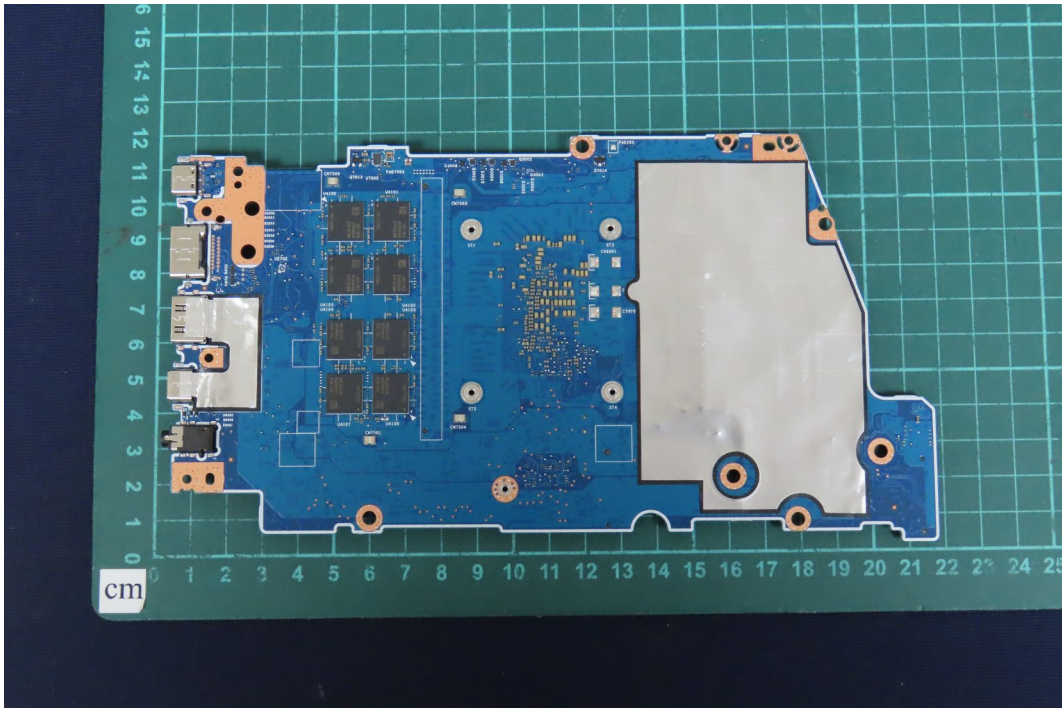
(34)EUT Photo
