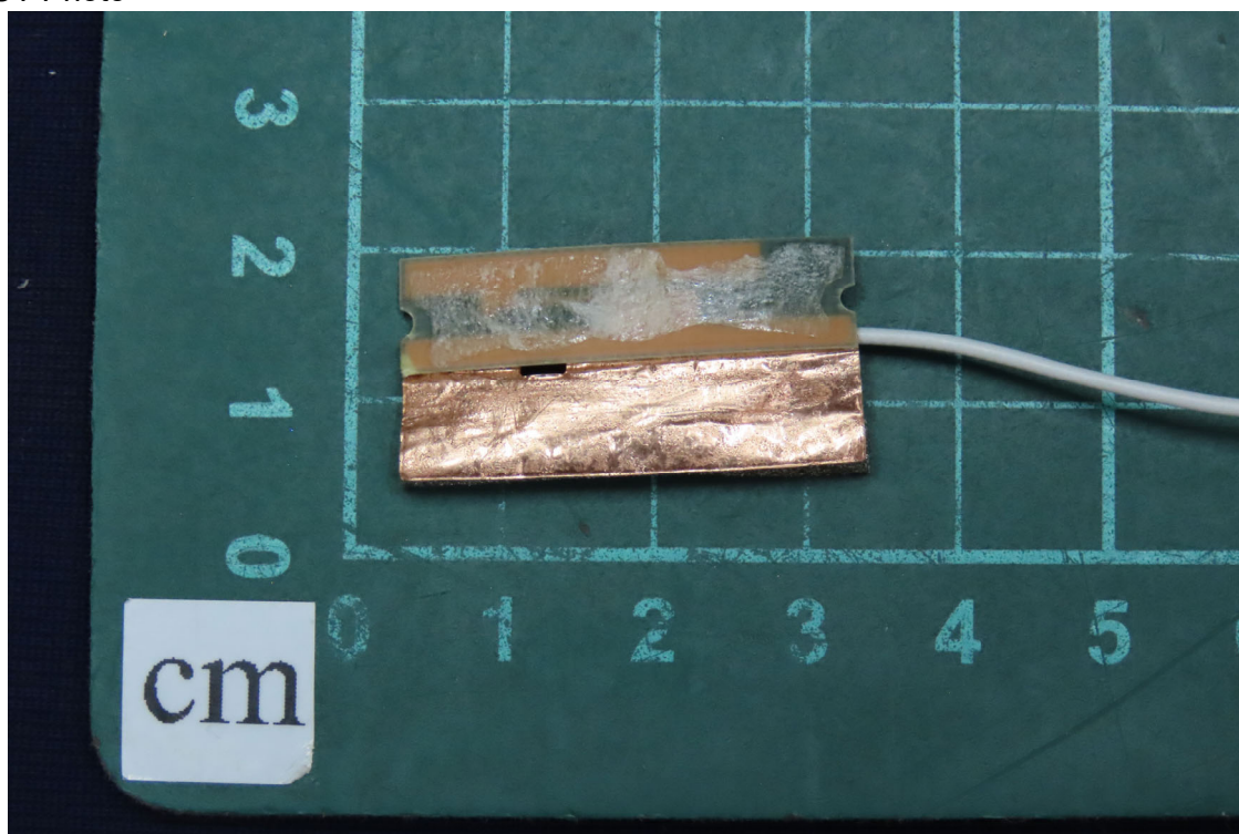
(11) EUT Photo
