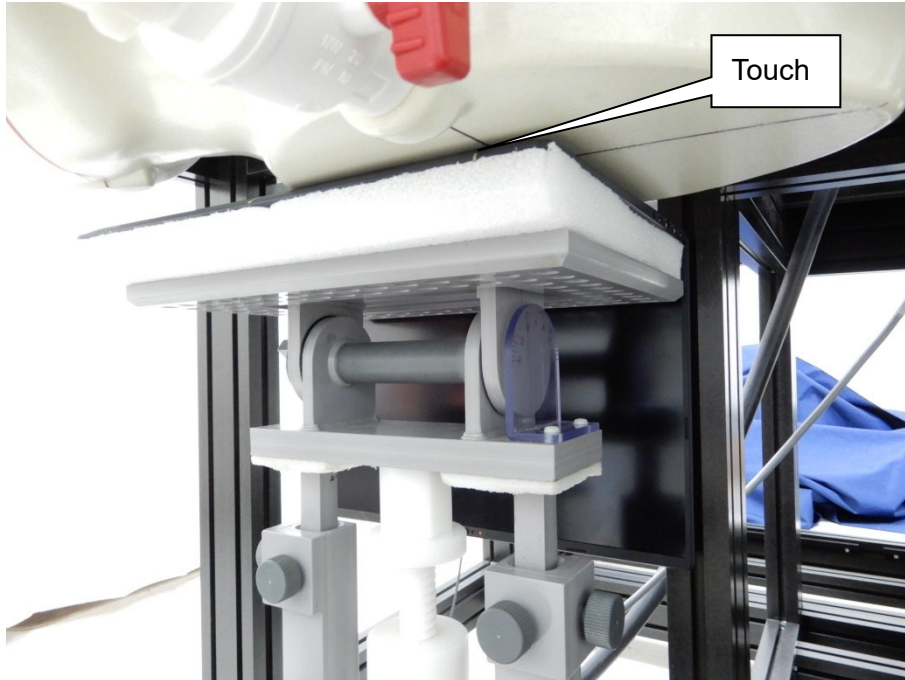
EUT Bottom of laptop_Ant Main
