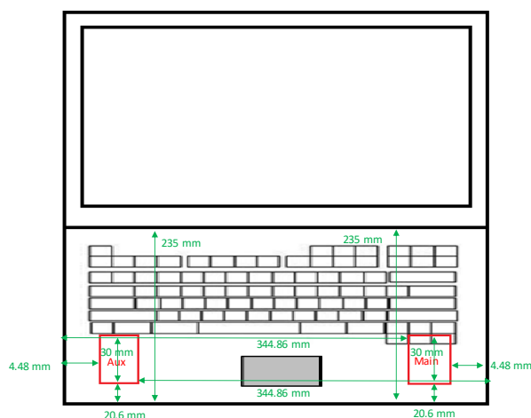
Photograph 5. Antenna position of EUT (Laptop mode)
