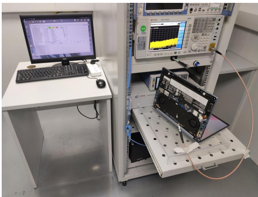
Conducted Test-WIFI
