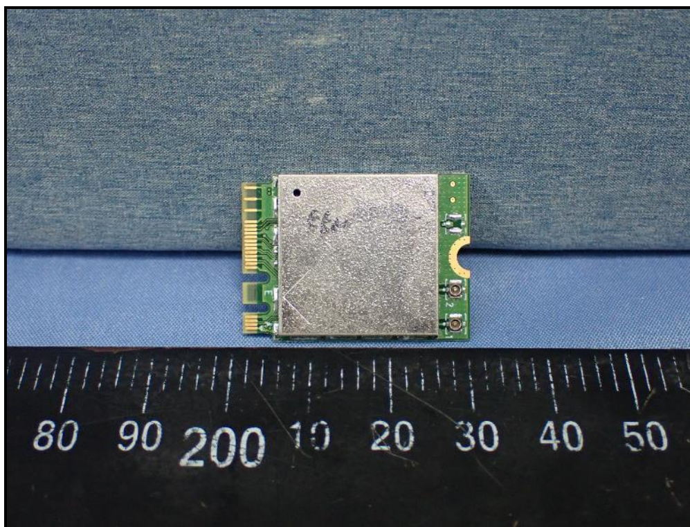
PCIe + USB (Dual antenna port)
