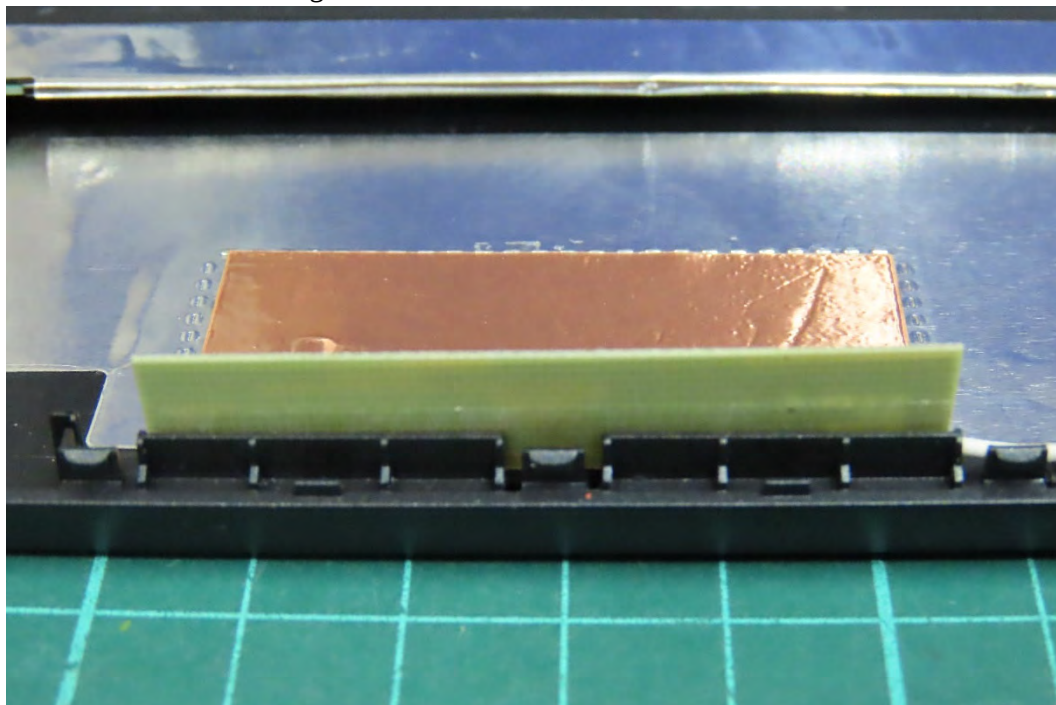
(42) EUT Photo - Antenna: High-Tek Electronics Co., Ltd.
