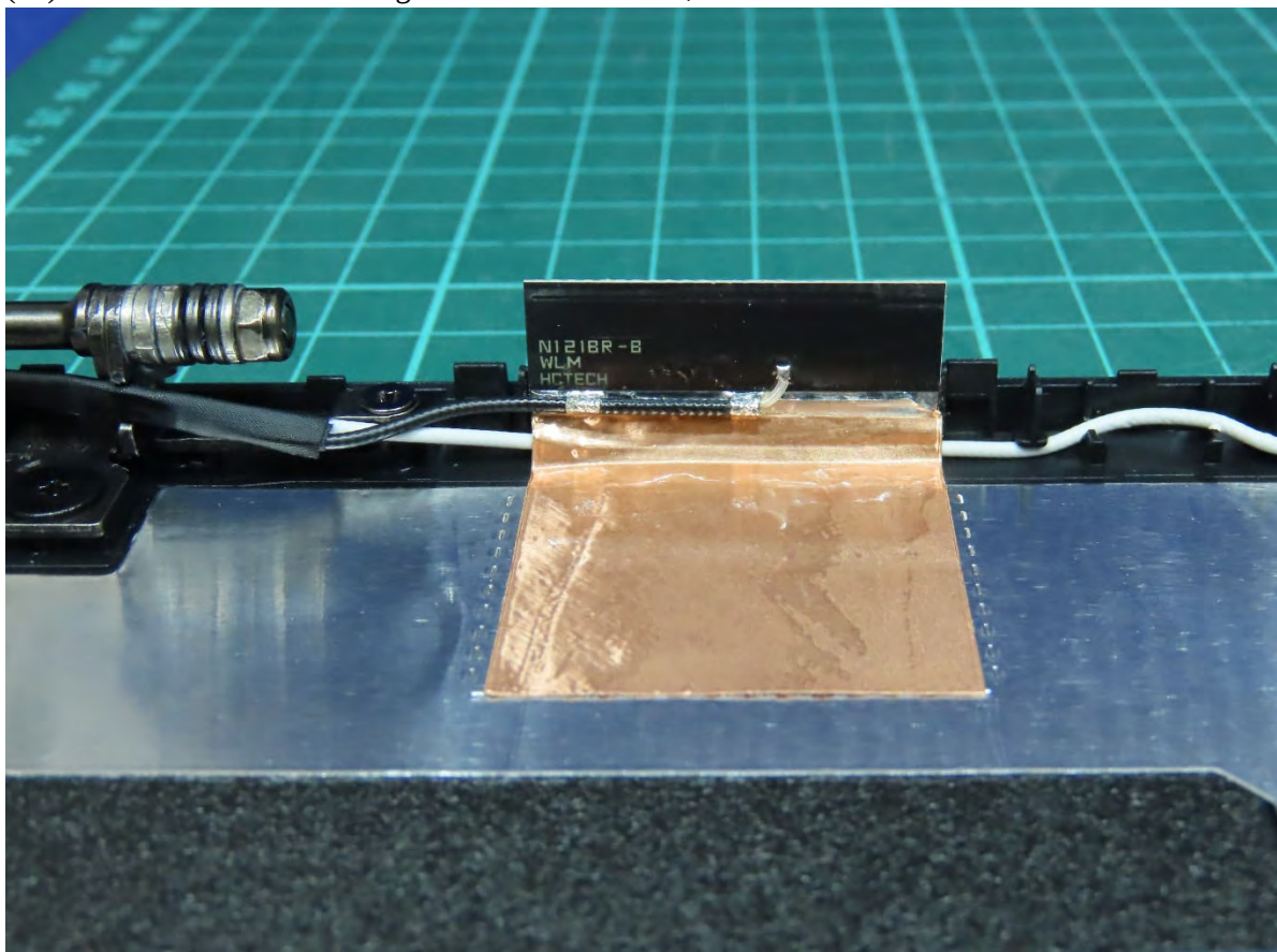
(39) EUT Photo - Antenna: High-Tek Electronics Co., Ltd.
