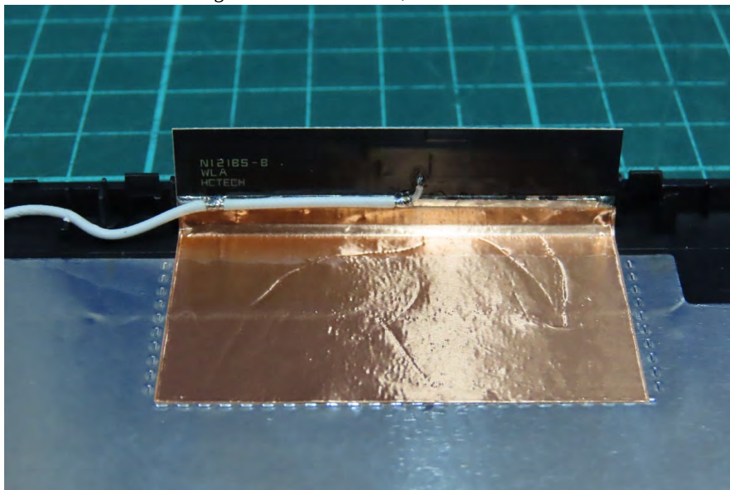
(41) EUT Photo - Antenna: High-Tek Electronics Co., Ltd.
