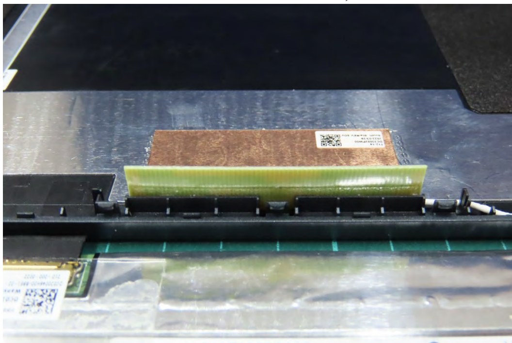
(38) EUT Photo - Antenna: SOUTHSTAR TECHNOLOGY CO.,LTD
