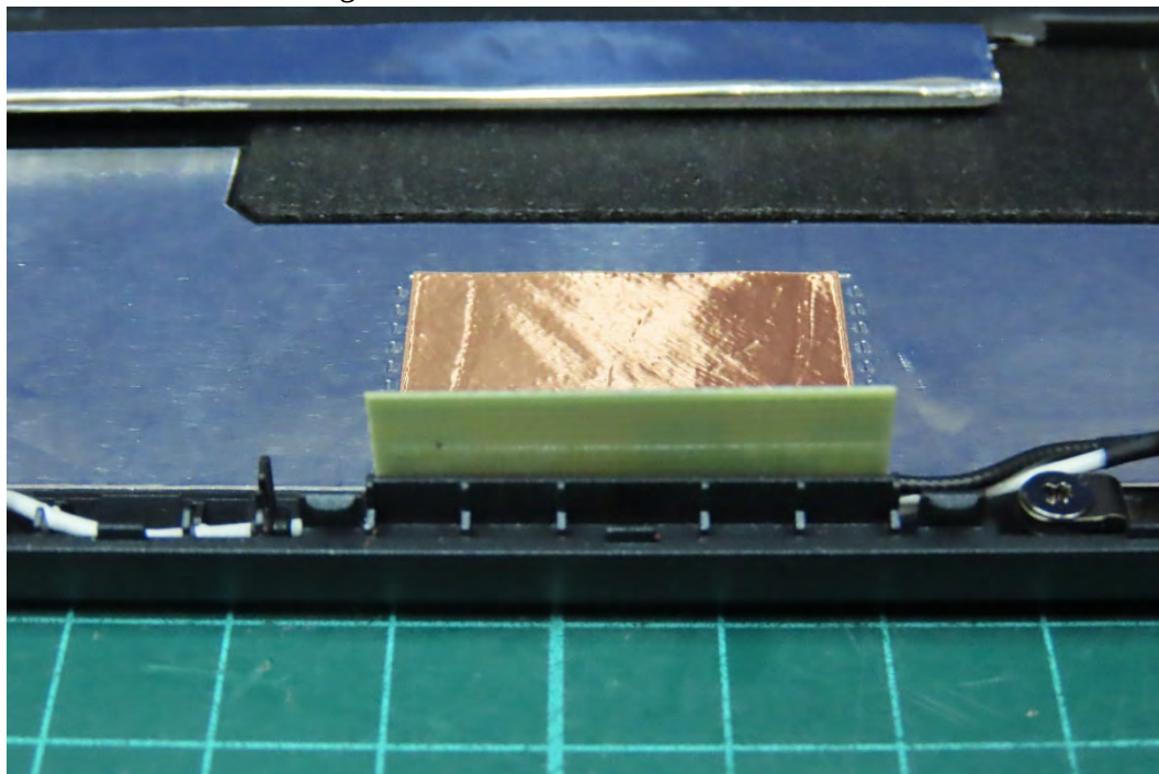
(40) EUT Photo - Antenna: High-Tek Electronics Co., Ltd.
