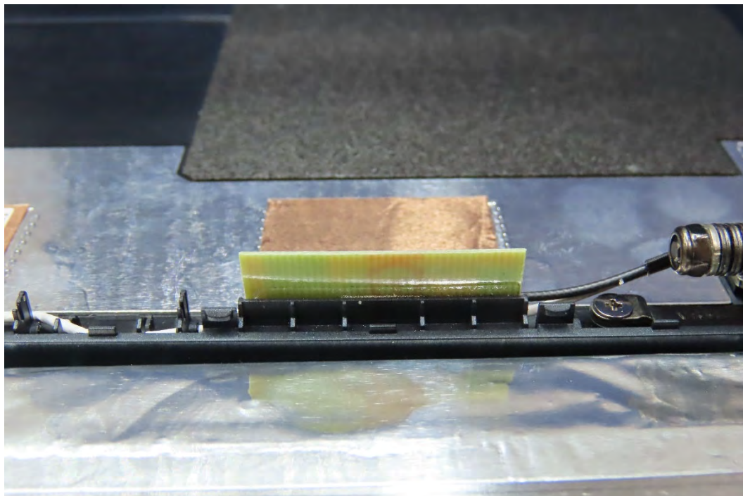
(36) EUT Photo - Antenna: SOUTHSTAR TECHNOLOGY CO.,LTD
