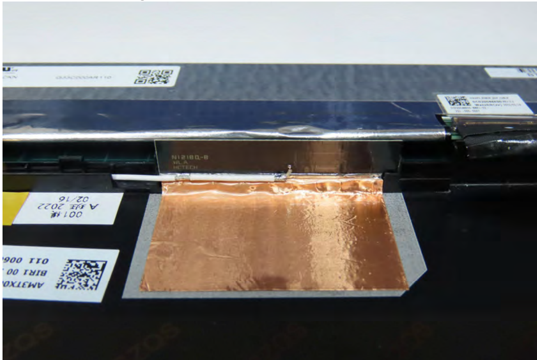
(29) EUT Photo - Antenna: High-Tek Electronics Co., Ltd.
