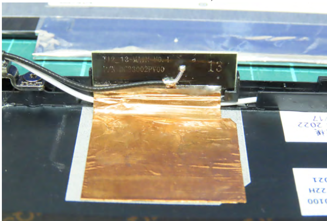
(27) EUT Photo - Antenna: SOUTHSTAR TECHNOLOGY CO.,LTD
