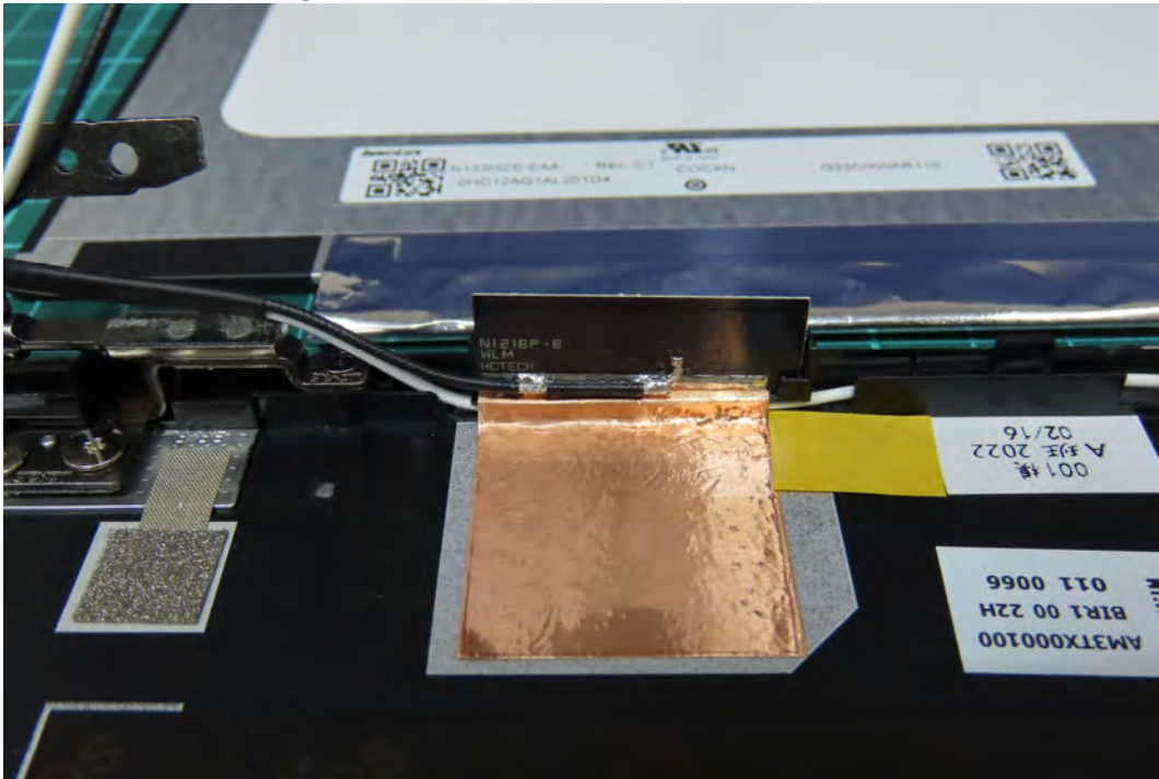
(31) EUT Photo - Antenna: High-Tek Electronics Co., Ltd.
