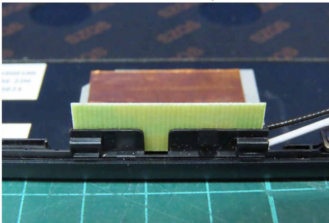
(28) EUT Photo - Antenna: SOUTHSTAR TECHNOLOGY CO.,LTD
