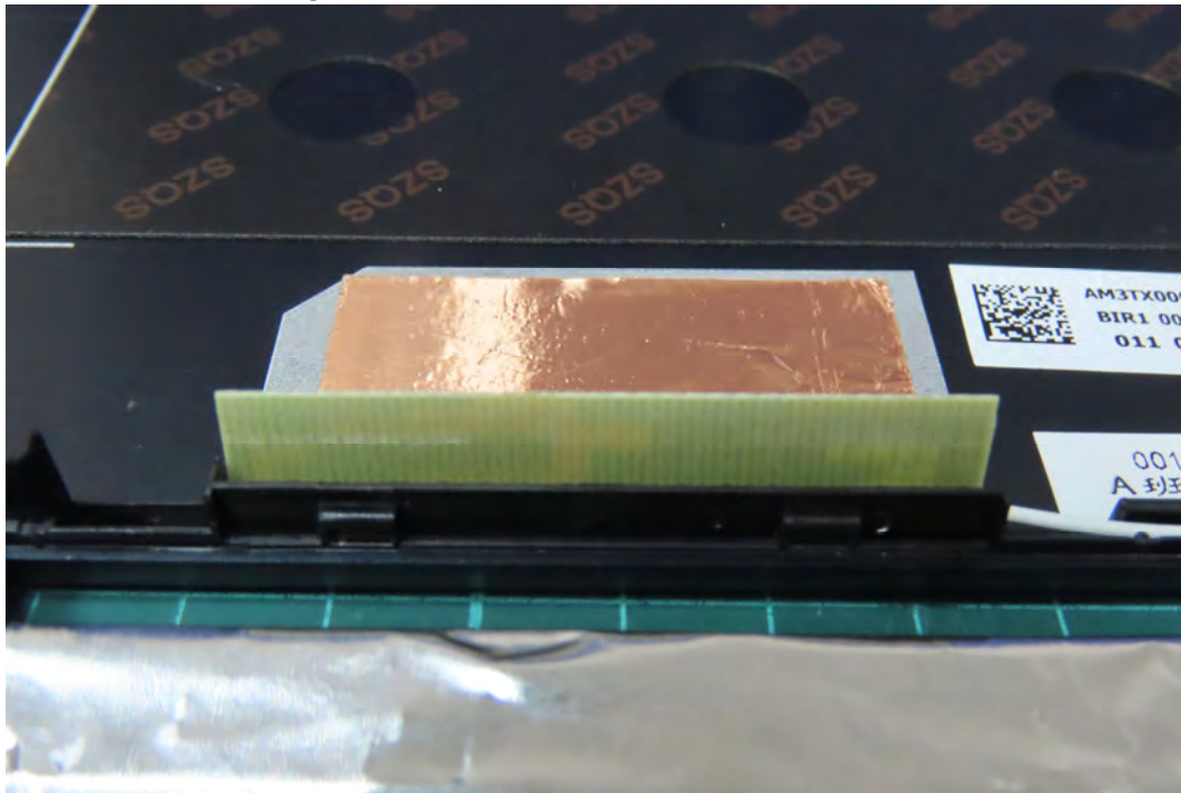
(30) EUT Photo - Antenna: High-Tek Electronics Co., Ltd.
