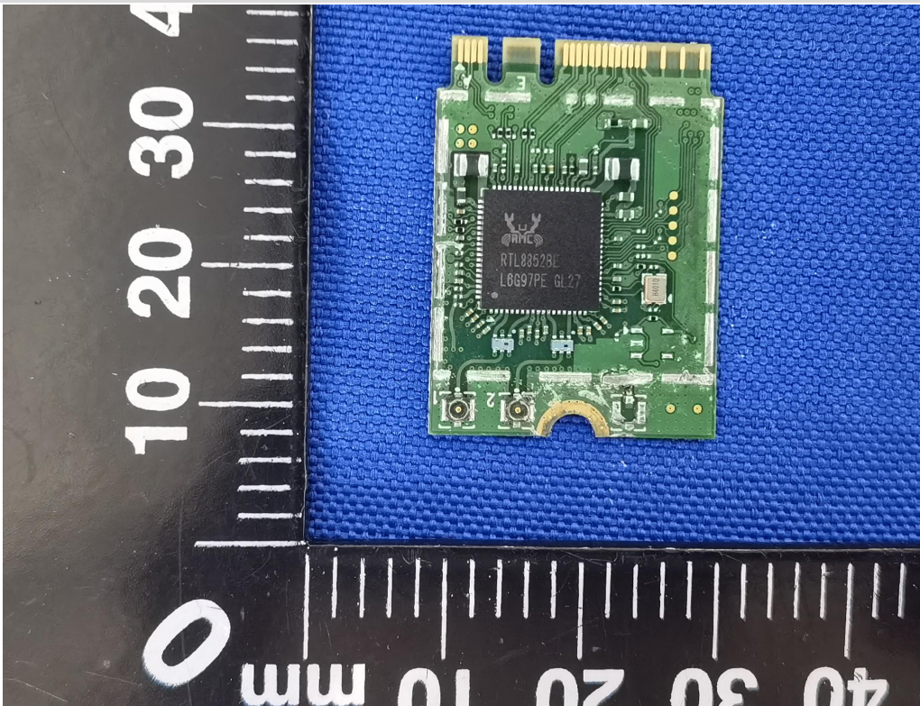
RF MODULE TOP VIEW(WITHOUT THE SHIELDING)_RTL8852BE
