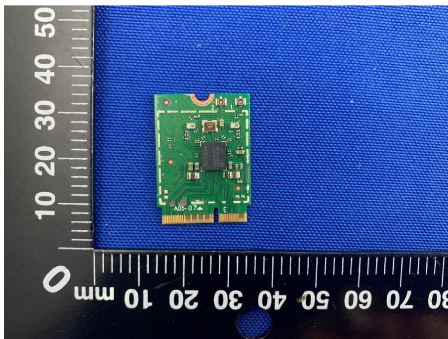
RF MODULE TOP VIEW (WITHOUT SHIELDING)_RTL8852BE
