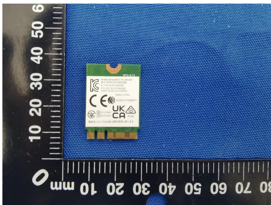
RF MODULE REAR VIEW _RTL8852BE
