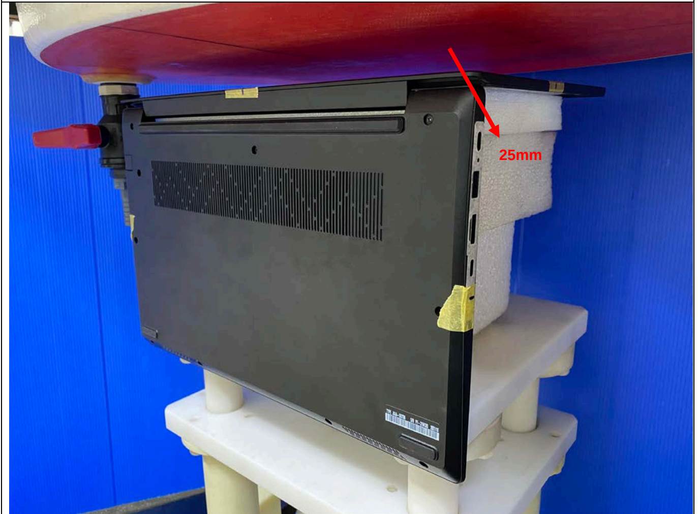
Photo 3: LCD Back_25mm
