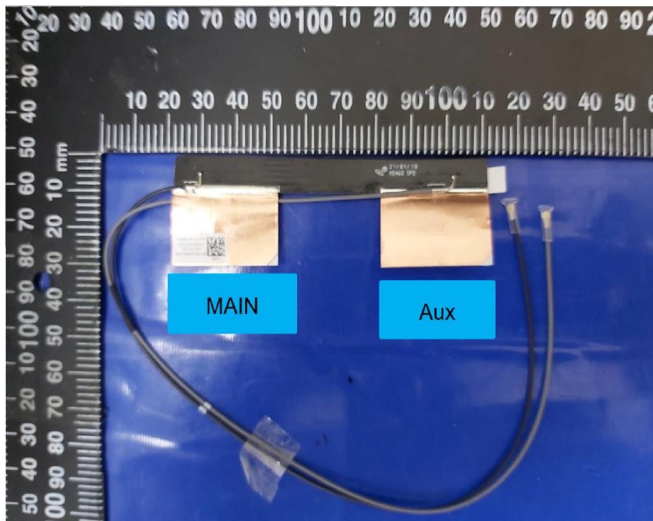
Speedwire Antenna
