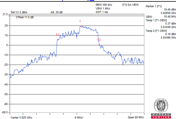
802.11ax (RU106)_Chain 1 / CH165
