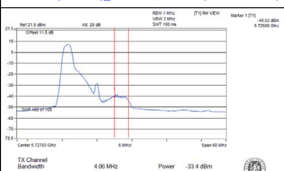
802.11ax (RU26/0)_Chain 1 / CH144 (U-NII-3 Band)
