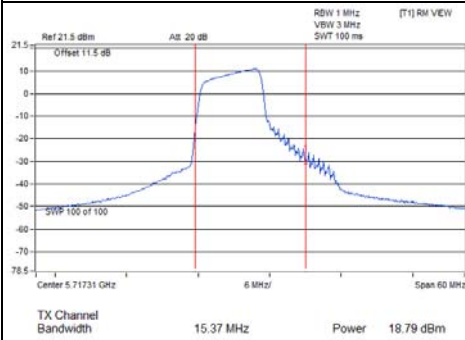
802.11ax (RU106/53) / CH144 (U-NII-2C Band)
