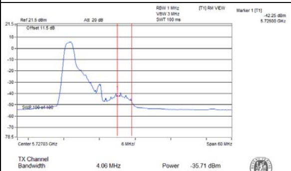
802.11ax (RU26/0)_Chain 0 / CH144 (U-NII-3 Band)
