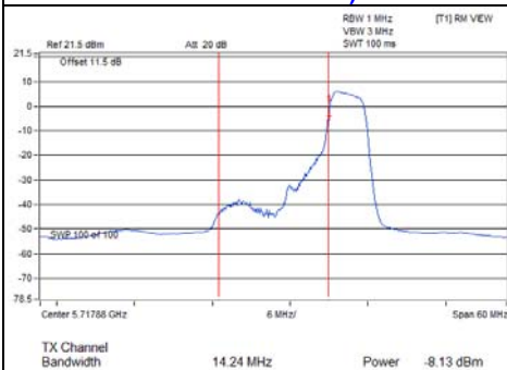
802.11ax (RU52/40)_Chain 1 / CH144 (U-NII-2C Band)
