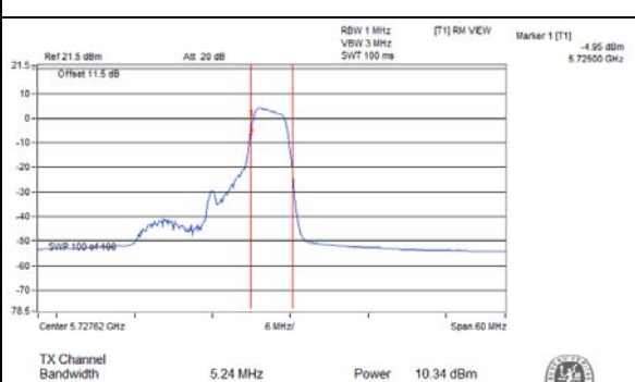
802.11ax (RU52/40)_Chain 0 / CH144 (U-NII-3 Band)
