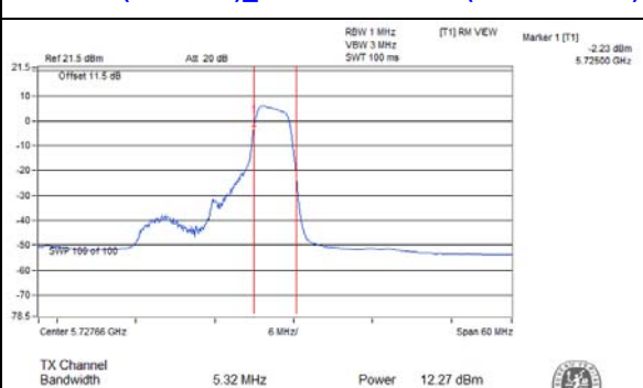
802.11ax (RU52/40)_Chain 1 / CH144 (U-NII-3 Band)
