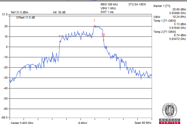
802.11ax (RU52)_Chain 0 / CH165
