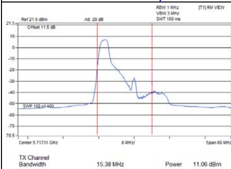
802.11ax (RU26/0)_Chain 1 / CH144 (U-NII-2C Band)
