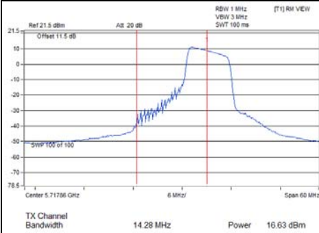
802.11ax (RU106/54) / CH144 (U-NII-2C Band)
