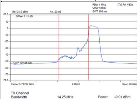
802.11ax (RU52/40)_Chain 0 / CH144 (U-NII-2C Band)
