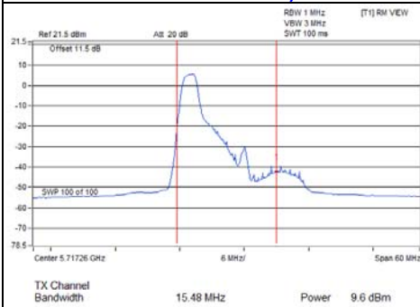
802.11ax (RU26/0)_Chain 0 / CH144 (U-NII-2C Band)
