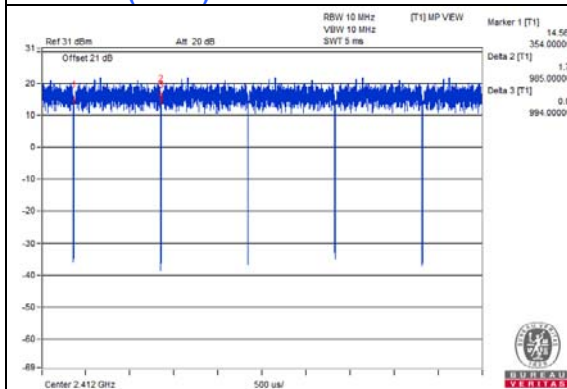
802.11ax (RU26)
