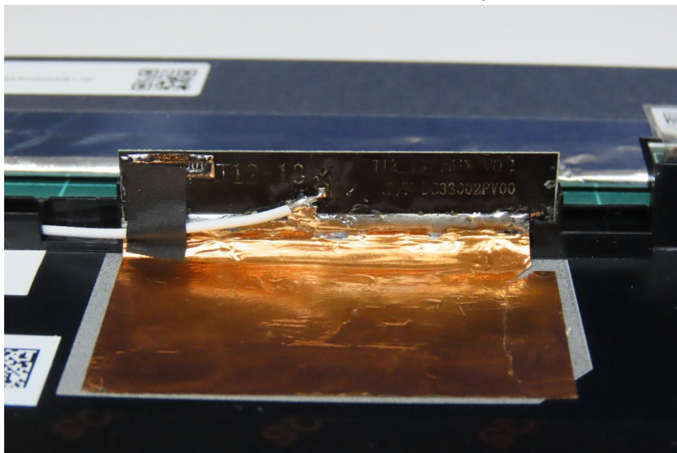
(32) EUT Photo - Antenna: SOUTHSTAR TECHNOLOGY CO.,LTD
