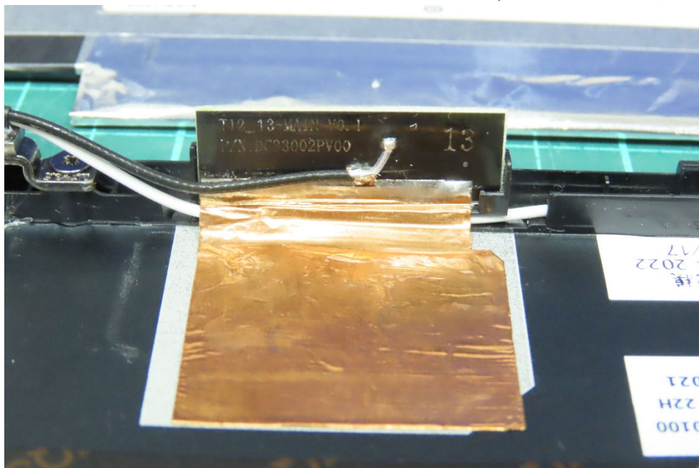
(34) EUT Photo - Antenna: SOUTHSTAR TECHNOLOGY CO.,LTD
