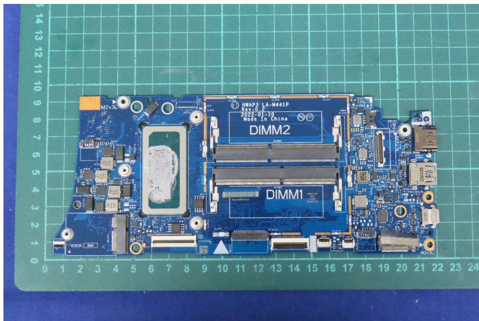
(25) EUT Photo
