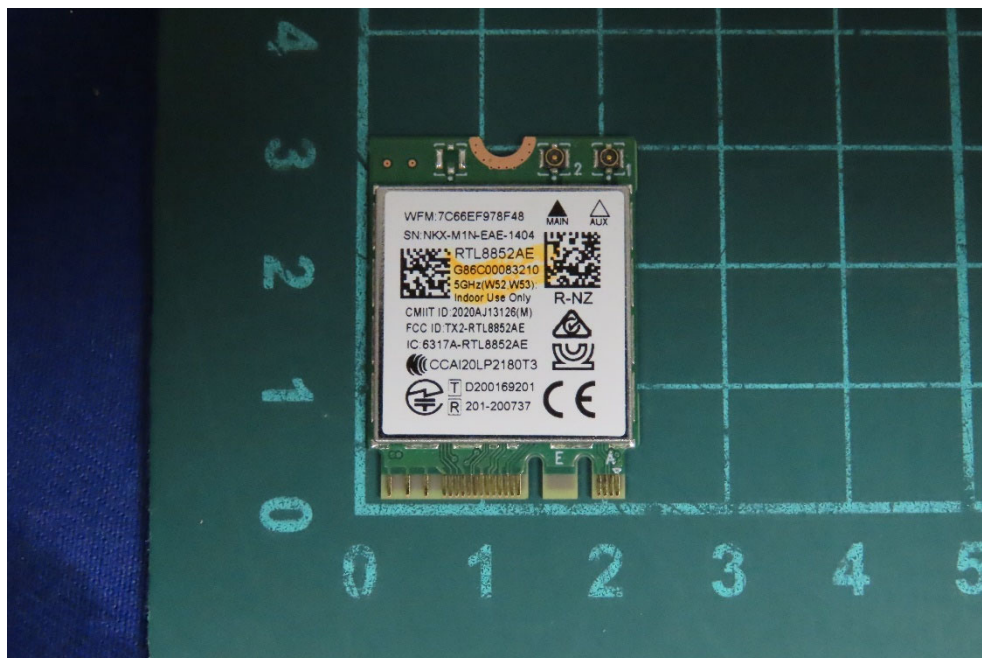
(23) EUT Photo
