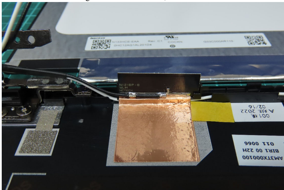
(38) EUT Photo - Antenna: High-Tek Electronics Co., Ltd.
