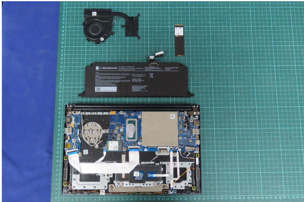
(11) EUT Photo
