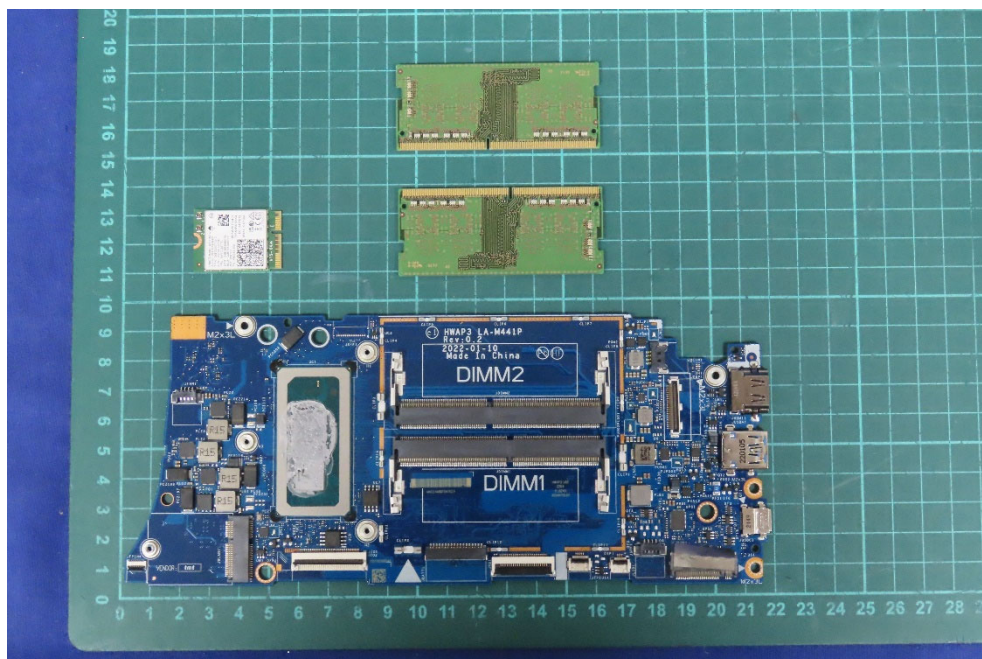
(22) EUT Photo
