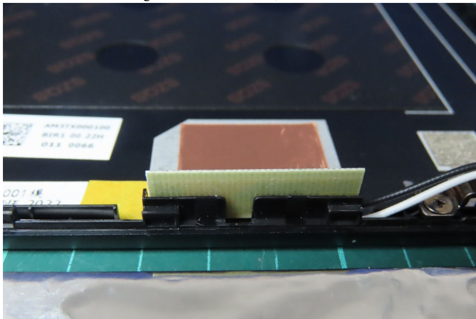
(39) EUT Photo - Antenna: High-Tek Electronics Co., Ltd.
