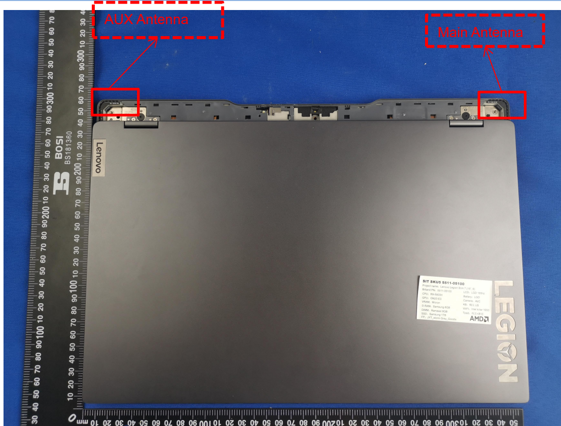
Antenna location
