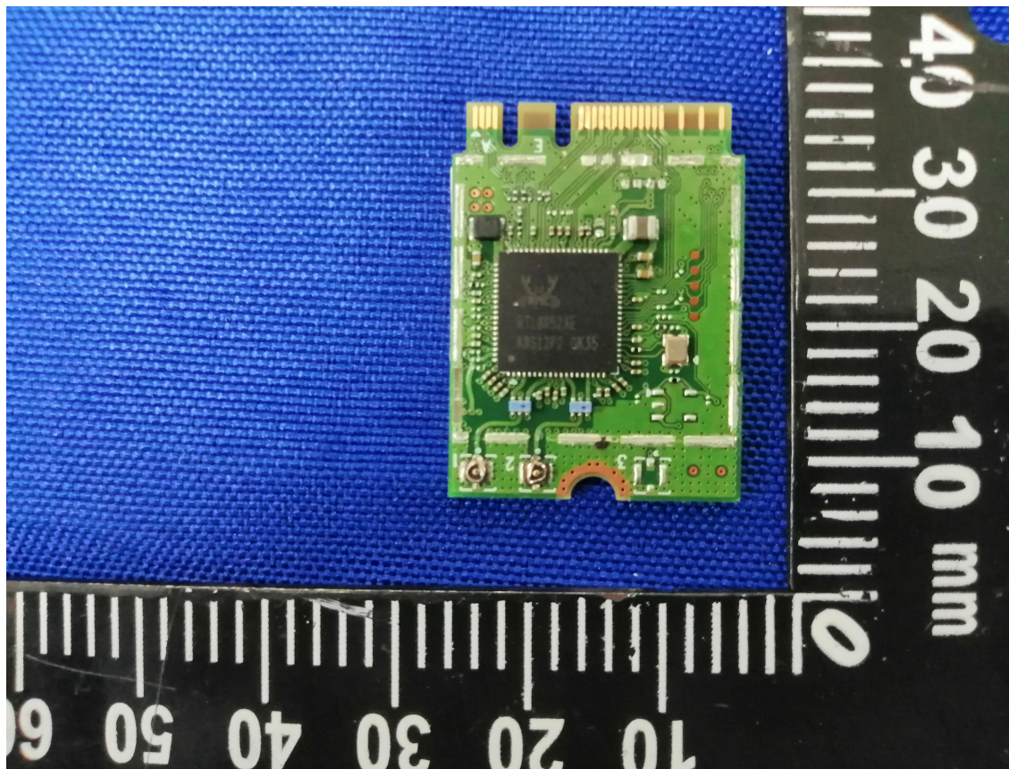
RF MODULE TOP VIE(WITHOUT THE SHIELDING)_RTL8852AE
