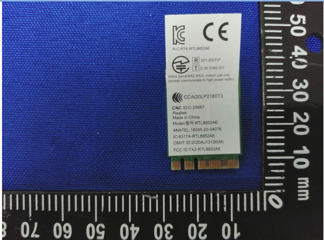
RF MODULE BACK VIEW_RTL8852AE
