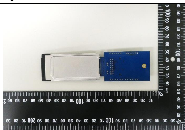
USB Jig
