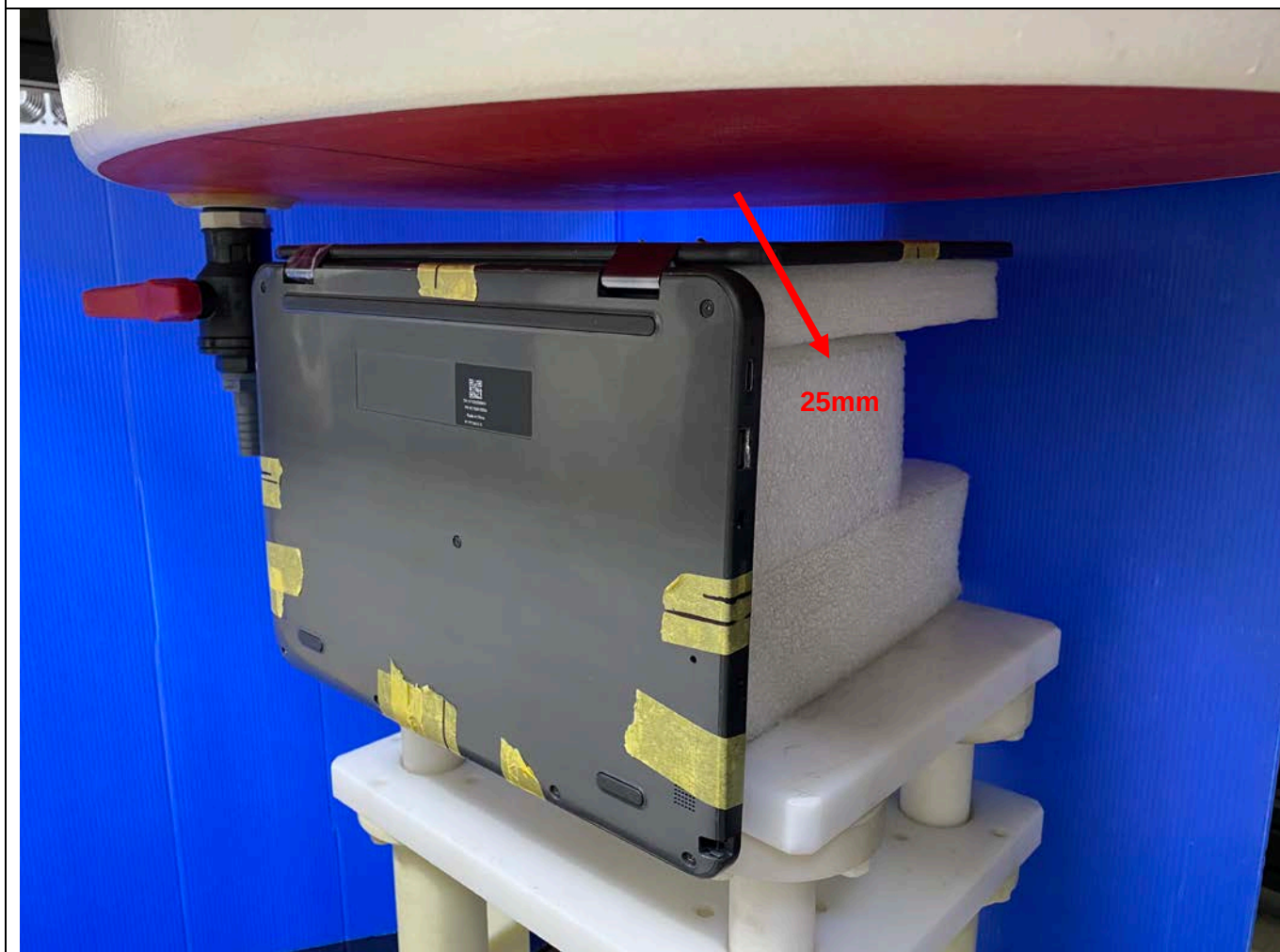
Photo 3: LCD Back_25mm
