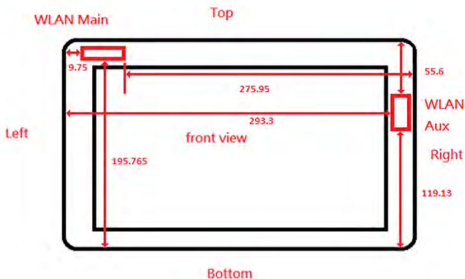
Photograph 15. Antenna location of EUT (tablet mode)
