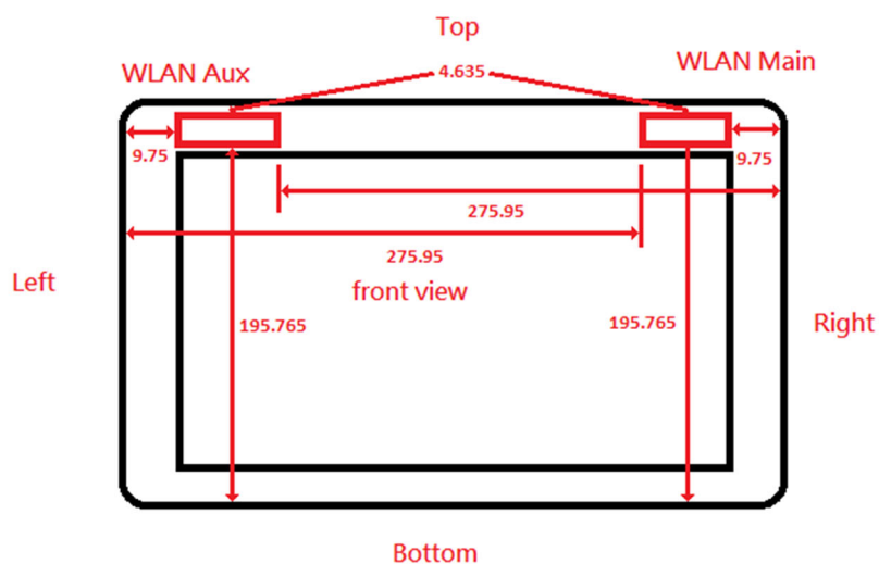
Photograph 13. Antenna location of EUT (tablet mode)
