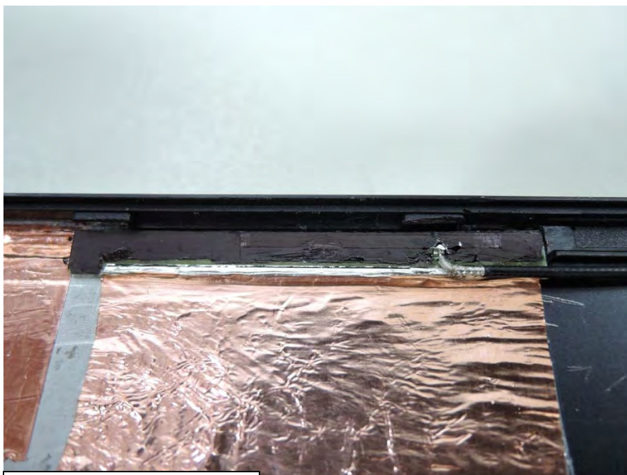
INPAQ Main Antenna Part No.: WA-P-LBLB-04-081
