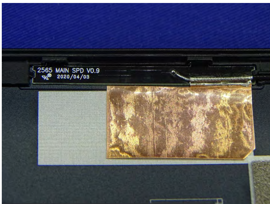
SPEED Main Antenna Part No.: F-0G-XZ-0231-000-00
