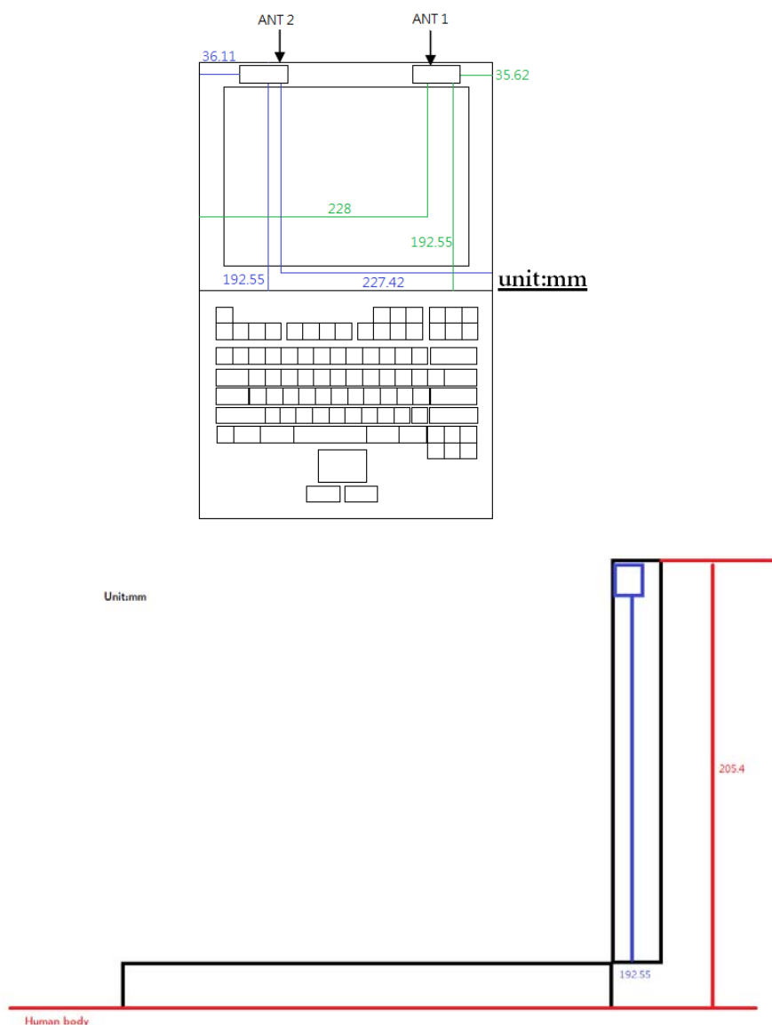
Fig.6 Antenna position of EUT
