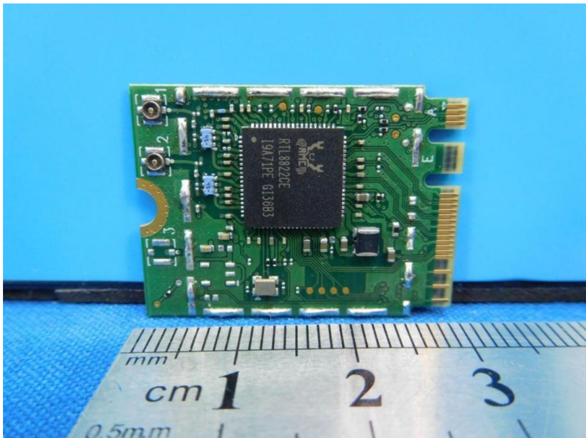
RF MODULE TOP VIEW (WITHOUT SHIELDING)
