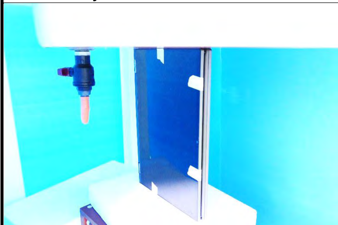
Body - Left Side of EUT at 0 mm
