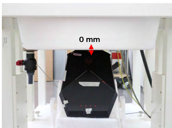
Fig.7 EUT position(2-2) to flat phantom
