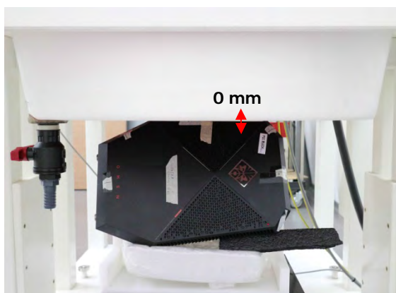
Fig.10 EUT position(2-5) to flat phantom
