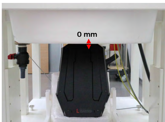
Fig.13 EUT position(2-8) to flat phantom
