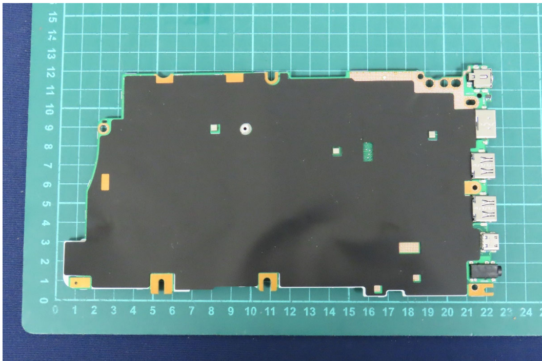
(23) EUT Photo
