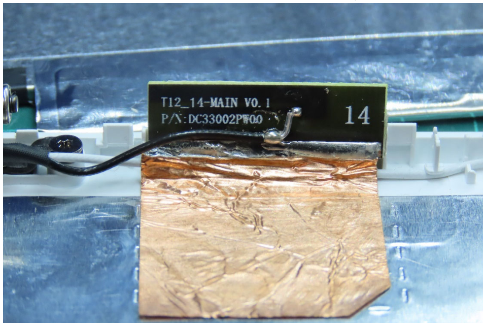
(31) EUT Photo - Antenna: SOUTHSTAR TECHNOLOGY CO.,LTD
