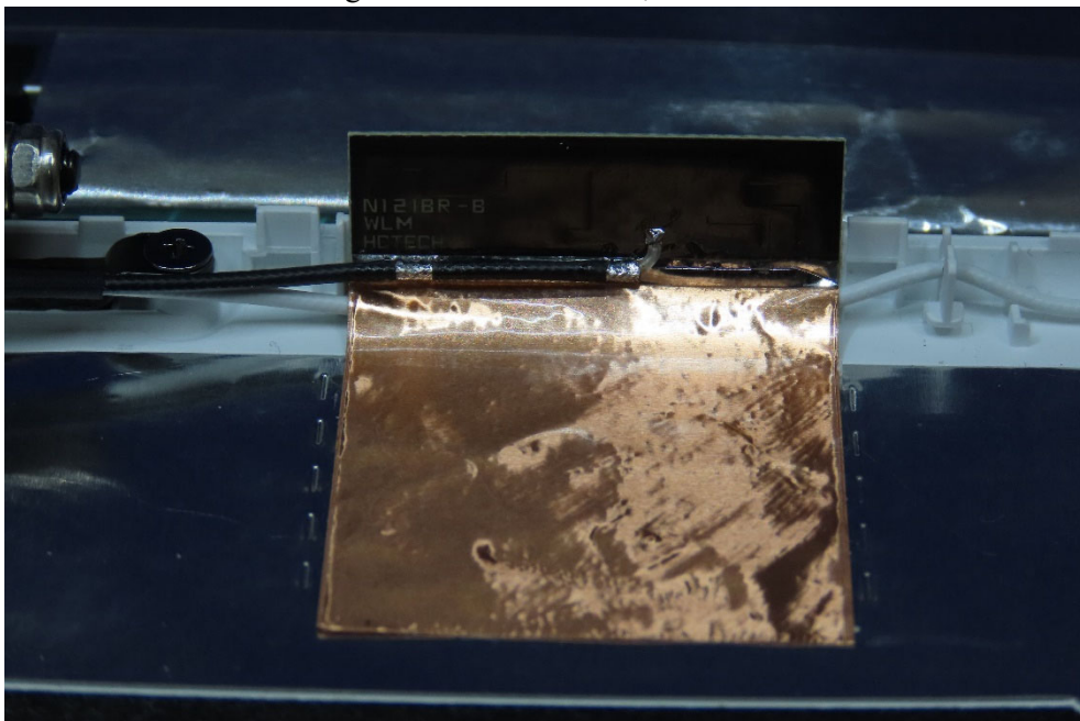
(35) EUT Photo - Antenna: High-Tek Electronics Co., Ltd.
