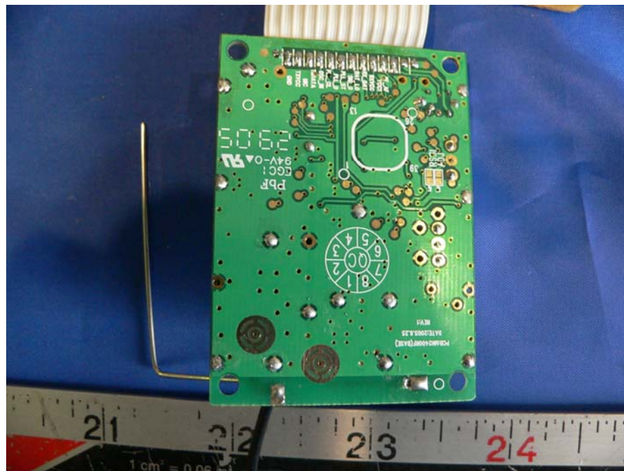
EUT – RF Solder View
