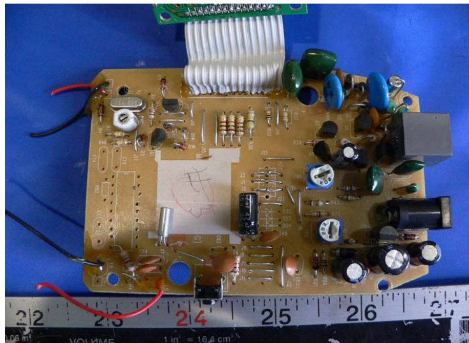
EUT – Component View
