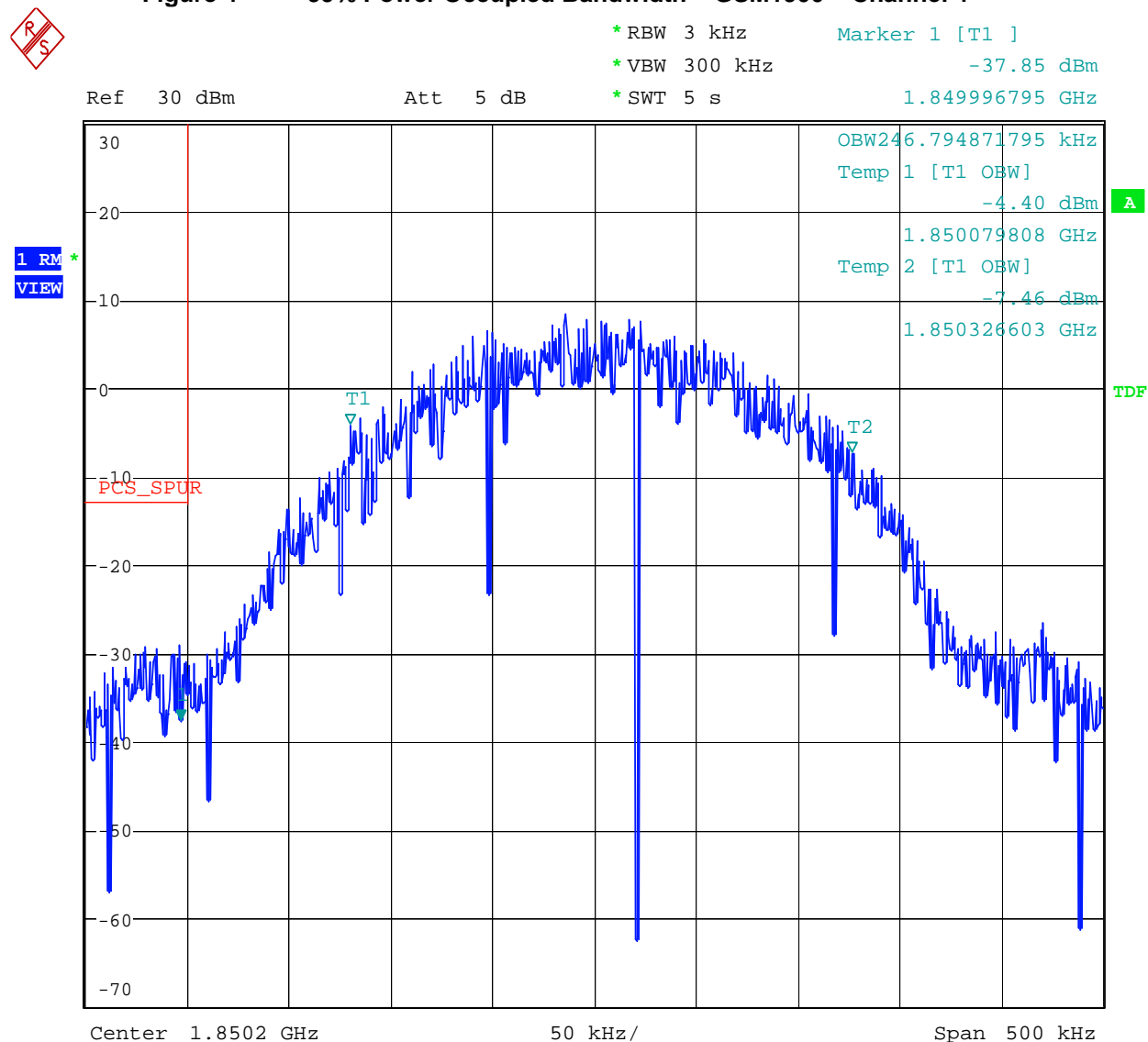
Figure 4 99% Power Occupied Bandwidth – GSM1900 – Channel 4
