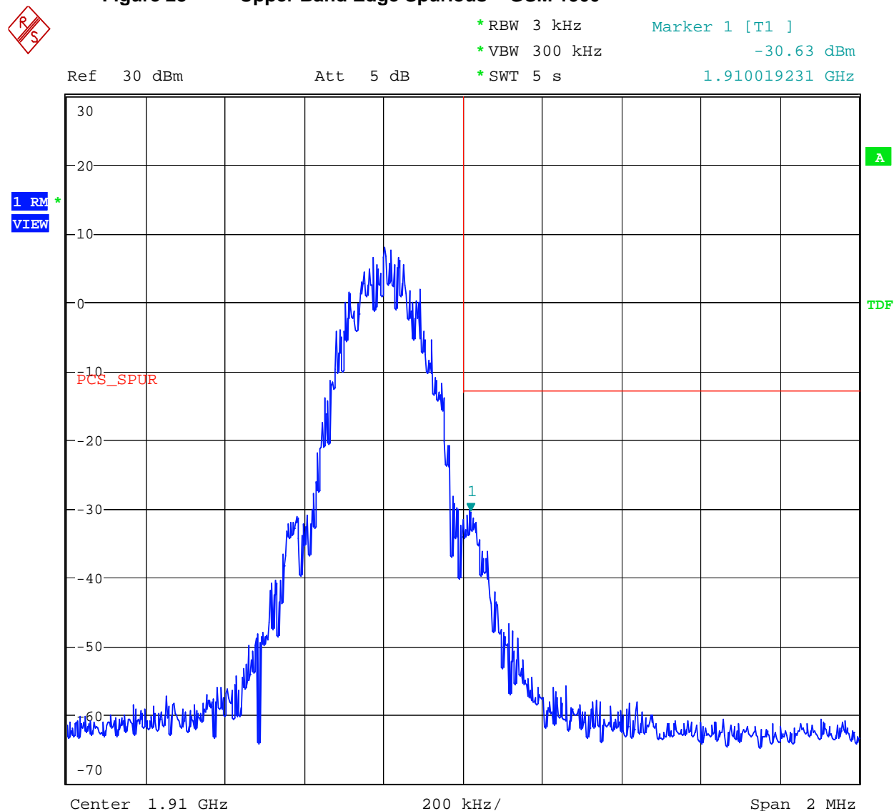
Figure 28 Upper Band Edge Spurious - GSM 1900
