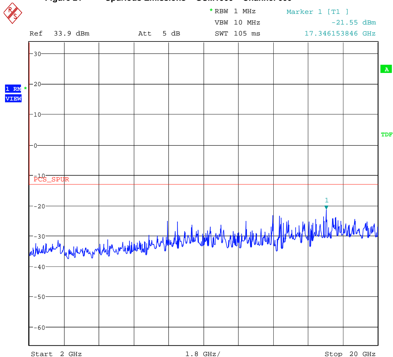
Figure 21 Spurious Emissions - GSM1900 – Channel 600
