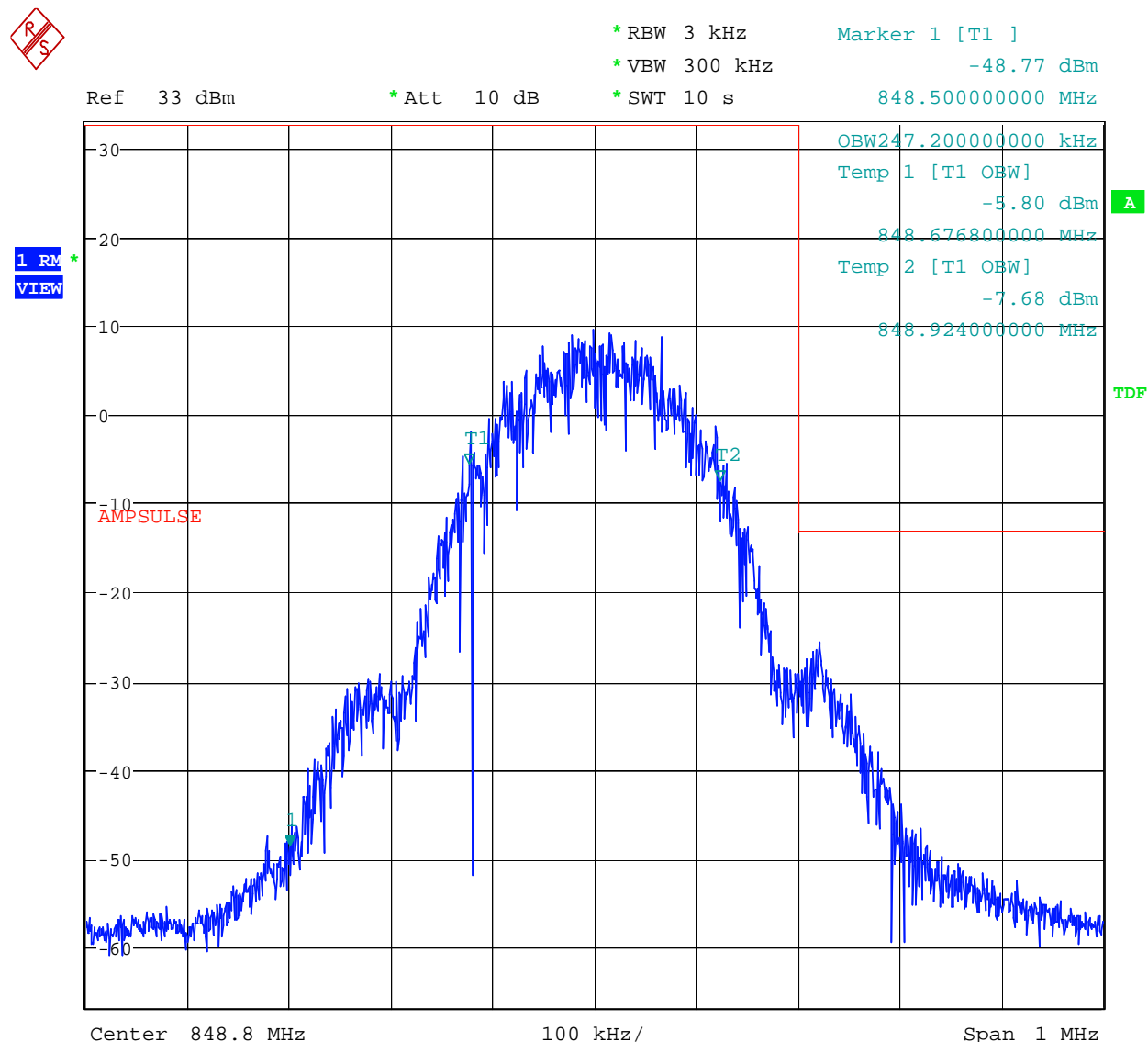
Figure 3 99% Power Occupied Bandwidth – GSM850 – Channel 251
