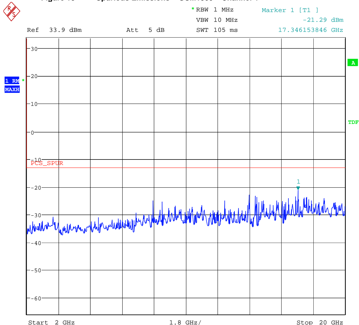
Figure 18 Spurious Emissions - GSM1900 – Channel 4
