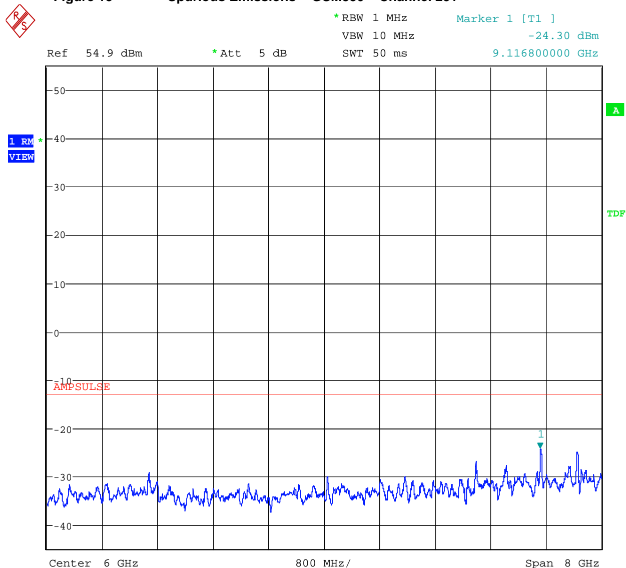
Figure 15 Spurious Emissions - GSM850 – Channel 251
