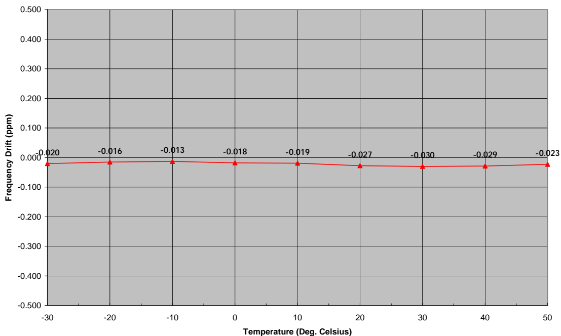
Frequency Drift with Temperature Variation
