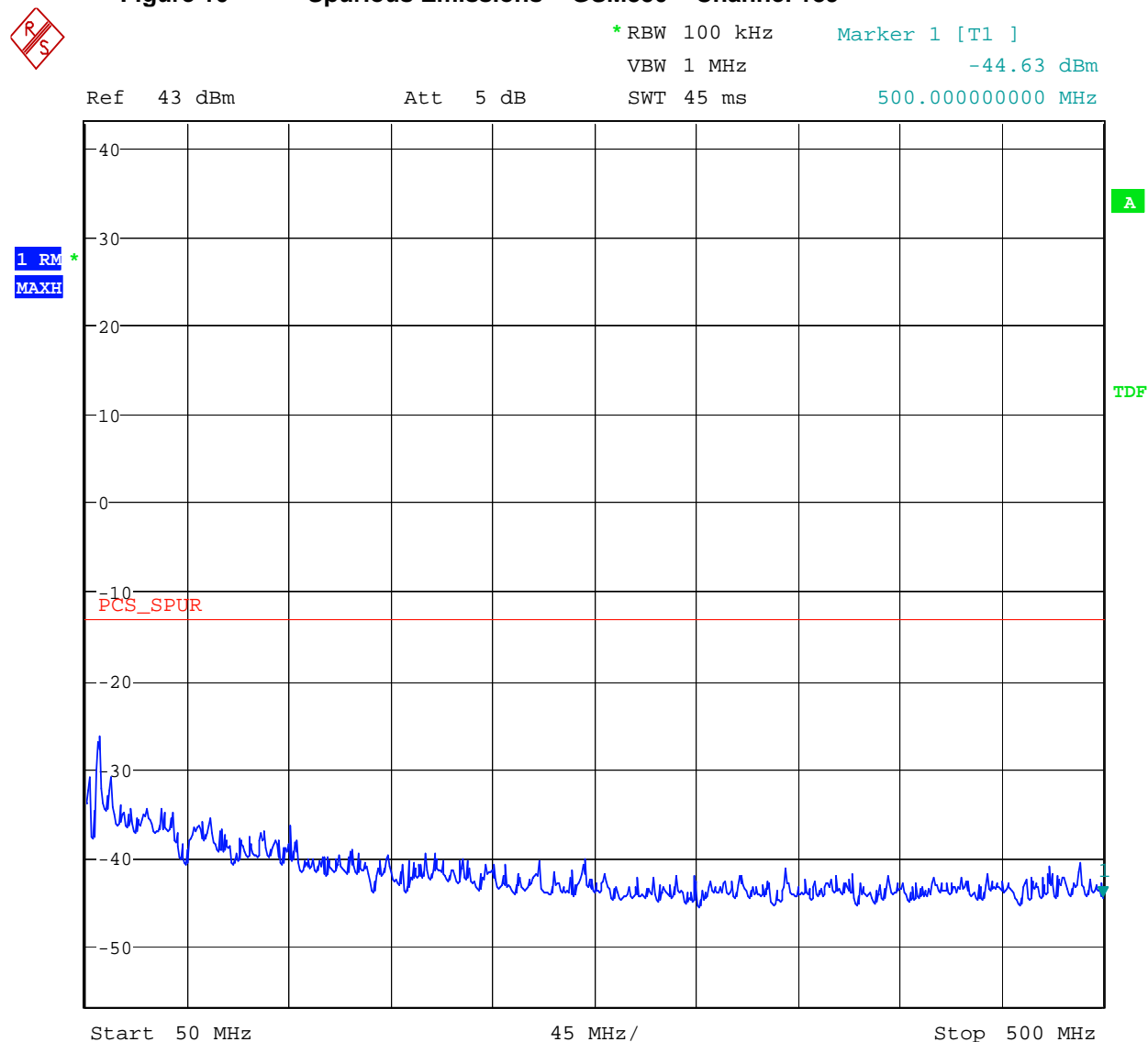
Figure 10 Spurious Emissions - GSM850 – Channel 189
