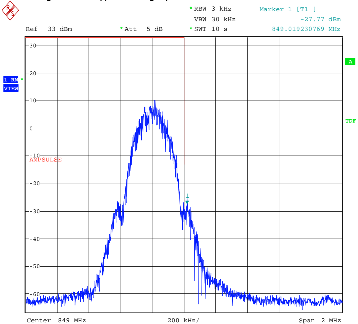
Figure 26 Upper Band Edge Spurious - GSM850
