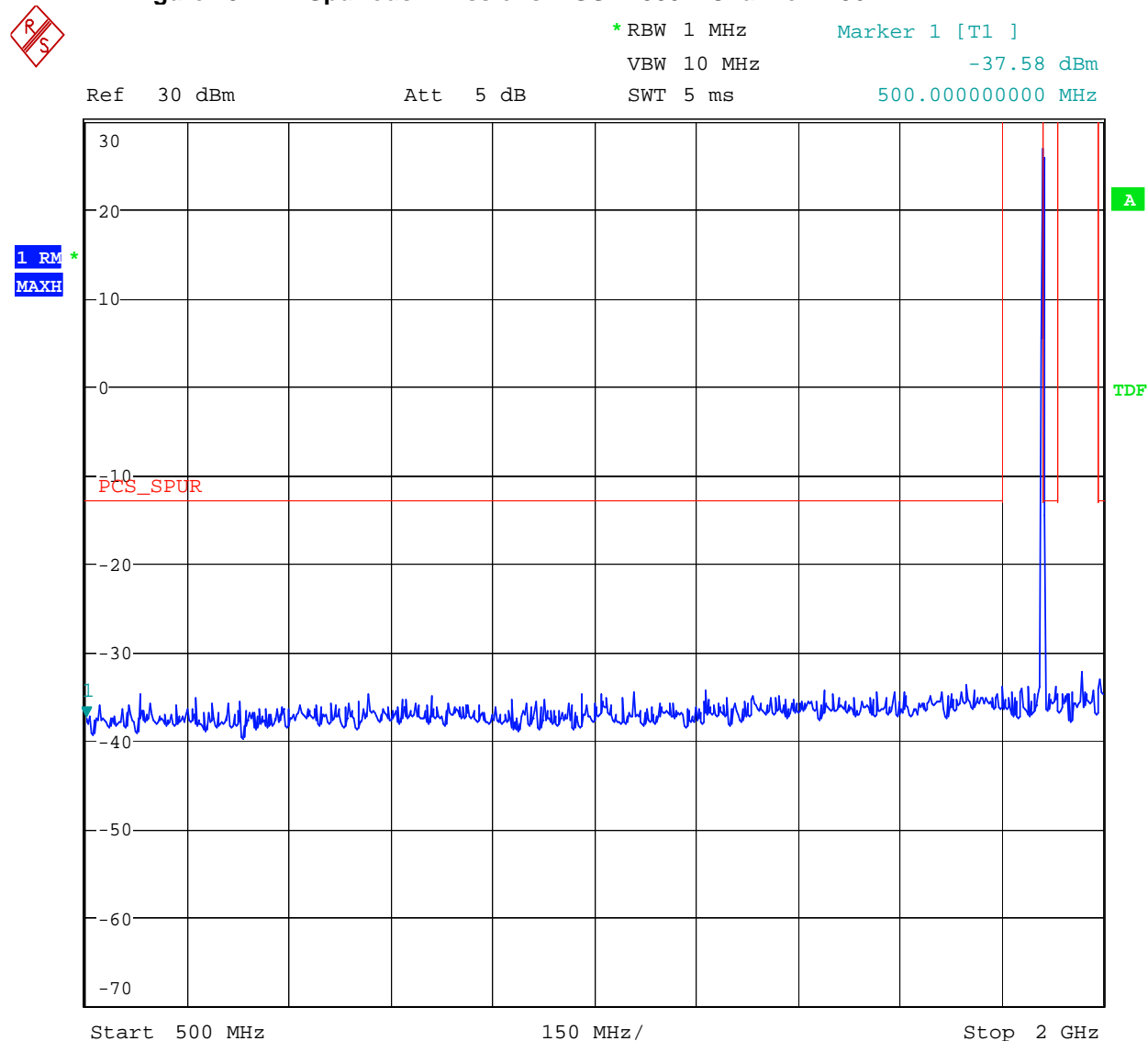
Figure 23 Spurious Emissions - GSM1900 – Channel 1196
