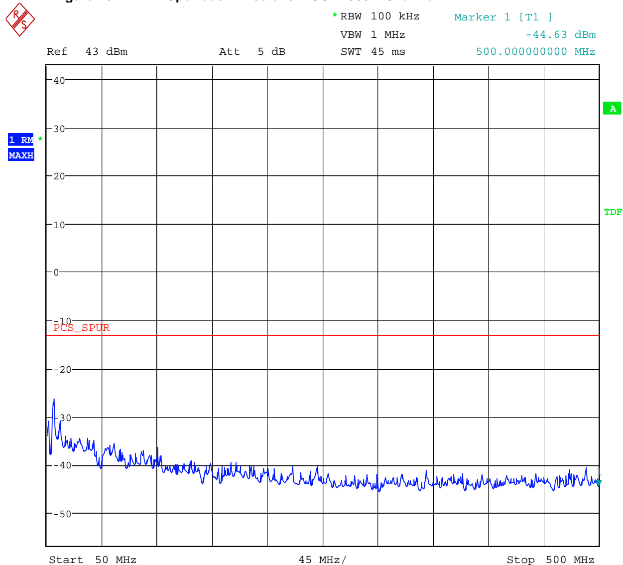
Figure 16 Spurious Emissions - GSM1900 – Channel 4
