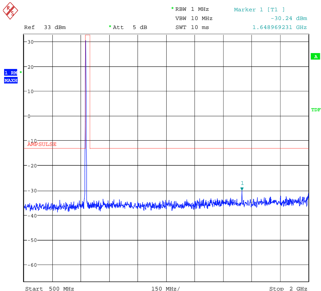
Figure 8 Spurious Emissions - GSM850 – Channel 128
