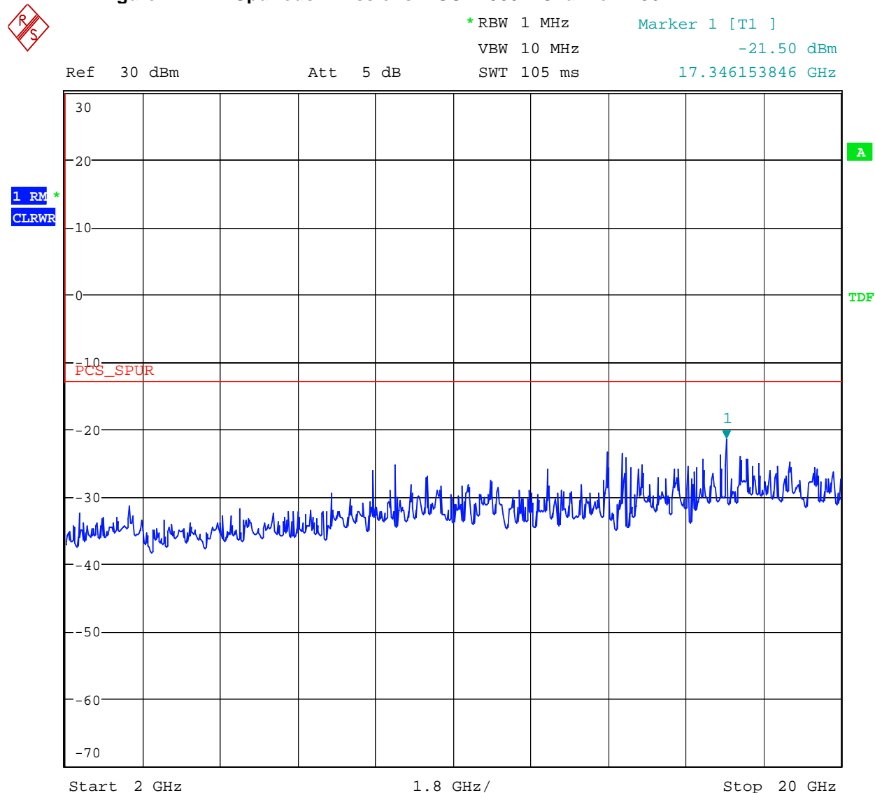
Figure 24 Spurious Emissions - GSM1900 – Channel 1196
