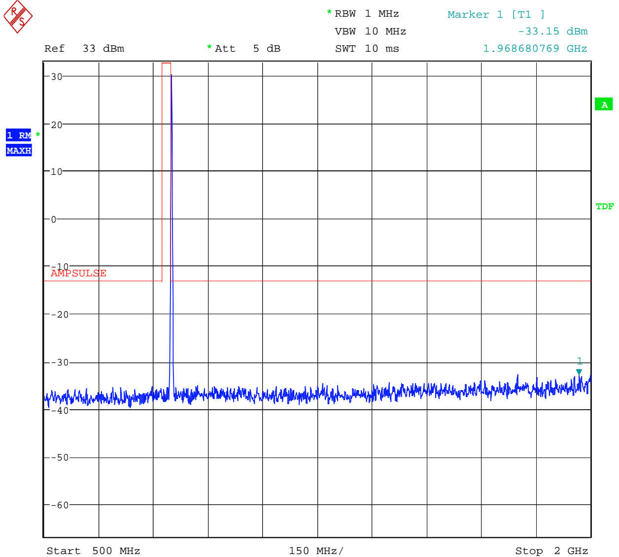
Figure 14 Spurious Emissions - GSM850 – Channel 251
