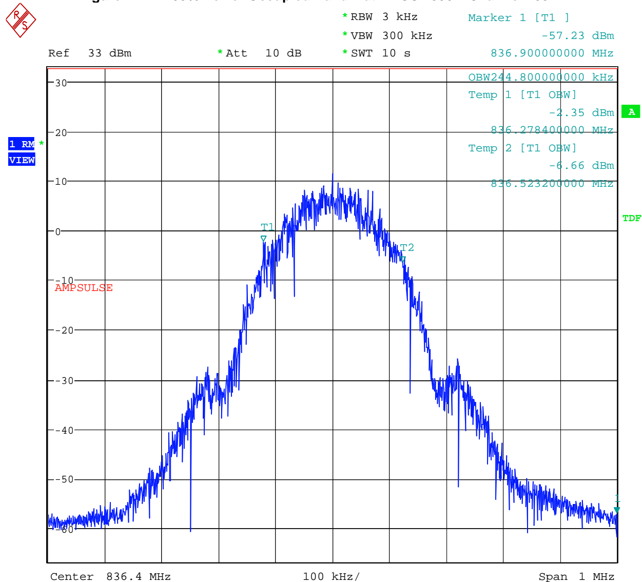
Figure 2 99% Power Occupied Bandwidth – GSM850 – Channel 189
