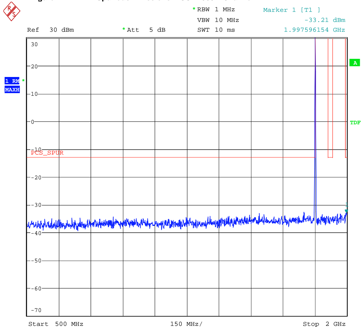
Figure 17 Spurious Emissions - GSM1900 – Channel 4
