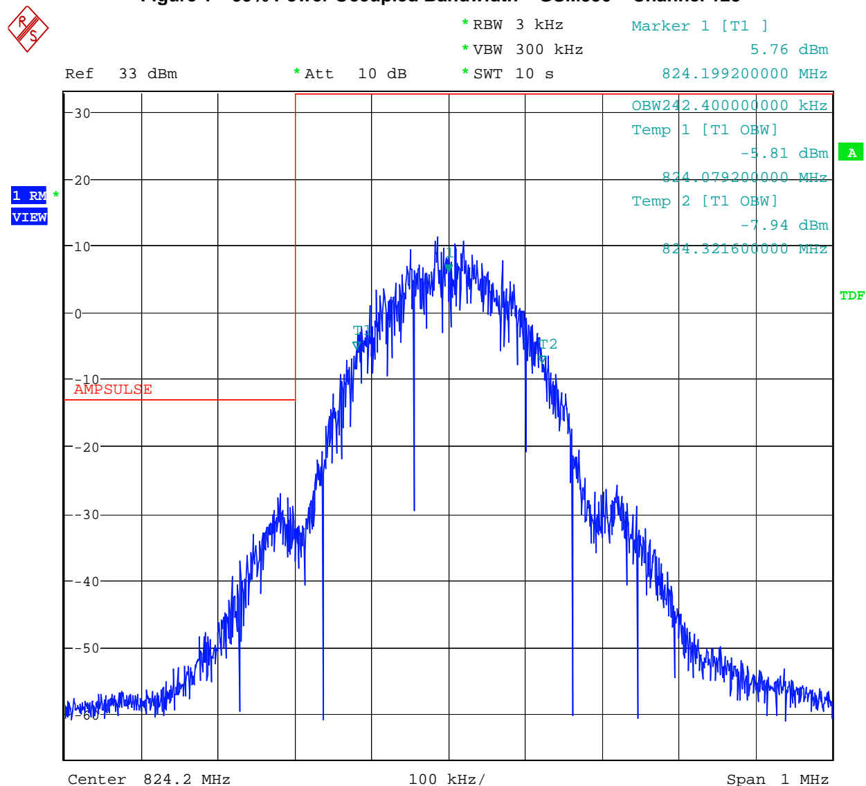
Figure 1 99% Power Occupied Bandwidth – GSM850 – Channel 128
