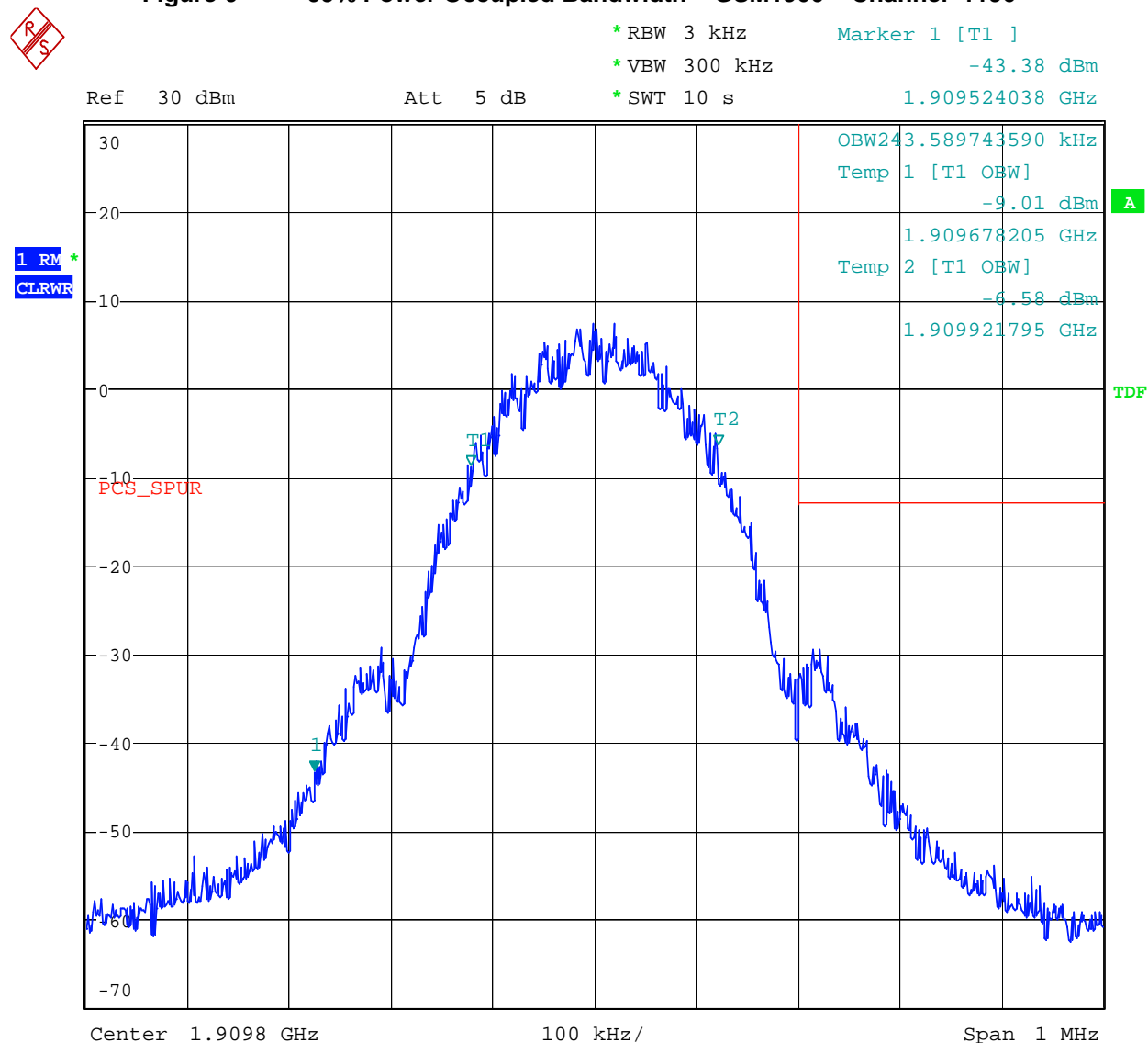
Figure 6 99% Power Occupied Bandwidth – GSM1900 – Channel 1196
