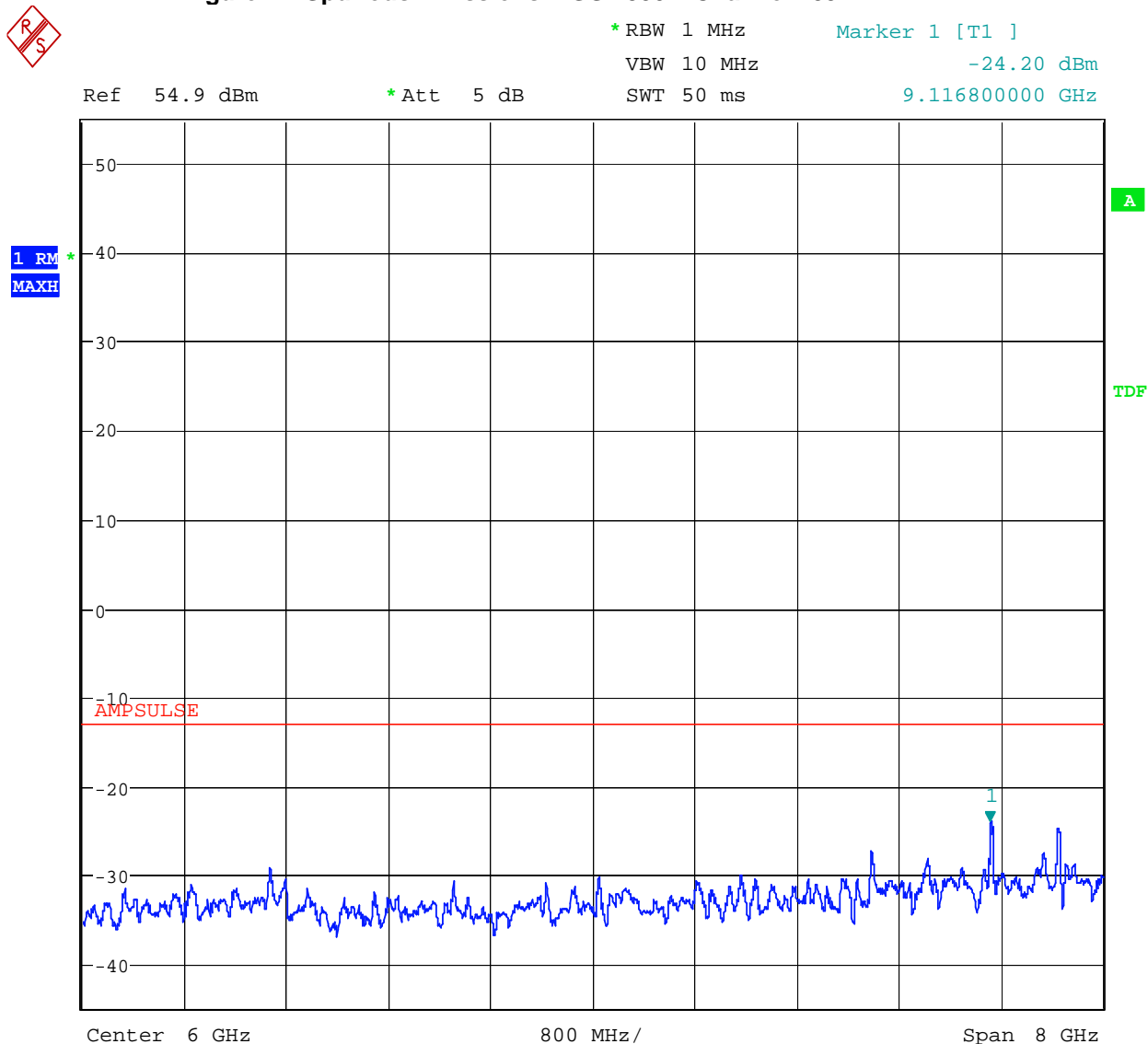
Figure 12 Spurious Emissions - GSM850 – Channel 189
