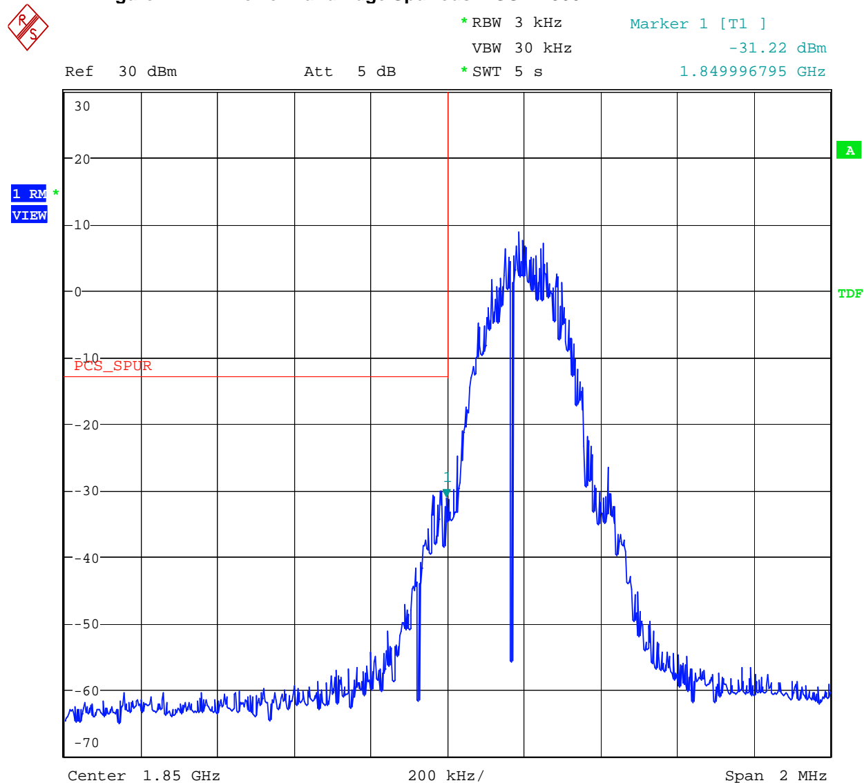
Figure 27 Lower Band Edge Spurious - GSM 1900
