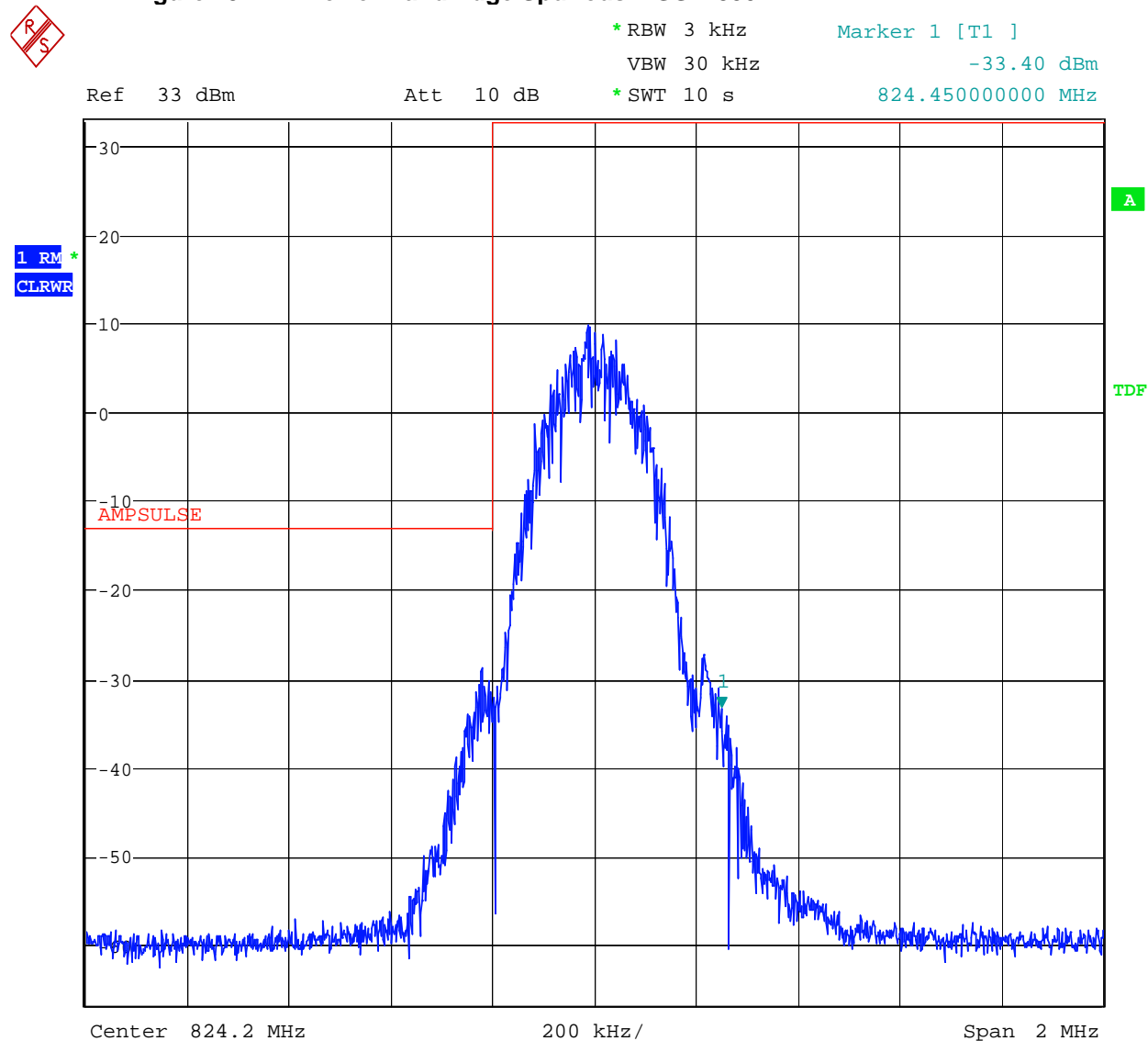
Figure 25 Lower Band Edge Spurious – GSM 850
