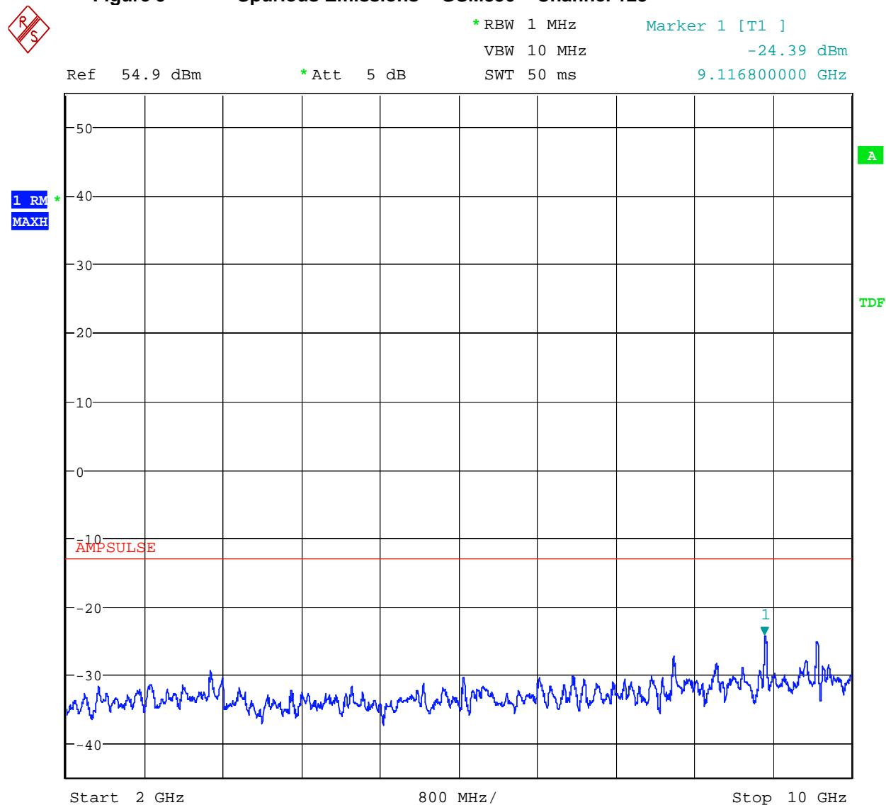
Figure 9 Spurious Emissions - GSM850 – Channel 128
