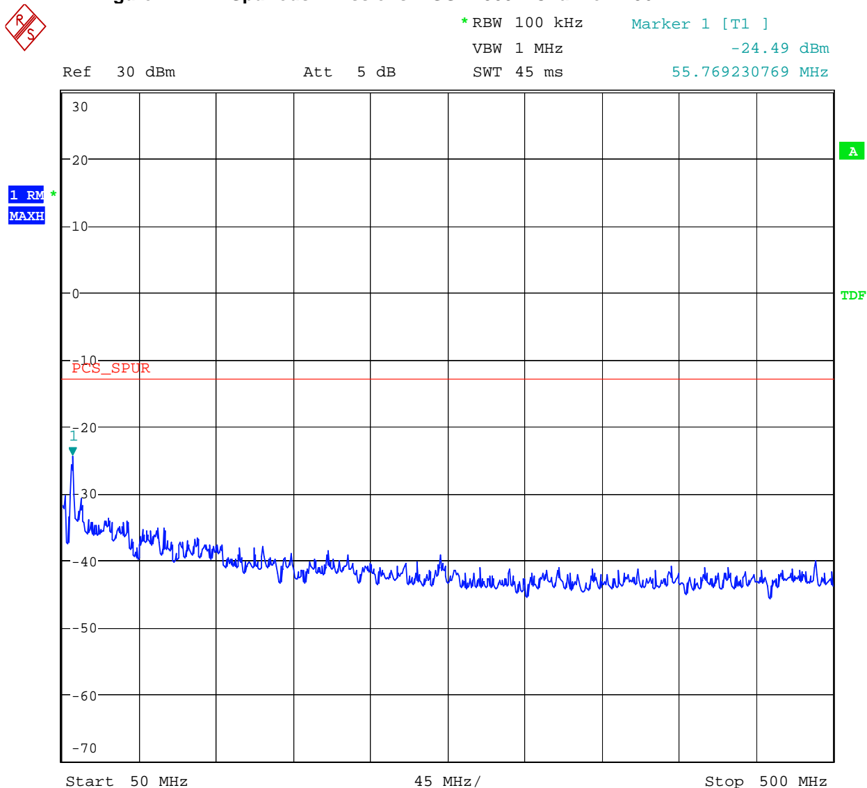
Figure 22 Spurious Emissions - GSM1900 – Channel 1196
