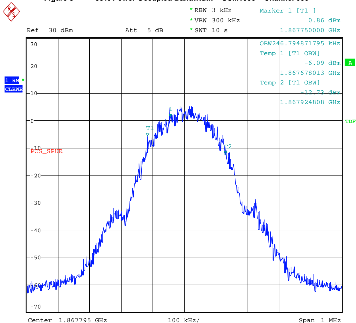
Figure 5 99% Power Occupied Bandwidth – GSM1900 – Channel 600
