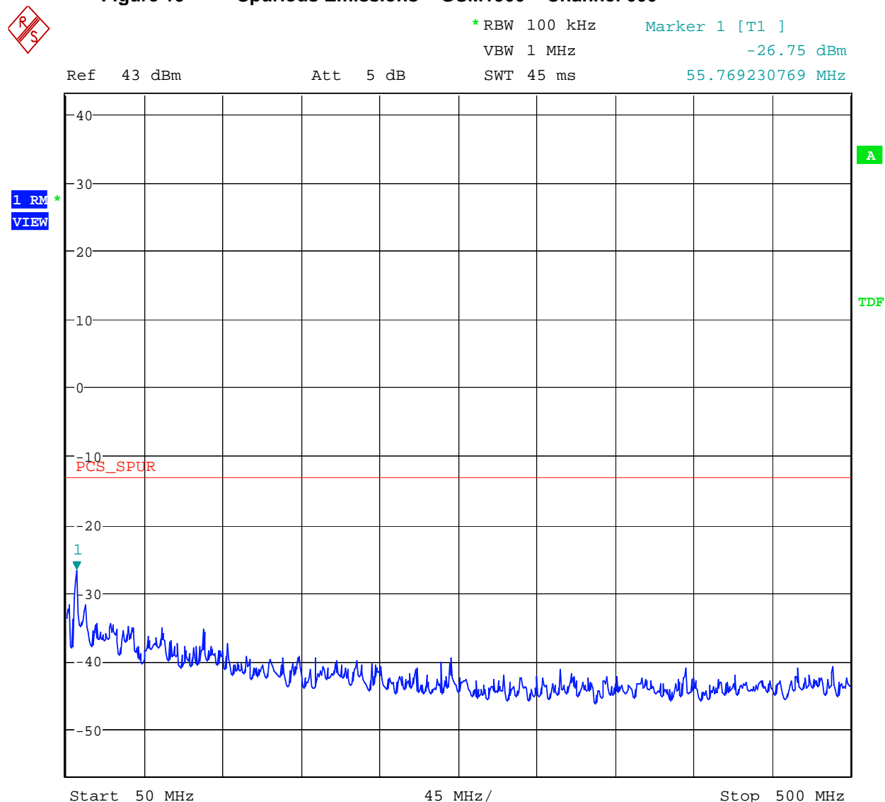
Figure 19 Spurious Emissions - GSM1900 – Channel 600
