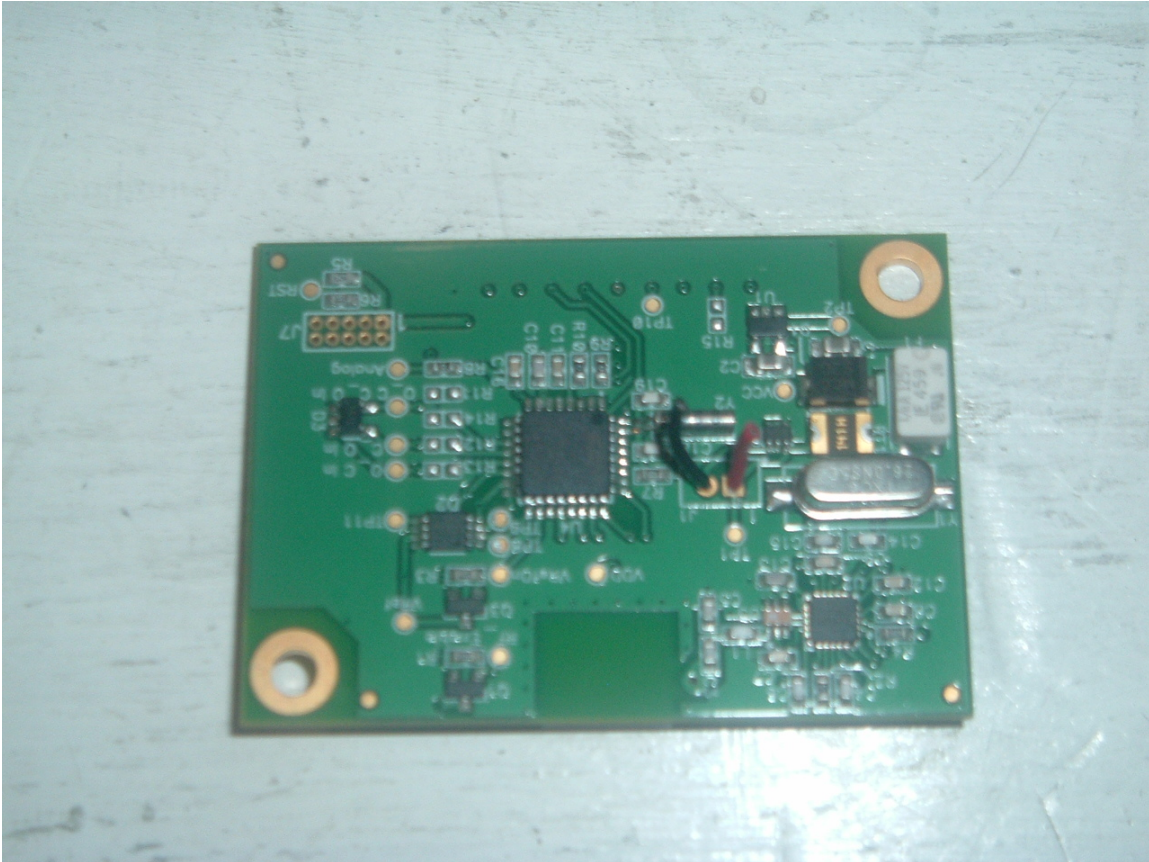
Photo 3 - Component side PCB
