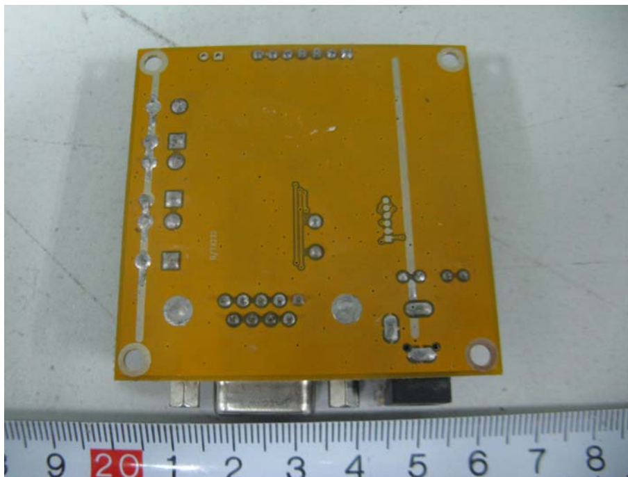
EUT- Test Board Bottom Components View
