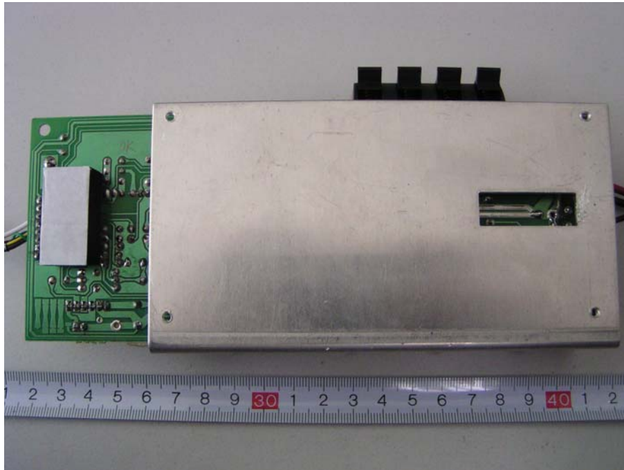
EUT-Audio PCB Rear View
