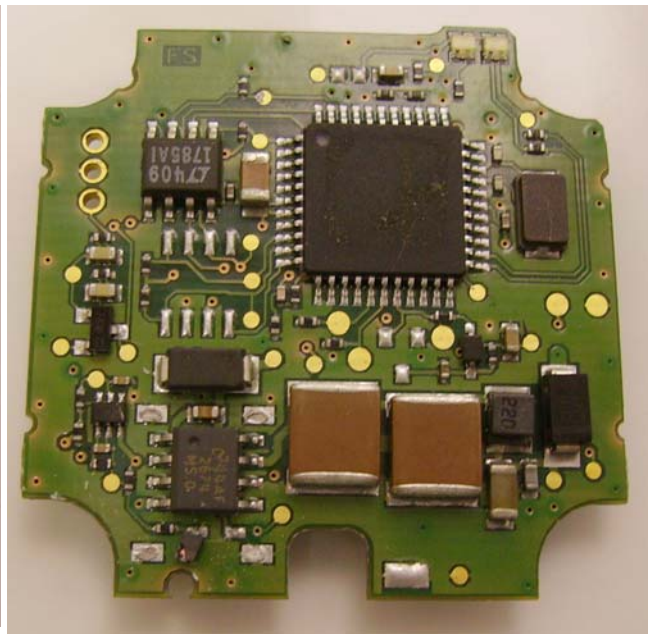
Solder side with metal shield removed
