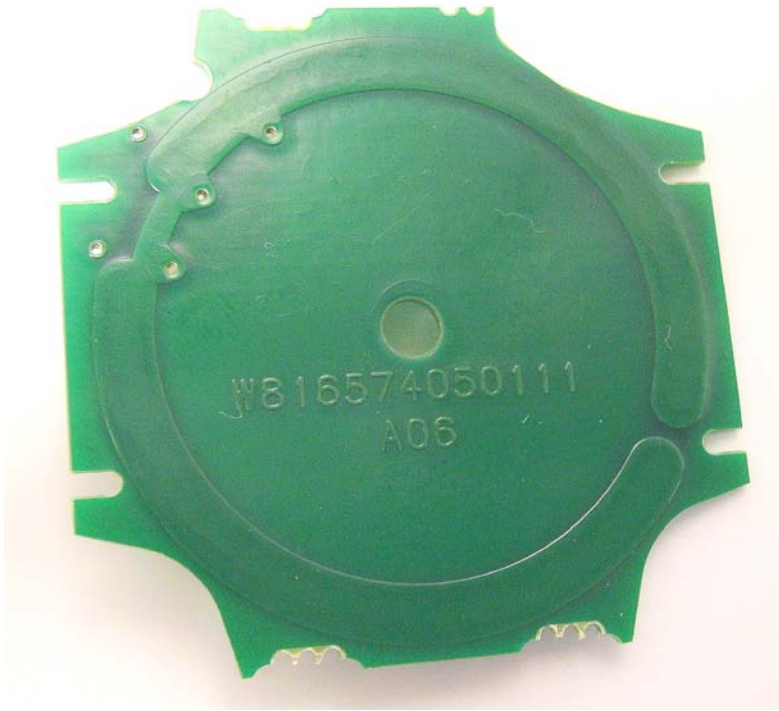
Coil side of the antenna board
