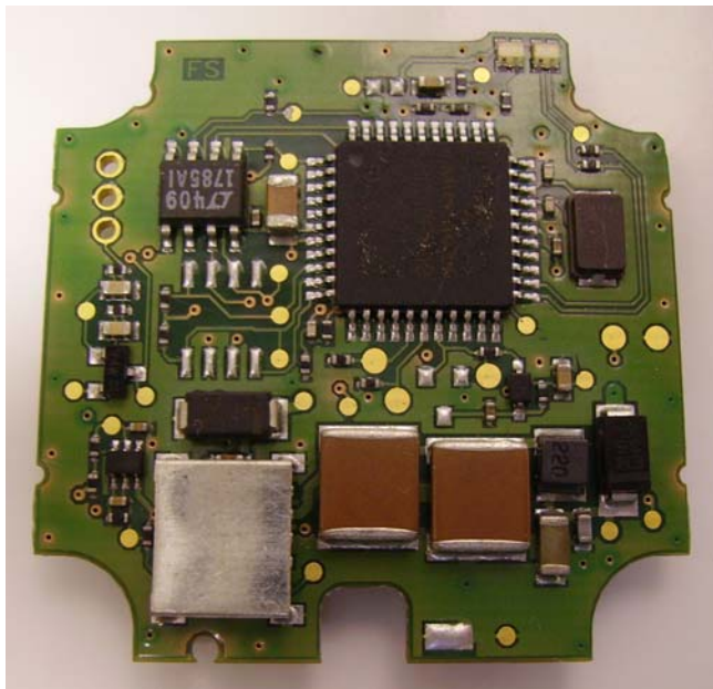
Solder side with metal shield
