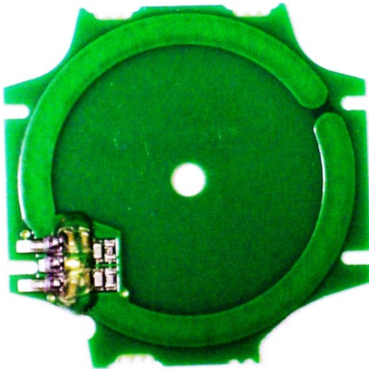
Component side of the antenna board
