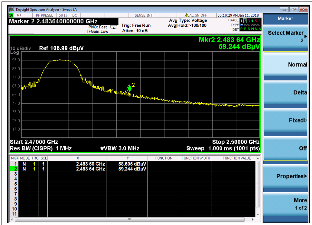
(Channel = 24, PEAK, 16QAM)
