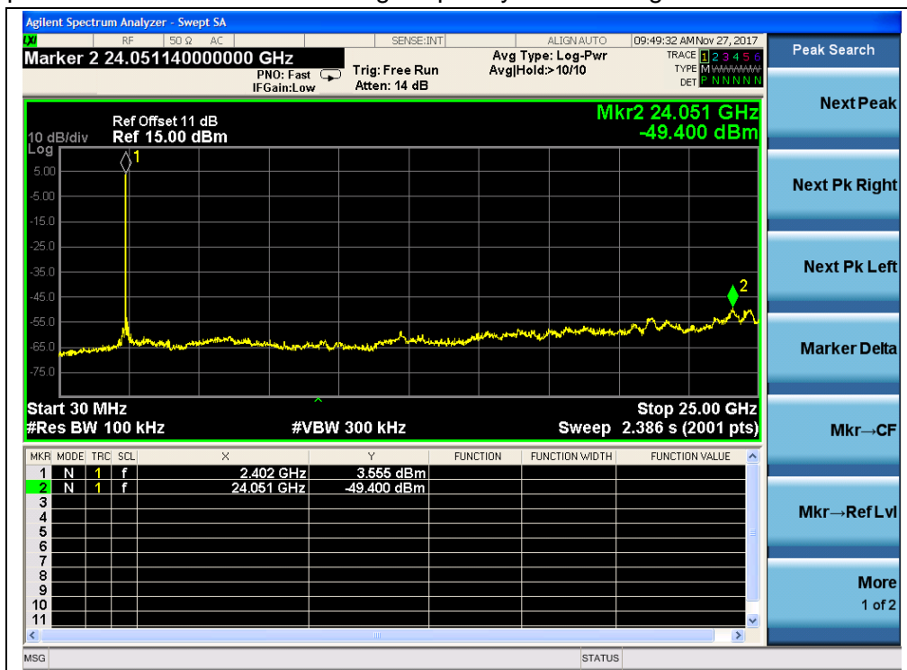
(16QAM, Channel = 1, 30MHz to 25GH)
