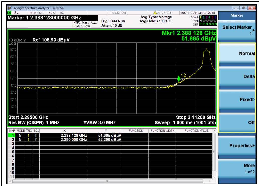
(Channel = 1, PEAK, 16QAM)
