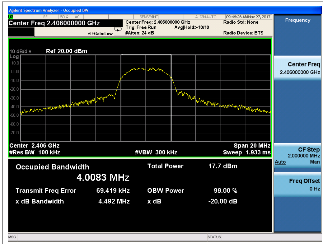
(16QAM, Channel 1, 2406MHz)
