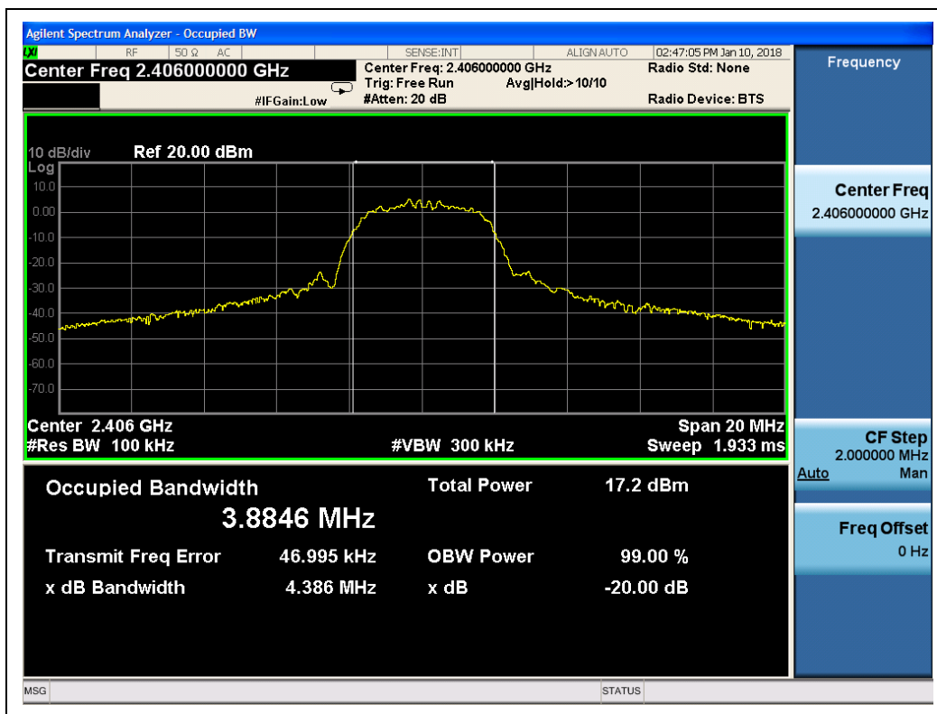
(BPSK, Channel 1, 2406MHz)
