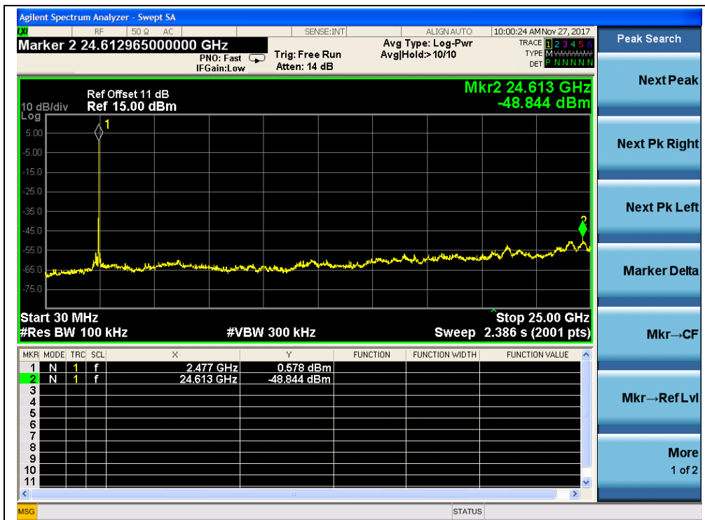
(16QAM, Channel = 24, 30MHz to 25GHz)
