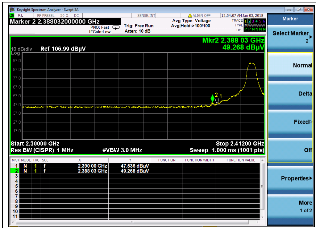
(Channel = 1, PEAK, QPSK)
