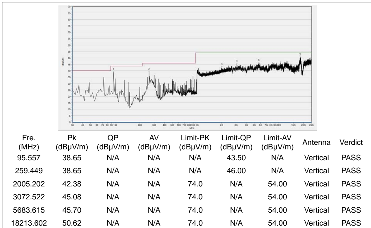
(30MHz to 25GHz, Antenna Vertical, BPSK)
