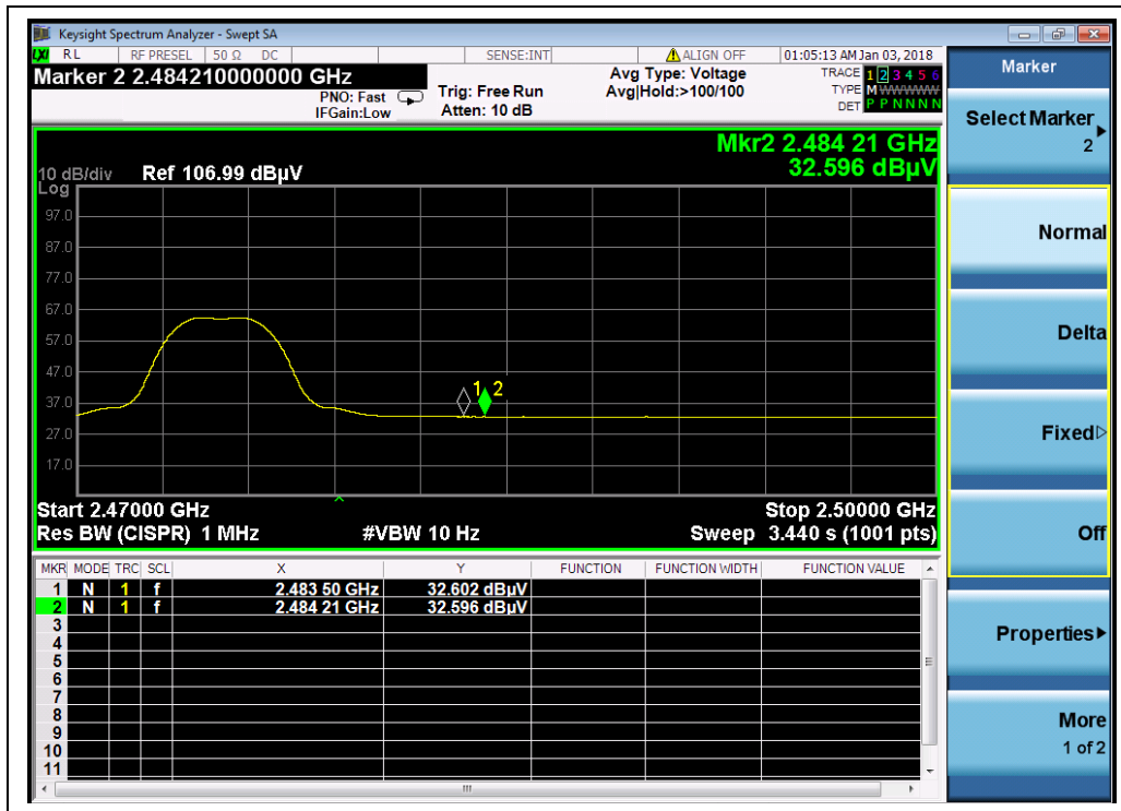
(Channel = 24, AVERAGE, QPSK)
