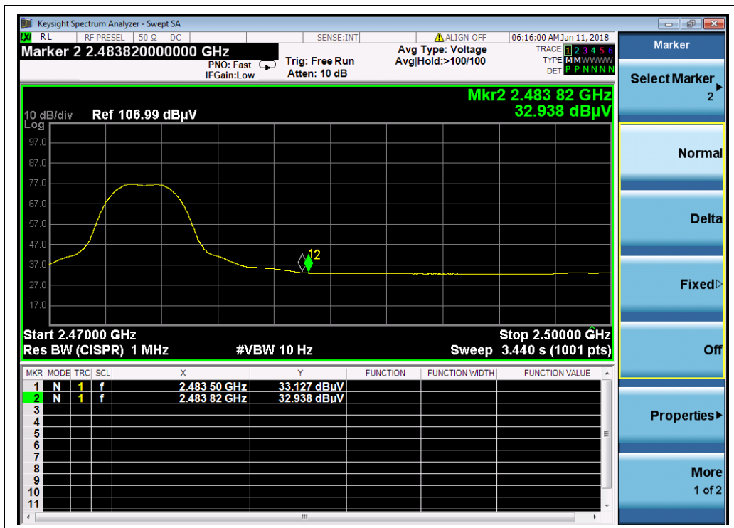
(Channel = 24, AVERAGE, 16QAM)
