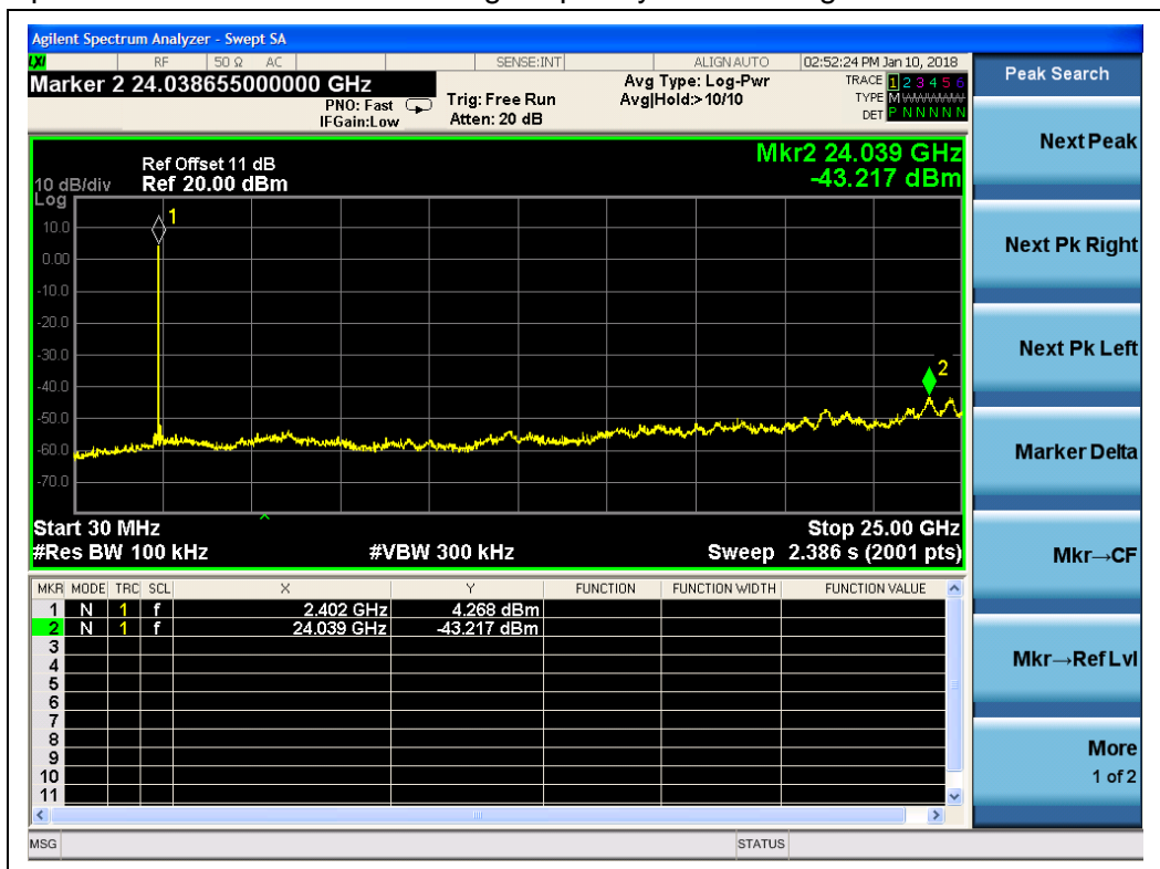
(BPSK, Channel = 1, 30MHz to 25GHz,)
