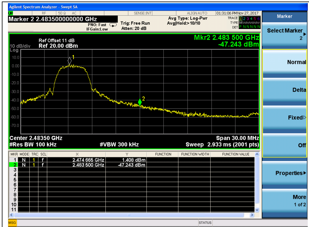
(BPSK, Channel = 24, Band edge)
