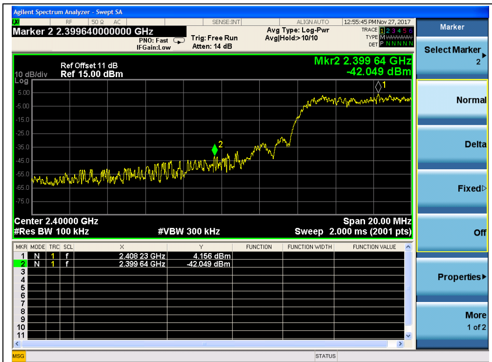
(QPSK, Channel = 1, Band edge with hopping on)
