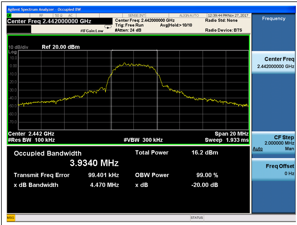
(QPSK, Channel 13, 2442MHz)
