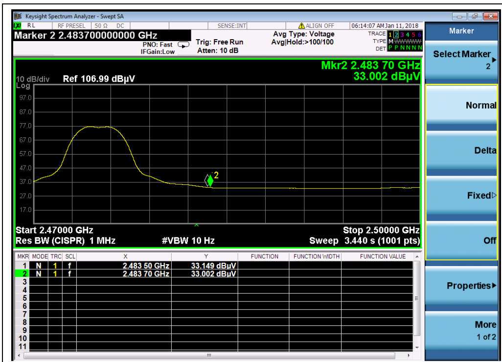
(Channel = 24, AVERAGE, BPSK)
