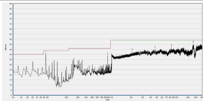
(30MHz to 25GHz, Antenna Horizontal, 16QAM)
