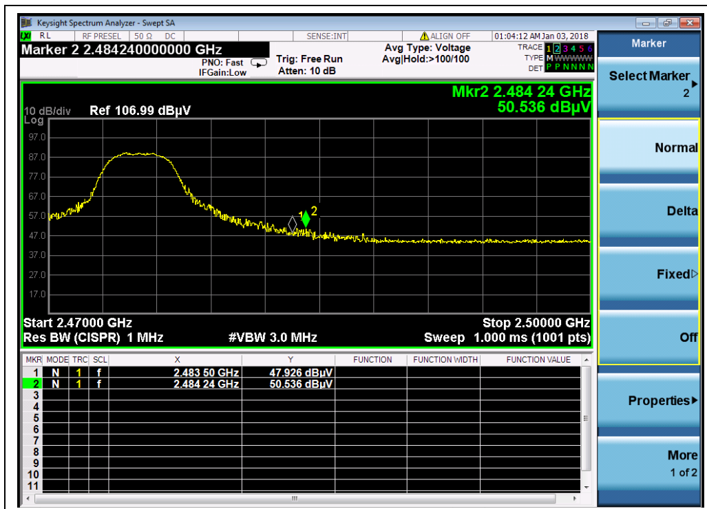
(Channel = 24, PEAK, QPSK)
