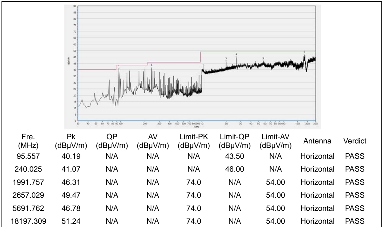
(30MHz to 25GHz, Antenna Horizontal, 16QAM)
