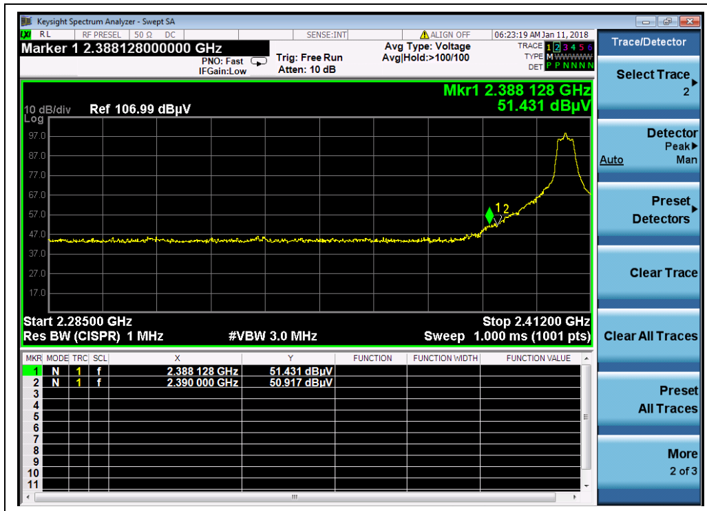
(Channel = 1, PEAK, BPSK)
