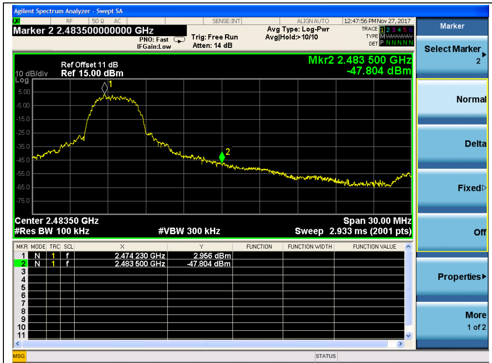
(QPSK, Channel = 24, Band edge)
