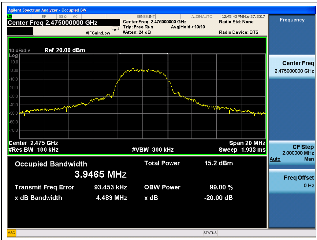
(QPSK, Channel 24, 2475MHz)
