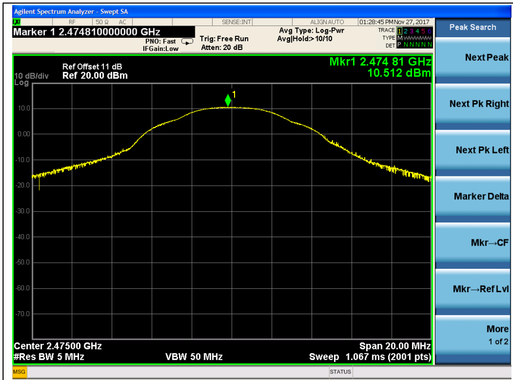
(BPSK, Channel 24, 2475MHz)
