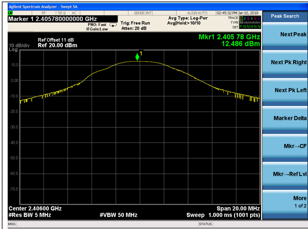
(BPSK, Channel 1, 2406MHz)
