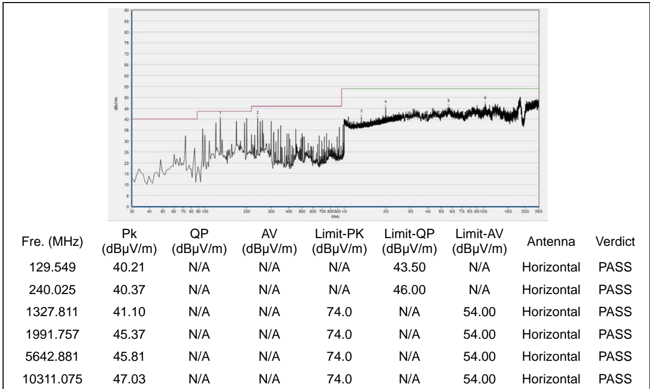
(30MHz to 25GHz, Antenna Horizontal, BPSK)
