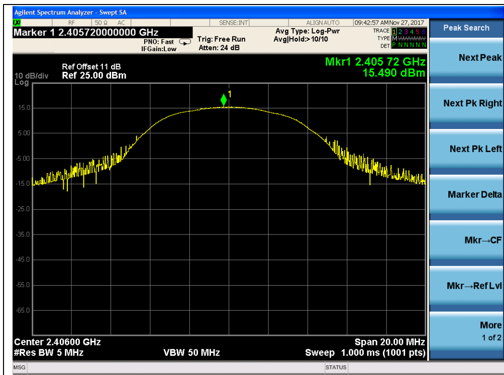
(16QAM, Channel 1, 2406MHz)
