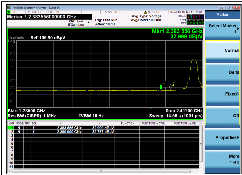
(Channel = 1, AVERAGE, BPSK)
