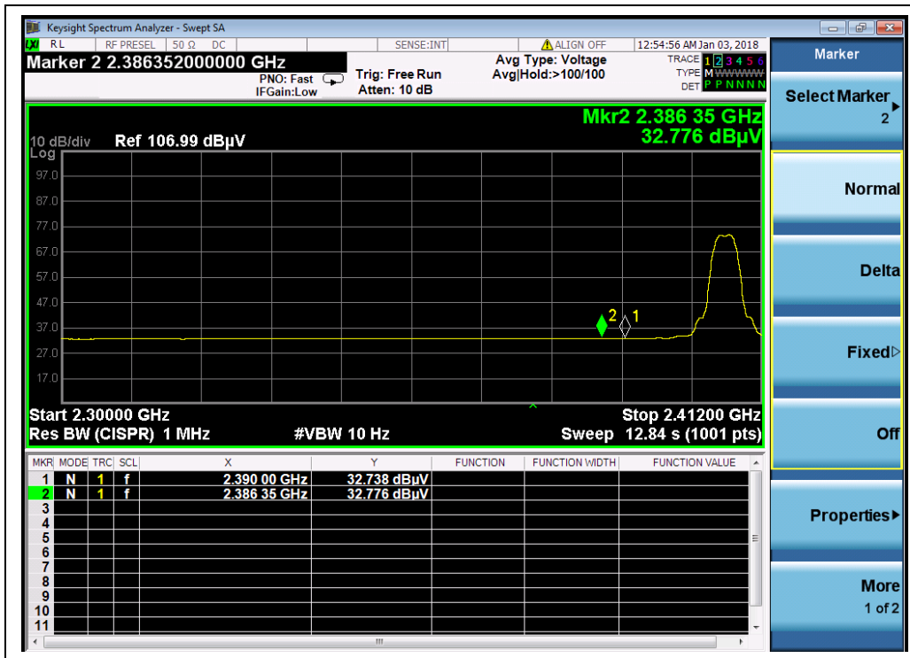
(Channel = 1, AVERAGE, QPSK)
