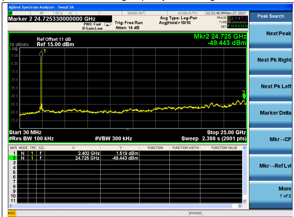
(QPSK, Channel = 1, 30MHz to 25GHz)
