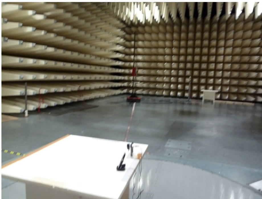
Photo 2: Radiated Emission
