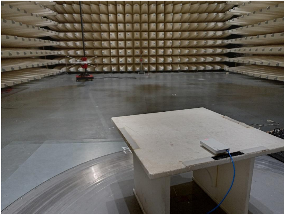
Photo 3: Radiated Emission
