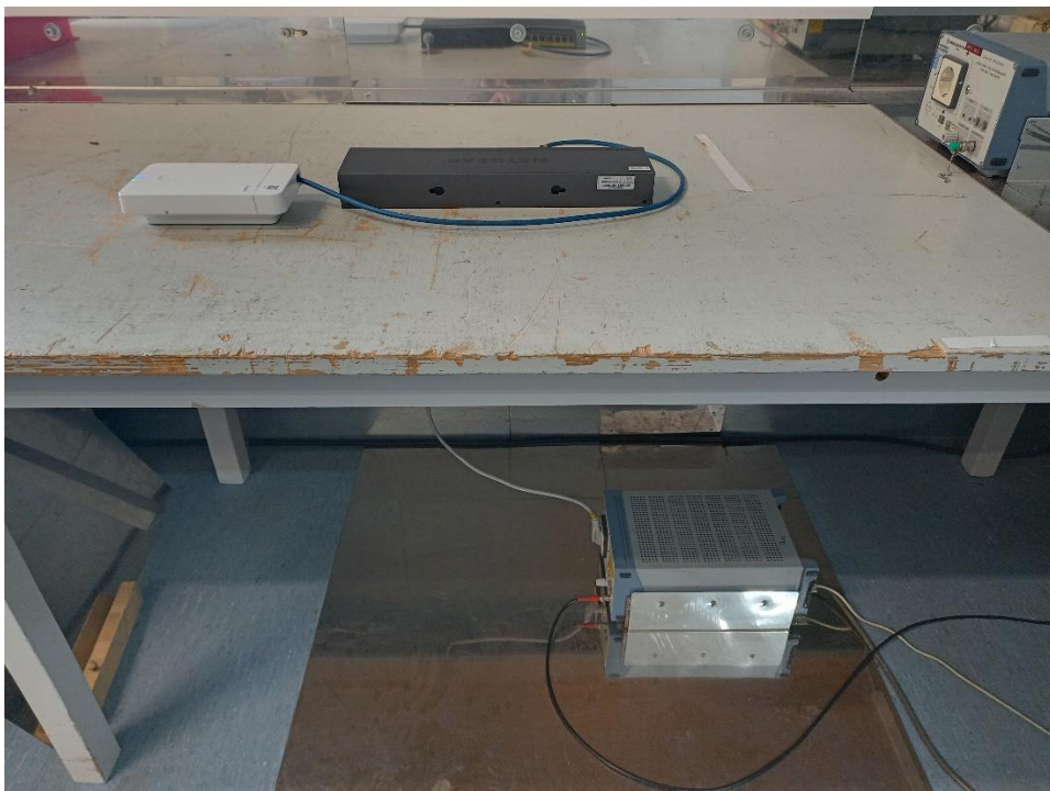
Photo 6: Conducted Emission
