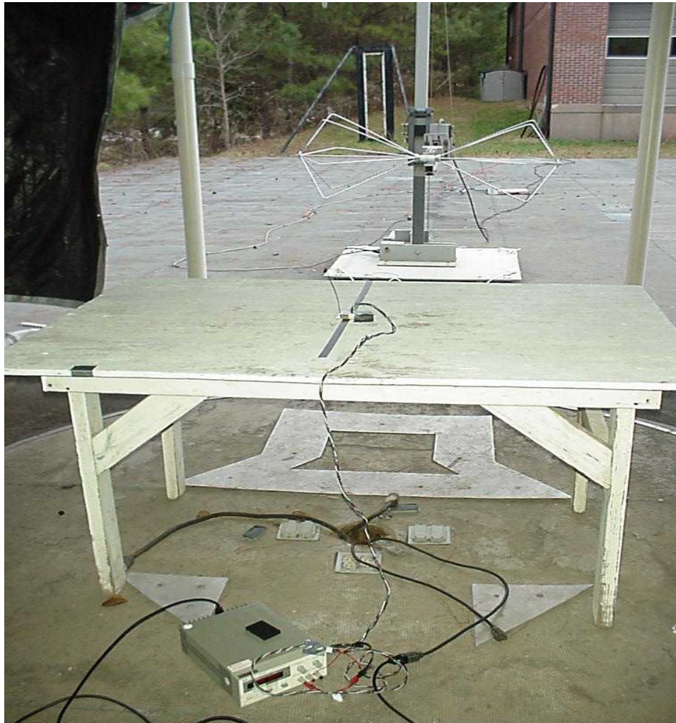
Figure 2b. Photograph of Spurious Radiation Test Setup, Rear View.
