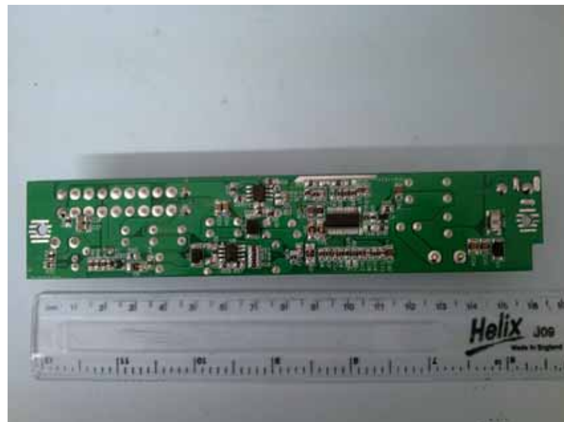
Underside View of Power Supply PCB
