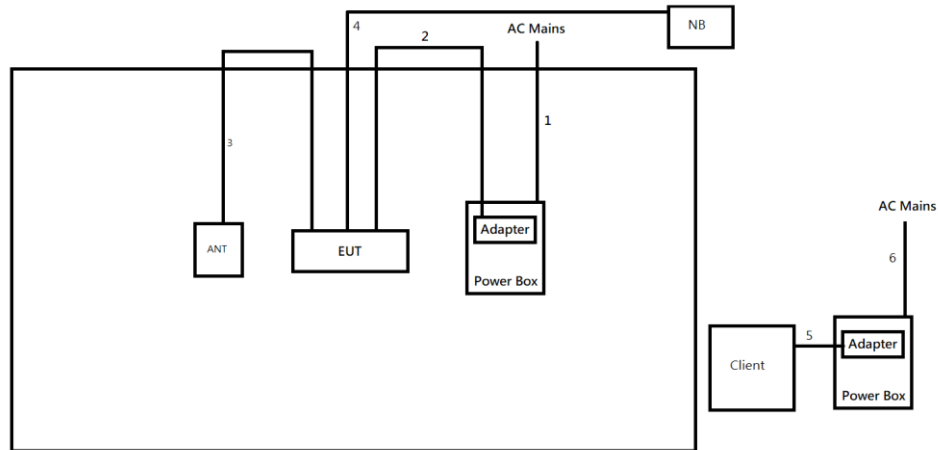
Test Setup Diagram - Radiated Test (Beamforming)
