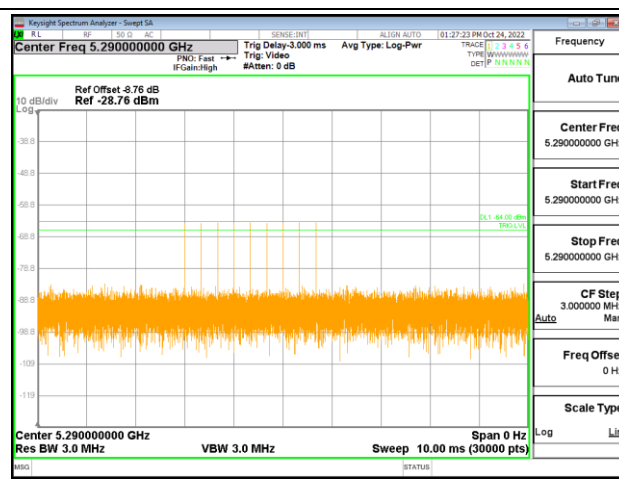
Single Burst of Radar Type 6
