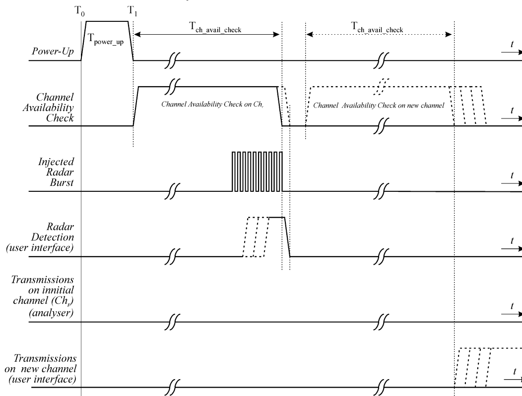
Figure 16: Example of timing for radar testing towards the end of the Channel Availability Check
