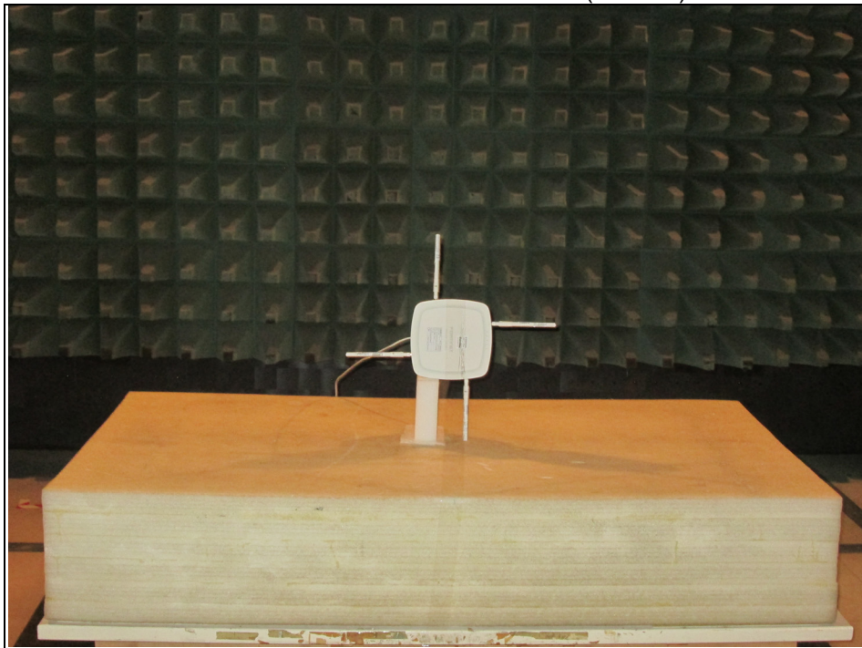
Radiated Emission Test below 1GHz (Mode D)
