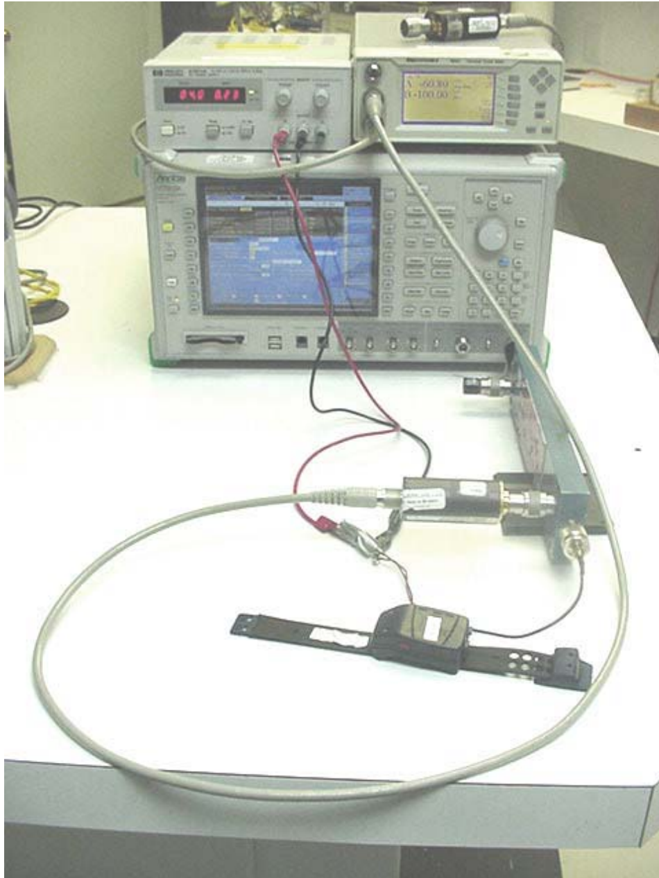
Photograph A.7-1-2-3 - Conducted Power Measurement Setup
