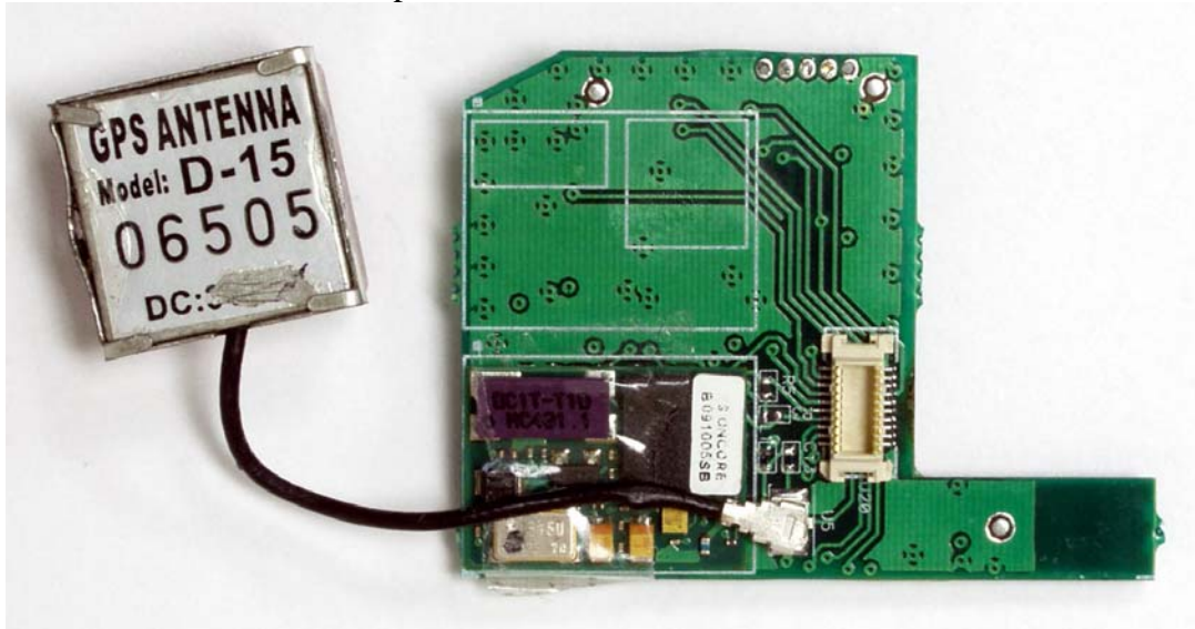
Top-board with GPS-RX – Bottom
