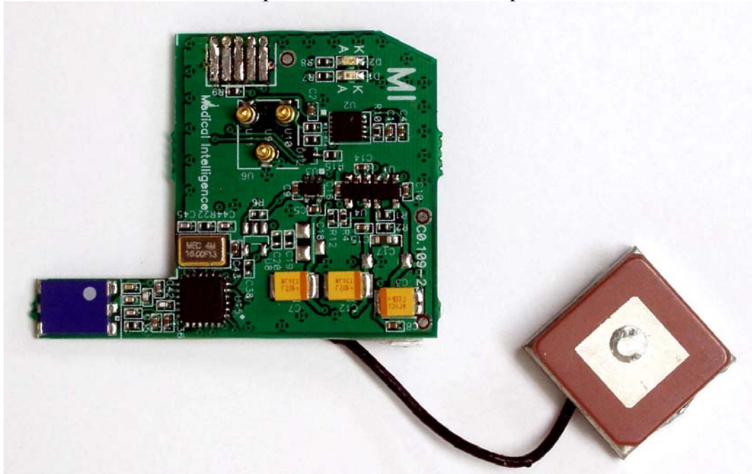
Top-board with GPS-RX – Top
