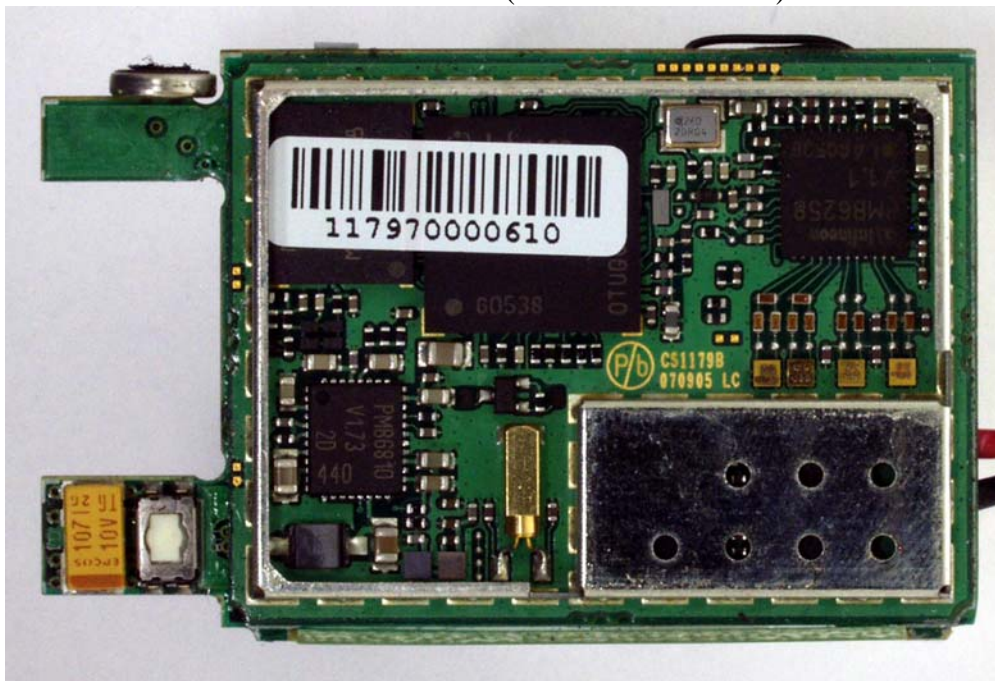
Main-board– Bottom (inside GSM-module)
