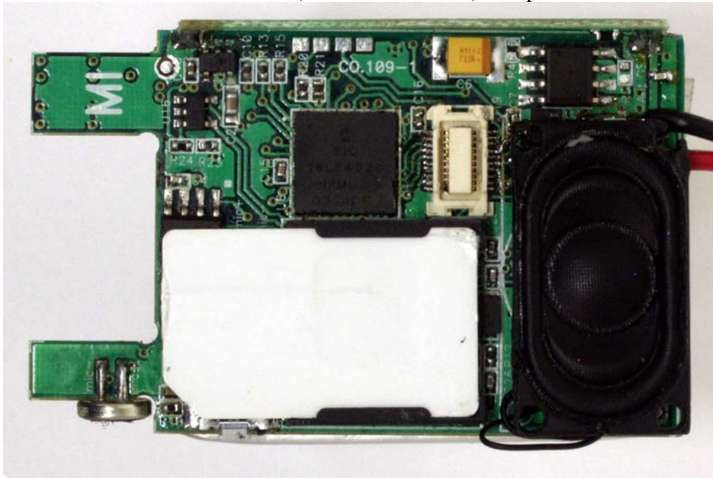
Main-board (with GSM-module) – Top
