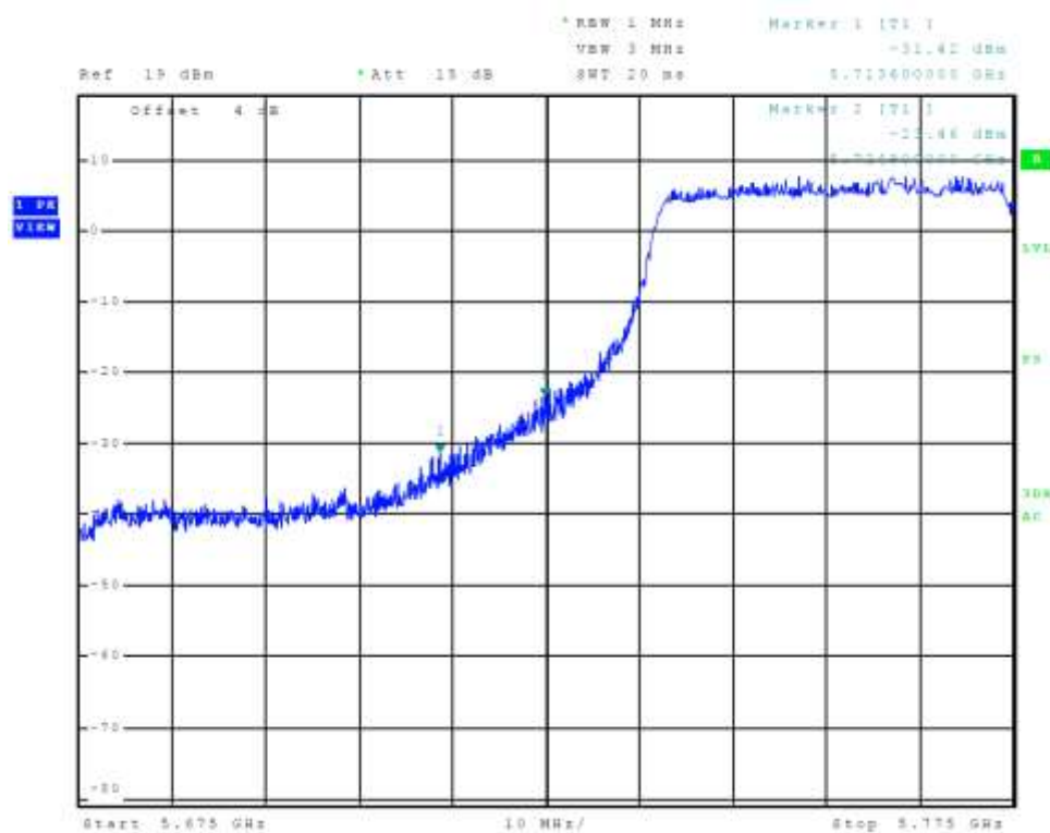
Figure 93 Plot of Transmitter Low Band Edge Chain 2 (5725-5850 MHz Band, 802.11ac)
