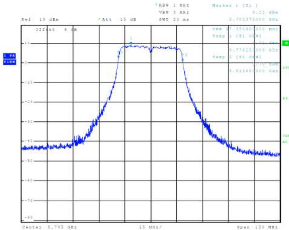
Figure 29 Plot of Transmitter Emissions Chain 0 (5725-5850 MHz Band, 802.11n40, 99% OBW)
