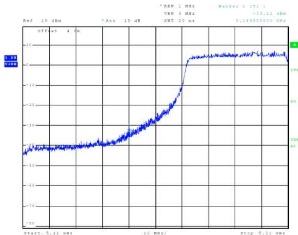
Figure 78 Plot of Transmitter Low Band Edge Chain 2 (5150-5250 MHz Band, 802.11ac)
