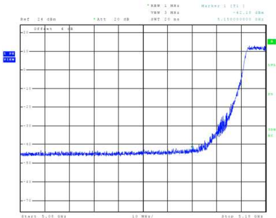
Figure 76 Plot of Transmitter Low Band Edge Chain 2 (5150-5250 MHz Band, 802.11a)
