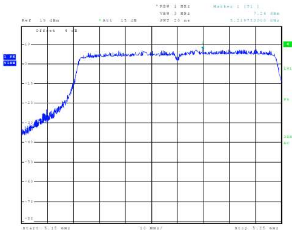
Figure 75 Plot of Transmitter Emissions Chain 2 (Across 5150-5250 MHz Band, 802.11ac)
