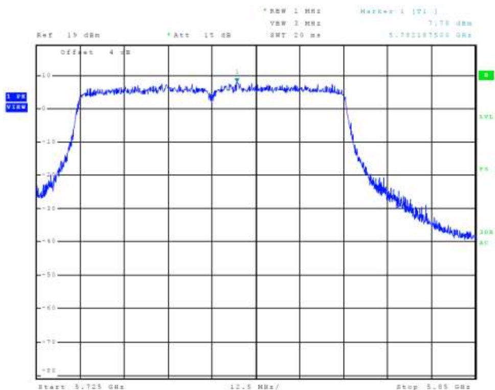
Figure 90 Plot of Transmitter Emissions Chain 2 (Across 5725-5850 MHz Band, 802.11ac)
