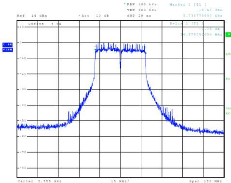
Figure 30 Plot of Transmitter Emissions Chain 0 (5725-5850 MHz Band, 802.11n40, 6-dB OBW)
