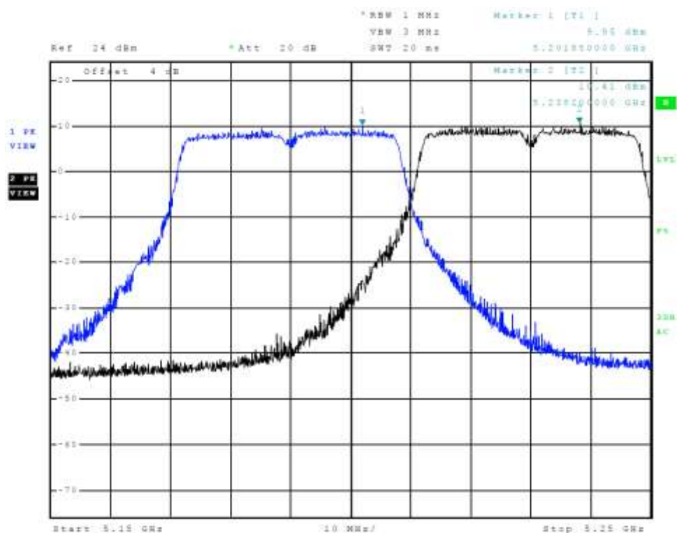
Figure 34 Plot of Transmitter Emissions Chain 1 (Across 5150-5250 MHz Band, 802.11n40)
