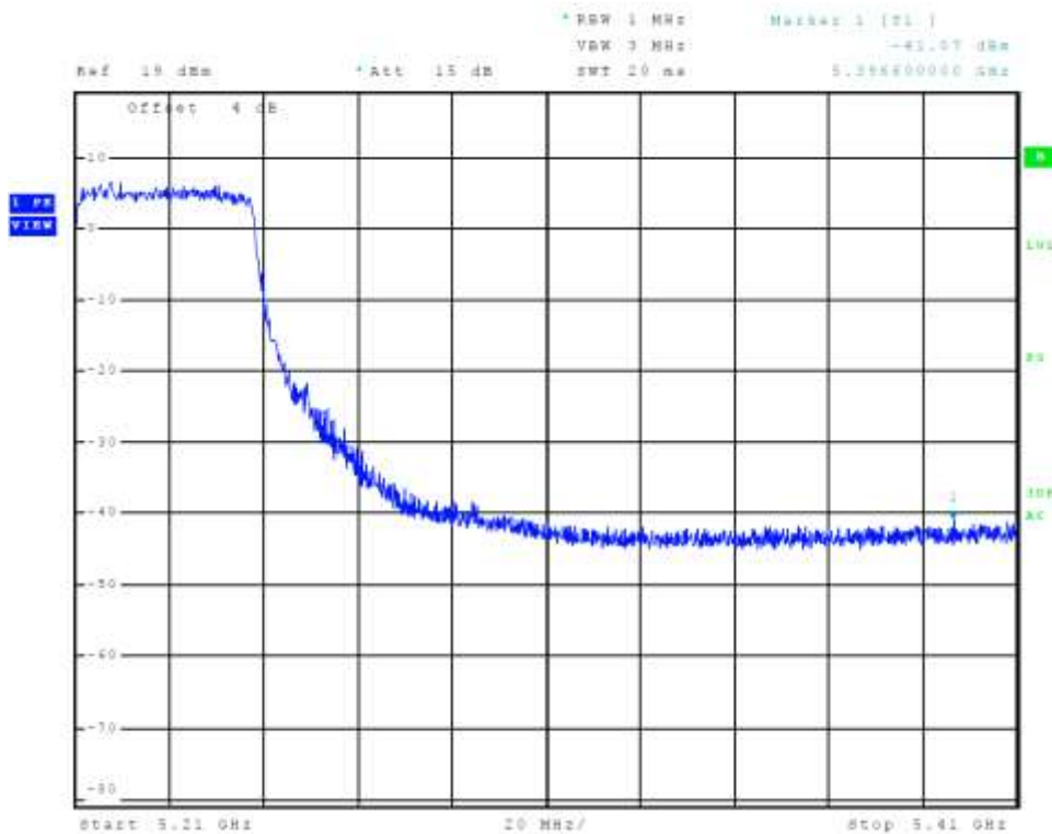
Figure 41 Plot of Transmitter High Band Edge Chain 1 (5150-5250 MHz Band, 802.11ac)
