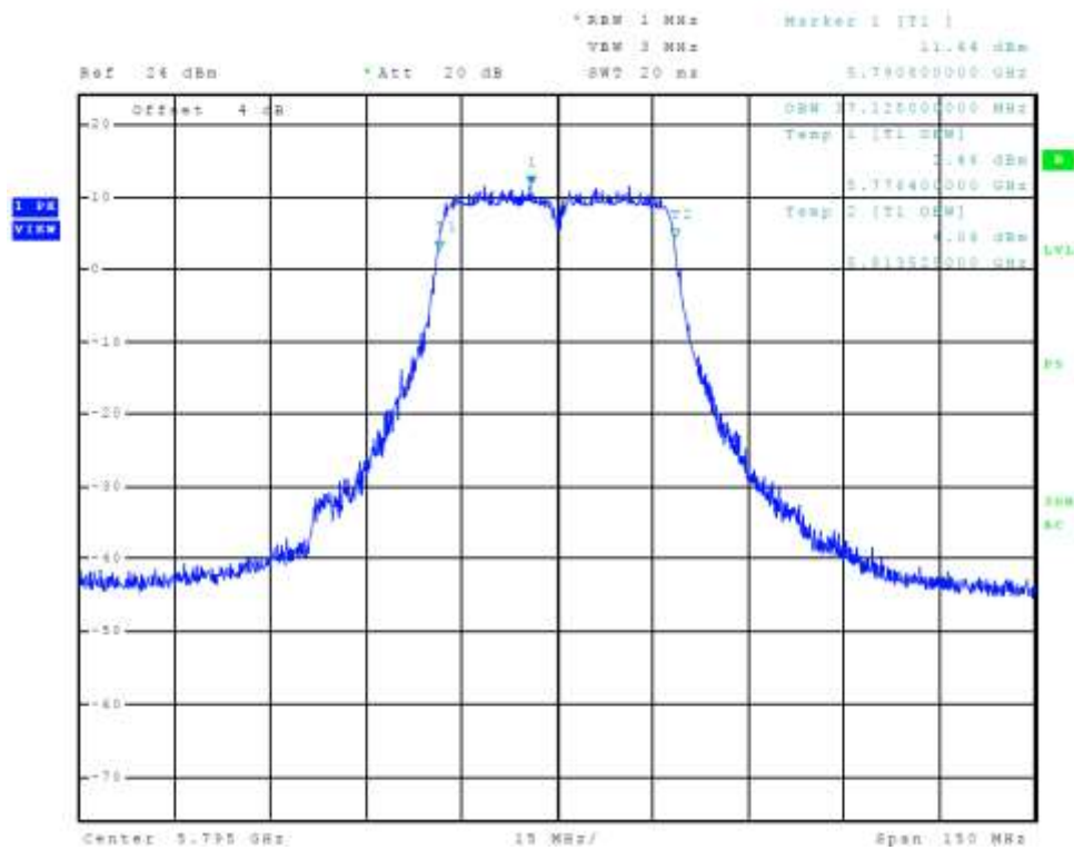
Figure 99 Plot of Transmitter Emissions Chain 2 (5725-5850 MHz Band, 802.11n40, 99% OBW)
