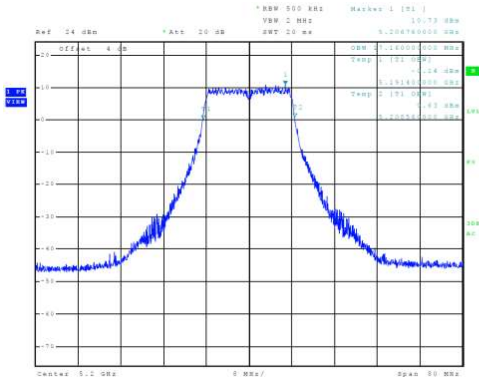
Figure 82 Plot of Transmitter Emissions Chain 2 (5150-5250 MHz Band, 802.11a, 99% OBW)
