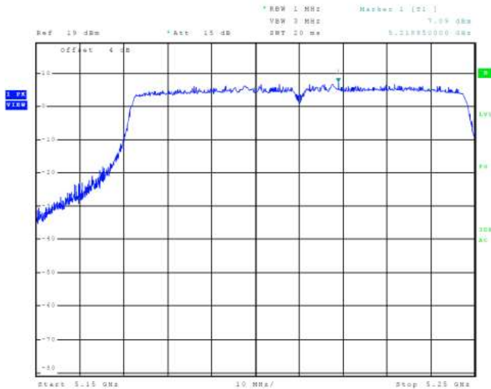
Figure 35 Plot of Transmitter Emissions Chain 1 (Across 5150-5250 MHz Band, 802.11ac)
