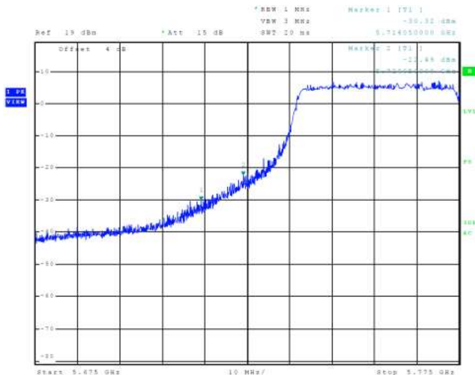
Figure 53 Plot of Transmitter Low Band Edge Chain 1 (5725-5850 MHz Band, 802.11ac)
