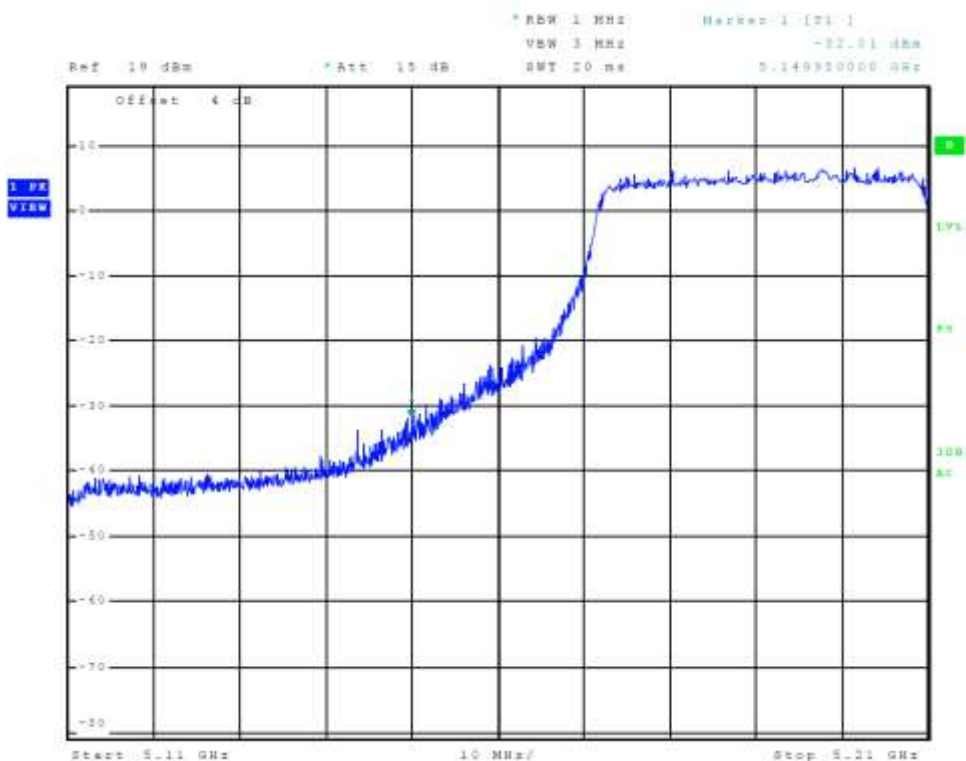
Figure 38 Plot of Transmitter Low Band Edge Chain 1 (5150-5250 MHz Band, 802.11ac)
