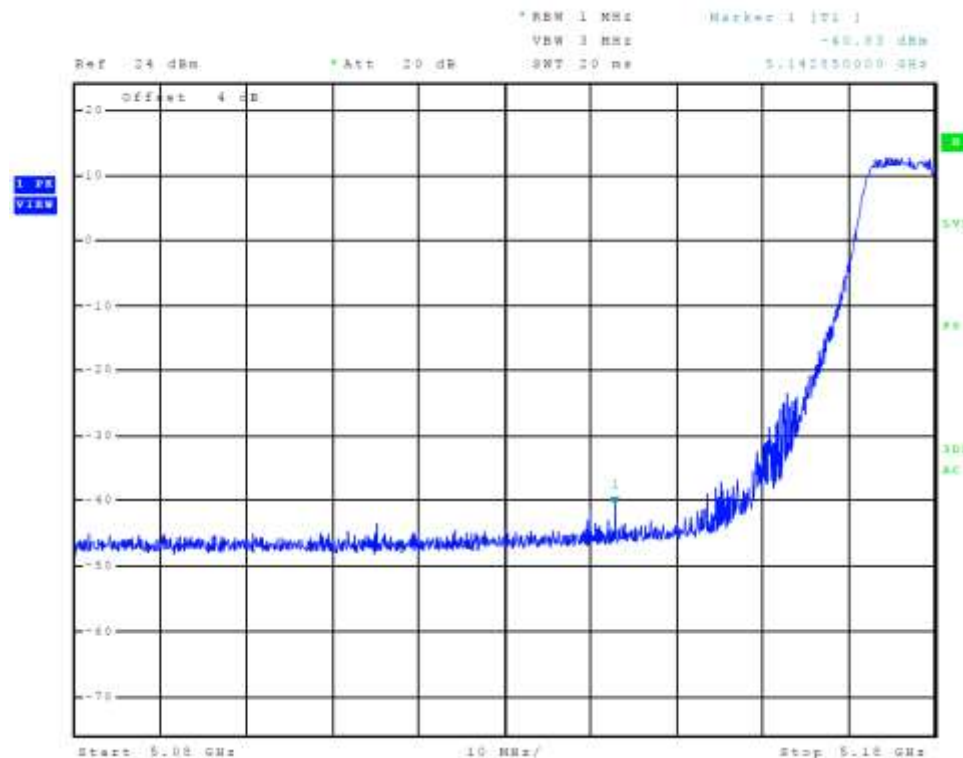
Figure 36 Plot of Transmitter Low Band Edge Chain 1 (5150-5250 MHz Band, 802.11a)
