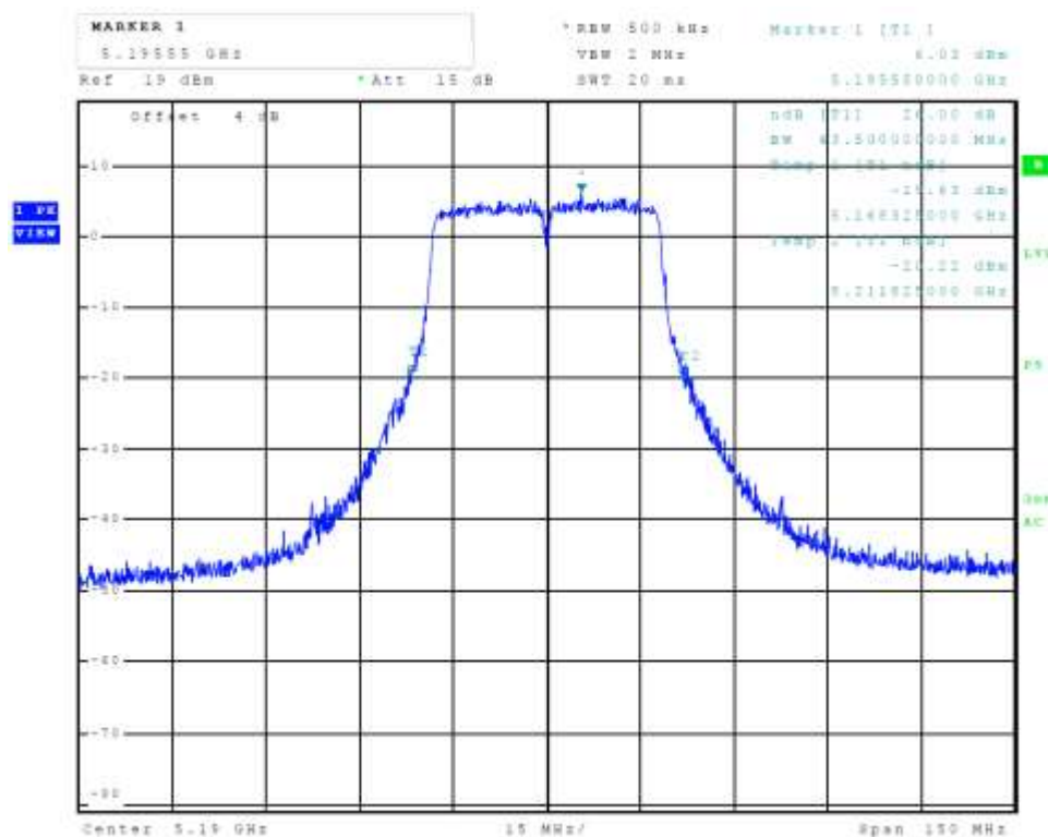
Figure 45 Plot of Transmitter Emissions Chain 1 (5150-5250 MHz Band, 802.11n40, 26 dB OBW)
