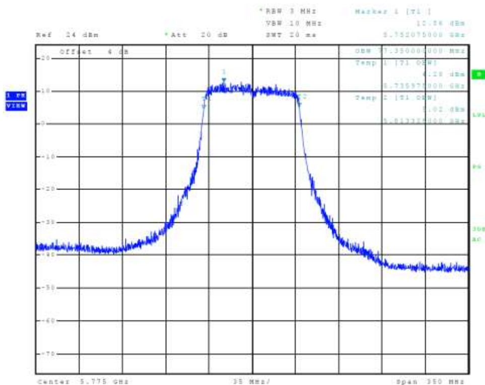
Figure 61 Plot of Transmitter Emissions Chain 1 (5725-5850 MHz Band, 802.11ac, 99% OBW)
