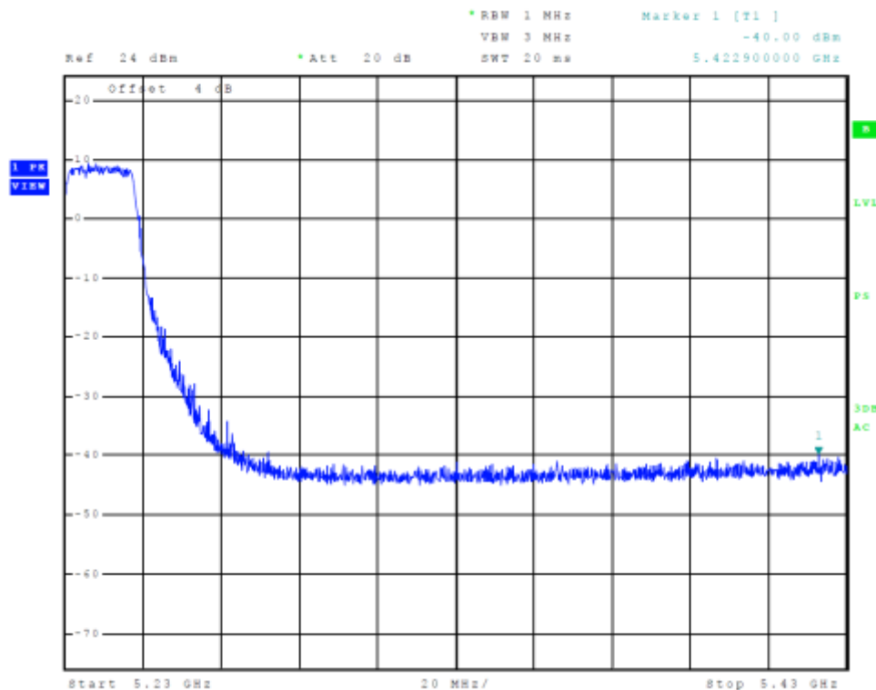
Figure 40 Plot of Transmitter High Band Edge Chain 1 (5150-5250 MHz Band, 802.11n40)
