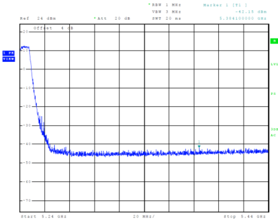
Figure 9 Plot of Transmitter High Band Edge Chain 0 (5150-5250 MHz Band, 802.11a)
