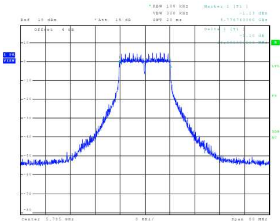
Figure 98 Plot of Transmitter Emissions Chain 2 (5725-5850 MHz Band, 802.11a, 6-dB OBW)
