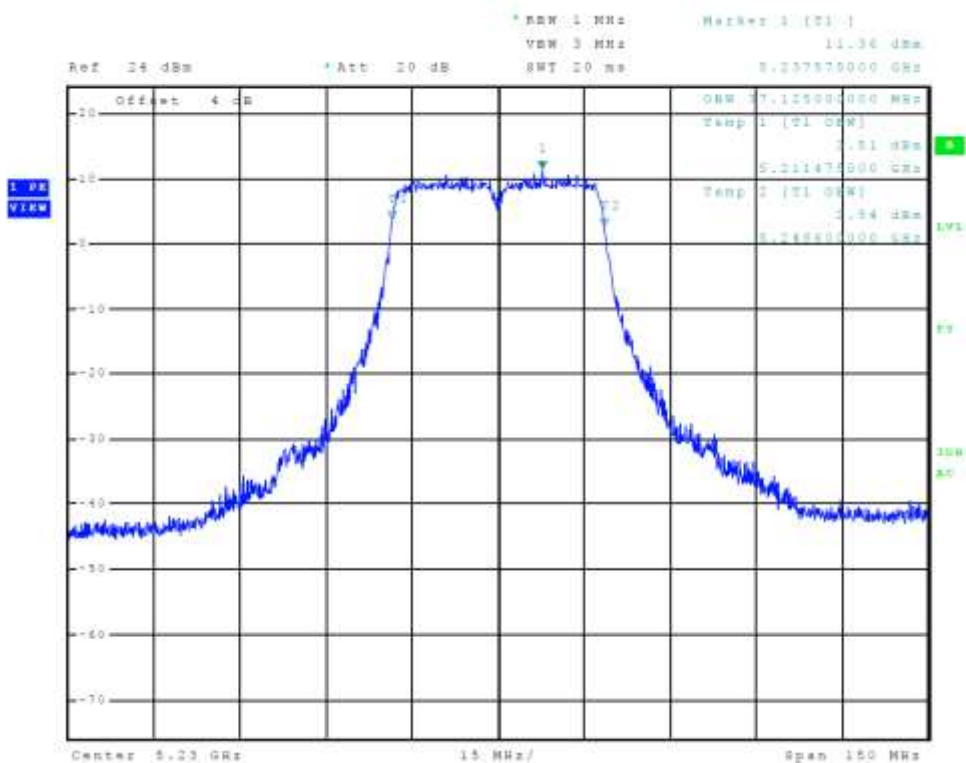
Figure 84 Plot of Transmitter Emissions Chain 2 (5150-5250 MHz Band, 802.11n40, 99% OBW)
