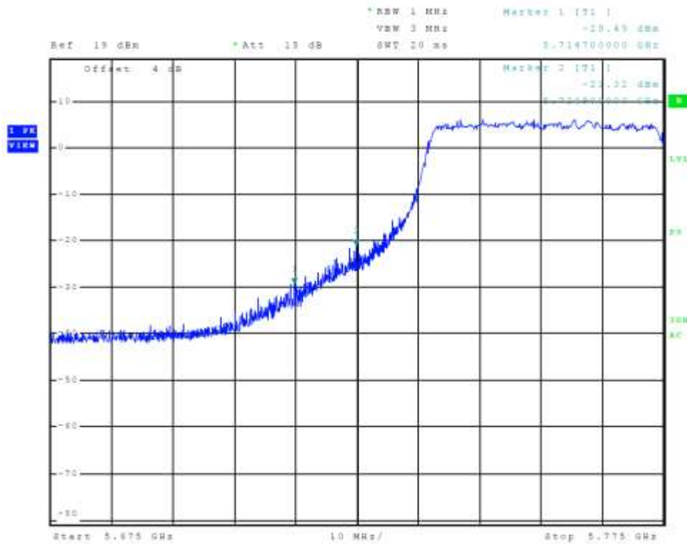
Figure 23 Plot of Transmitter Low Band Edge Chain 0 (5725-5850 MHz Band, 802.11ac)
