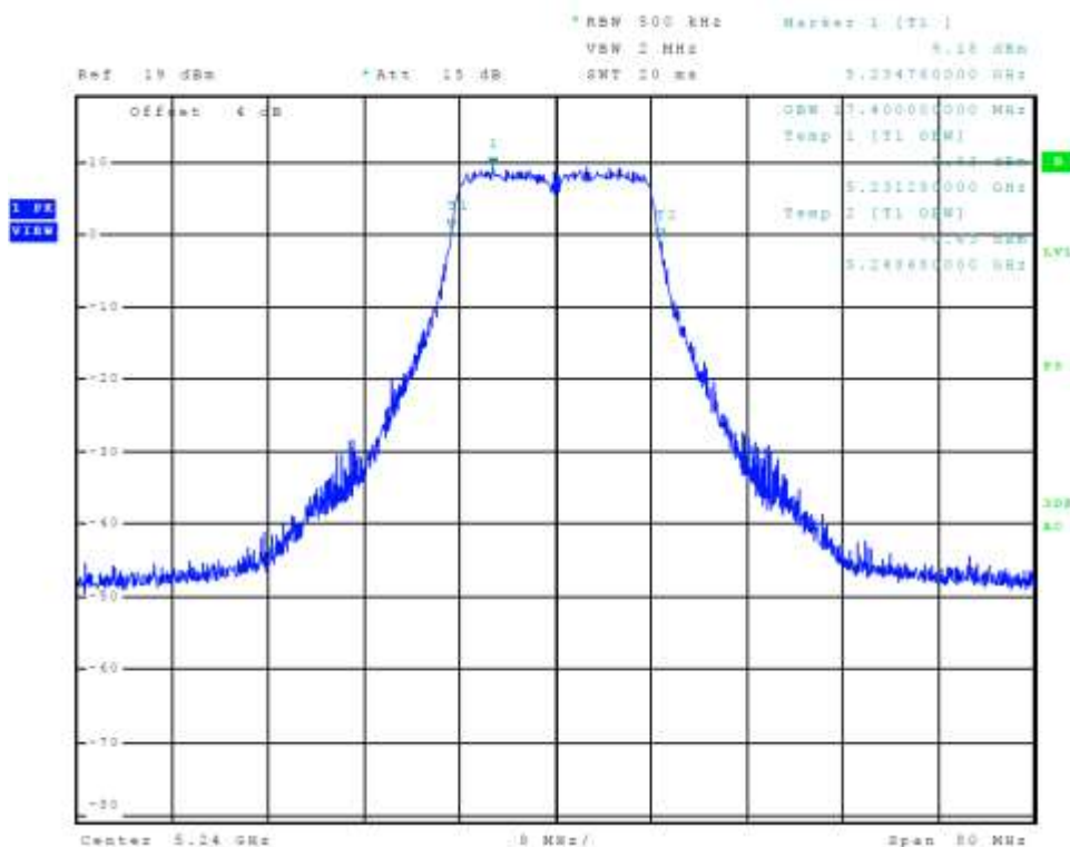
Figure 12 Plot of Transmitter Emissions Chain 0 (5150-5250 MHz Band, 802.11a, 99% OBW)
