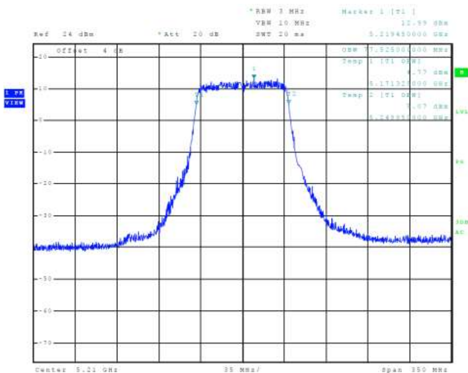
Figure 46 Plot of Transmitter Emissions Chain 1 (5150-5250 MHz Band, 802.11ac, 99% OBW)
