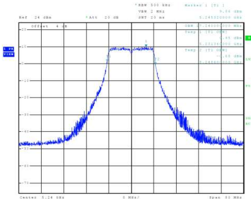
Figure 42 Plot of Transmitter Emissions Chain 1 (5150-5250 MHz Band, 802.11a, 99% OBW)
