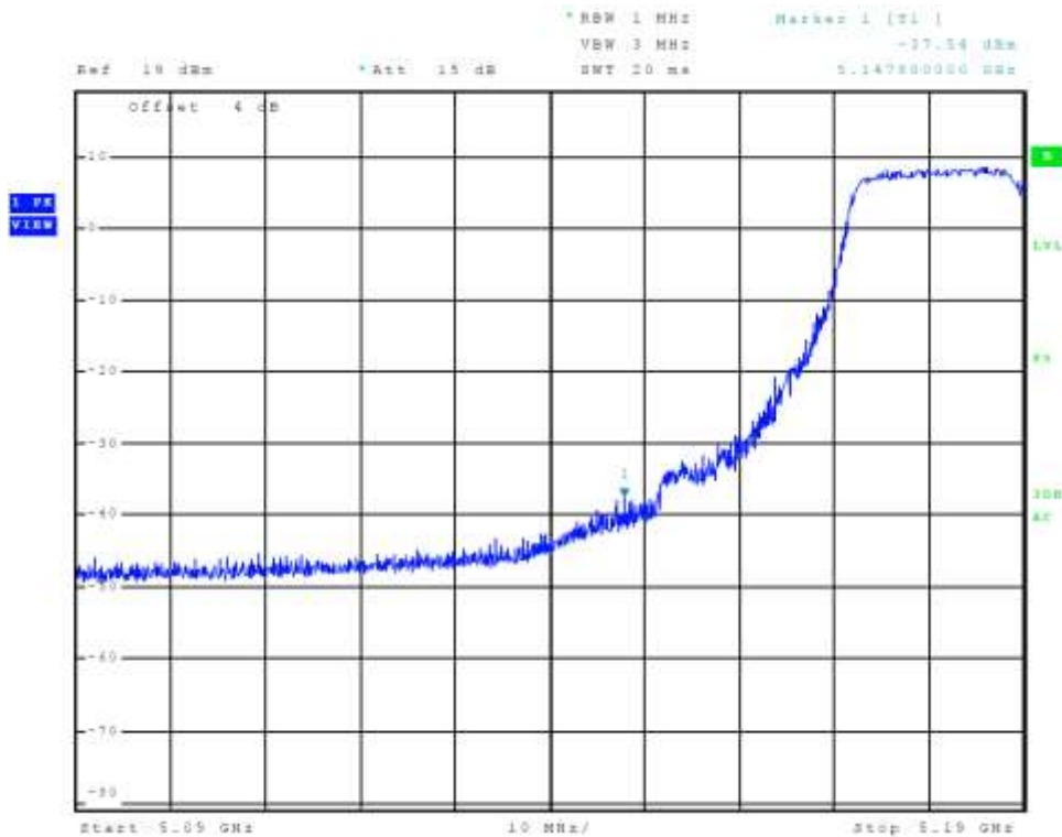
Figure 7 Plot of Transmitter Low Band Edge Chain 0 (5150-5250 MHz Band, 802.11n40)
