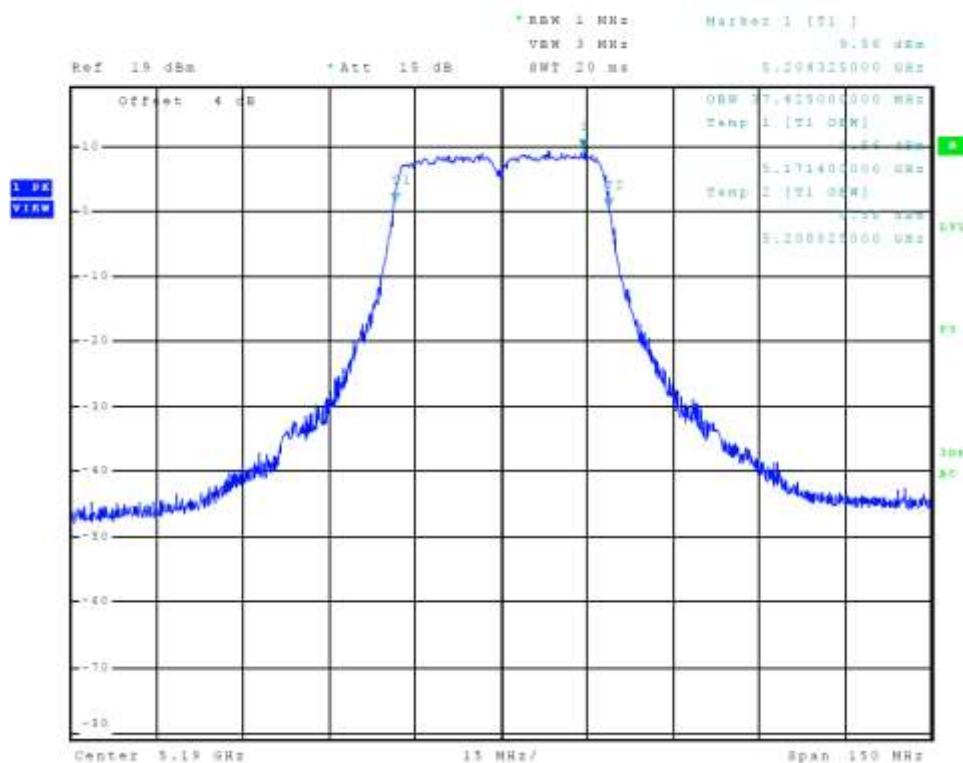
Figure 14 Plot of Transmitter Emissions Chain 0 (5150-5250 MHz Band, 802.11n40, 99% OBW)
