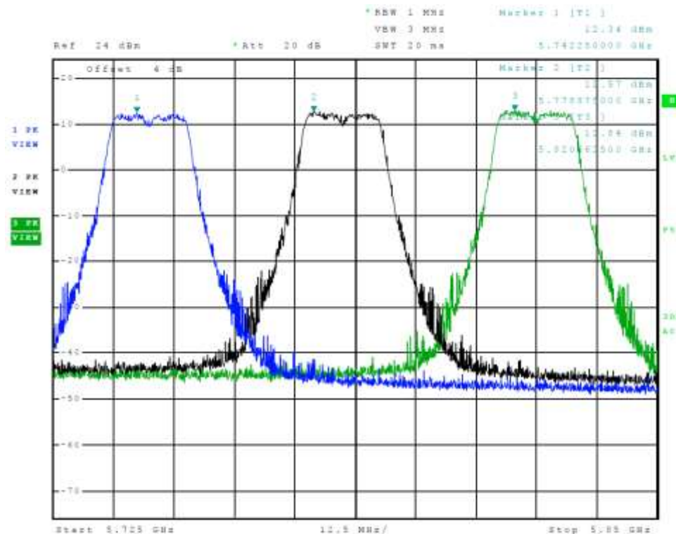
Figure 18 Plot of Transmitter Emissions Chain 0 (Across 5725-5850 MHz Band, 802.11a)
