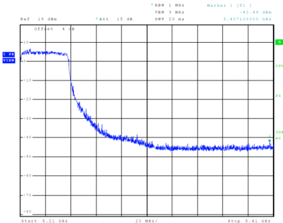
Figure 11 Plot of Transmitter High Band Edge Chain 0 (5150-5250 MHz Band, 802.11ac)
