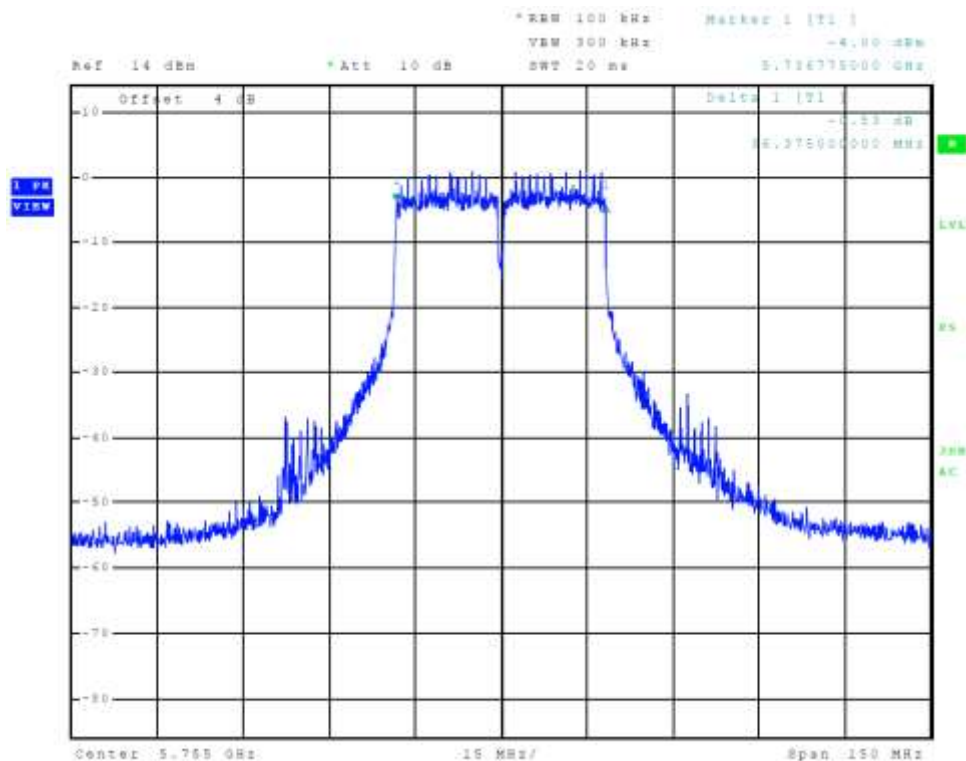
Figure 100 Plot of Transmitter Emissions Chain 2 (5725-5850 MHz Band, 802.11n40, 6-dB OBW)
