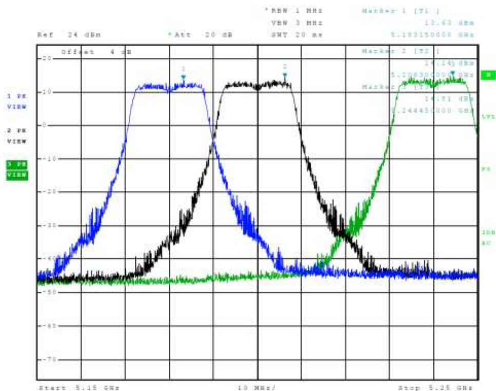
Figure 73 Plot of Transmitter Emissions Chain 2 (Across 5150-5250 MHz Band, 802.11a)
