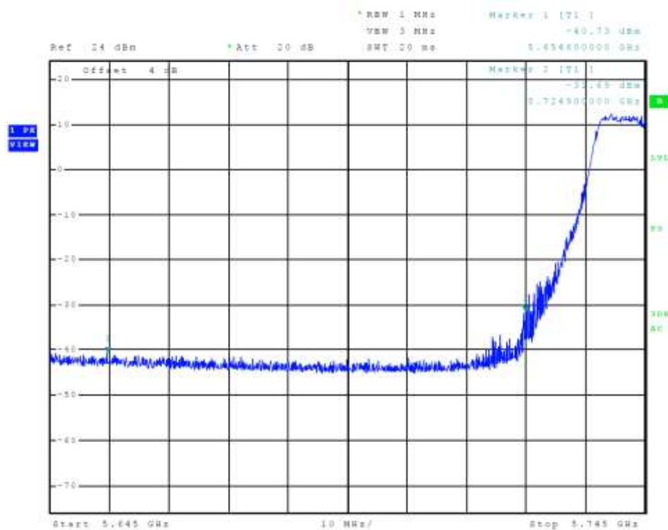
Figure 51 Plot of Transmitter Low Band Edge Chain 1 (5725-5850 MHz Band, 802.11a)
