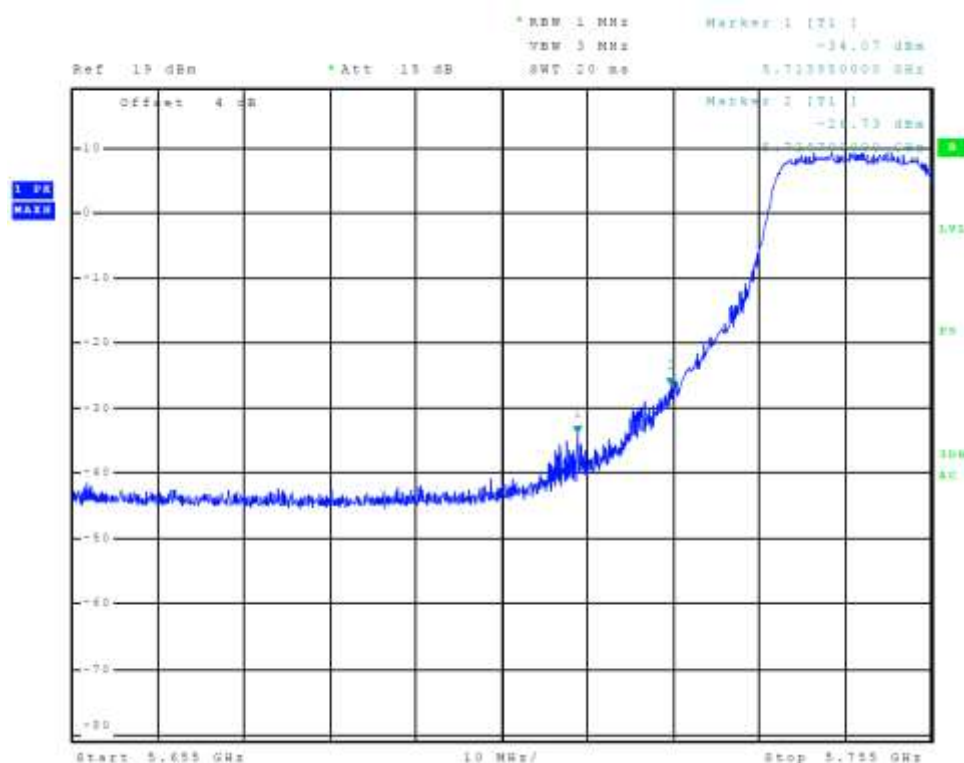
Figure 52 Plot of Transmitter Low Band Edge Chain 1 (5725-5850 MHz Band, 802.11n40)
