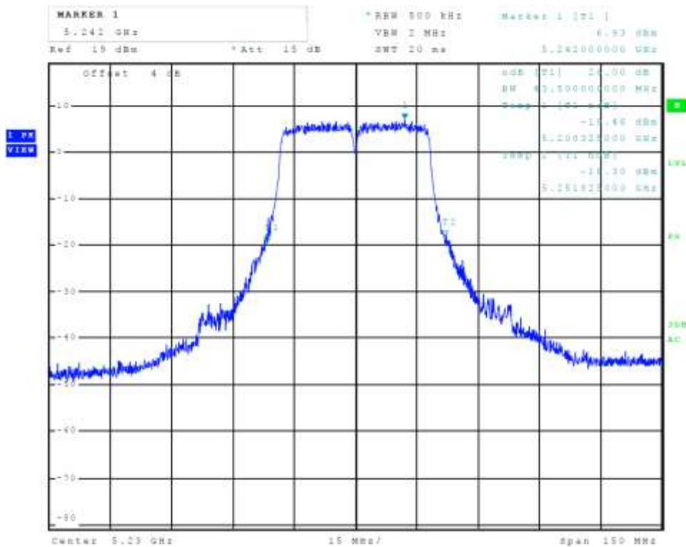
Figure 85 Plot of Transmitter Emissions Chain 2 (5150-5250 MHz Band, 802.11n40, 26 dB OBW)
