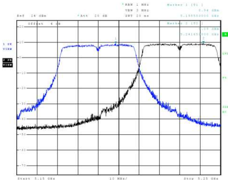
Figure 4 Plot of Transmitter Emissions Chain 0 (Across 5150-5250 MHz Band, 802.11n40)
