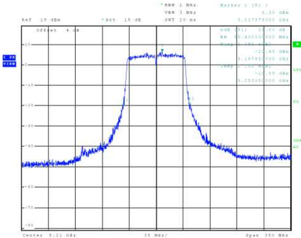
Figure 17 Plot of Transmitter Emissions Chain 0 (5150-5250 MHz Band, 802.11ac, 26 dB OBW)
