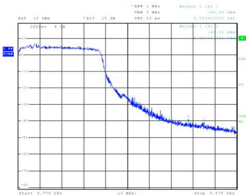
Figure 56 Plot of Transmitter High Band Edge Chain 1 (5725-5850 MHz Band, 802.11ac)
