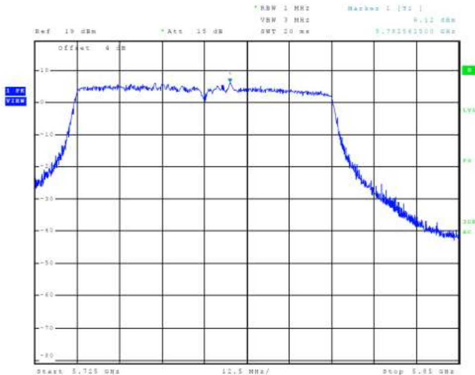
Figure 20 Plot of Transmitter Emissions Chain 0 (Across 5725-5850 MHz Band, 802.11ac)
