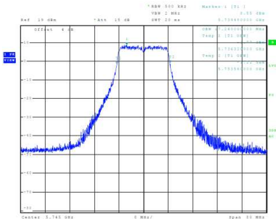
Figure 57 Plot of Transmitter Emissions Chain 1 (5725-5850 MHz Band, 802.11a, 99% OBW)
