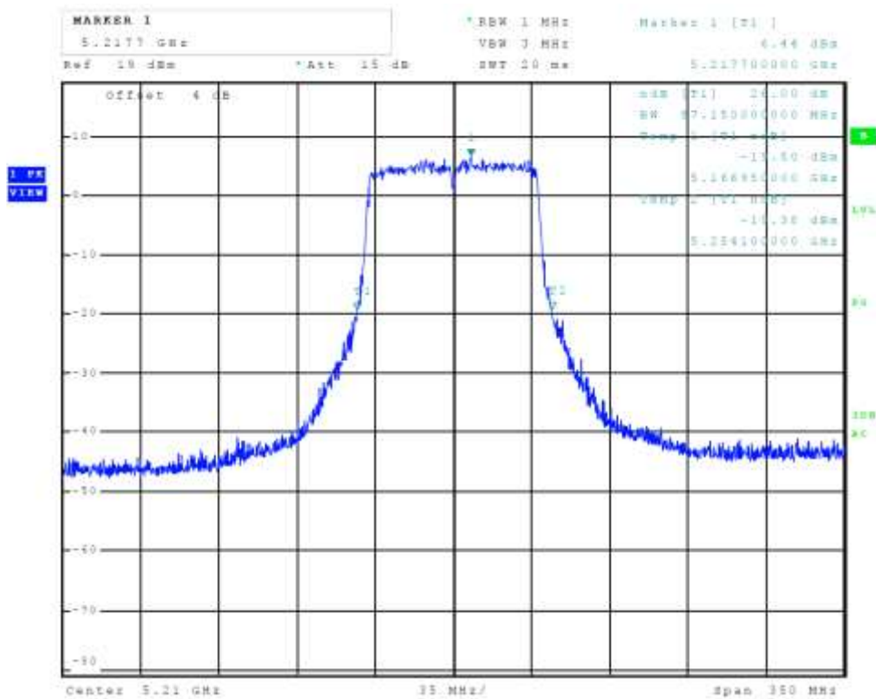
Figure 47 Plot of Transmitter Emissions Chain 1 (5150-5250 MHz Band, 802.11ac, 26 dB OBW)
