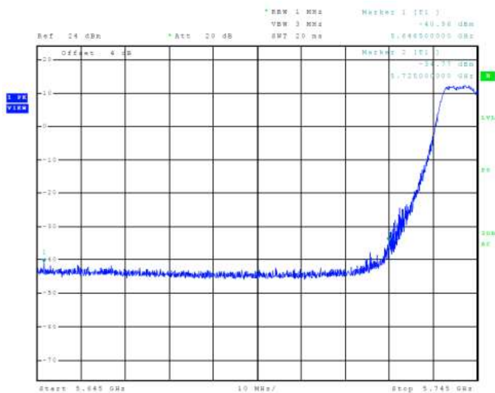
Figure 21 Plot of Transmitter Low Band Edge Chain 0 (5725-5850 MHz Band, 802.11a)
