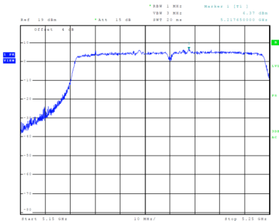
Figure 5 Plot of Transmitter Emissions Chain 0 (Across 5150-5250 MHz Band, 802.11ac)
