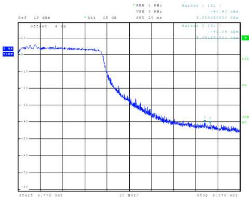
Figure 26 Plot of Transmitter High Band Edge Chain 0 (5725-5850 MHz Band, 802.11ac)
