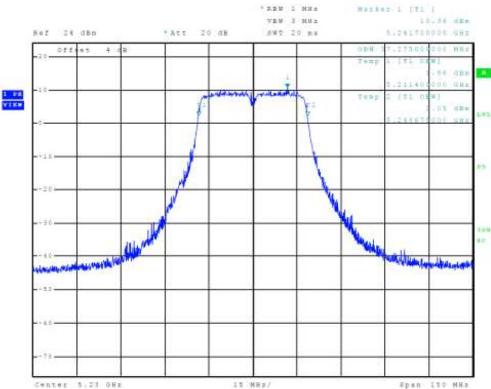
Figure 44 Plot of Transmitter Emissions Chain 1 (5150-5250 MHz Band, 802.11n40, 99% OBW)
