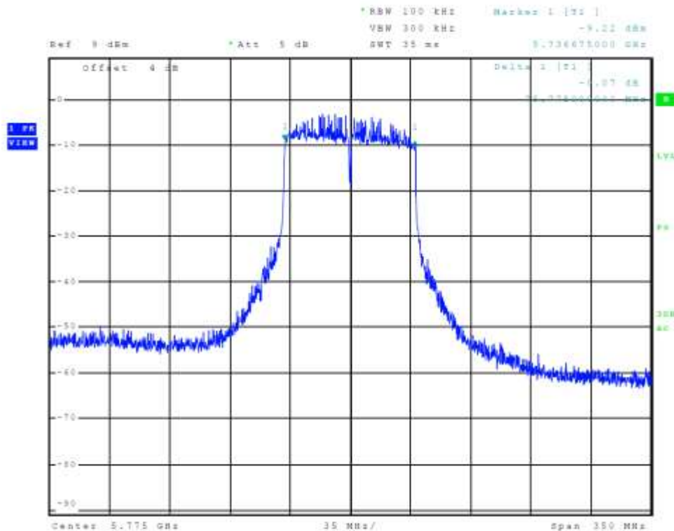
Figure 32 Plot of Transmitter Emissions Chain 0 (5725-5850 MHz Band, 802.11ac, 6-dB OBW)
