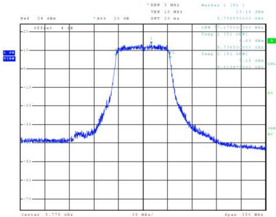
Figure 101 Plot of Transmitter Emissions Chain 2 (5725-5850 MHz Band, 802.11ac, 99% OBW)
