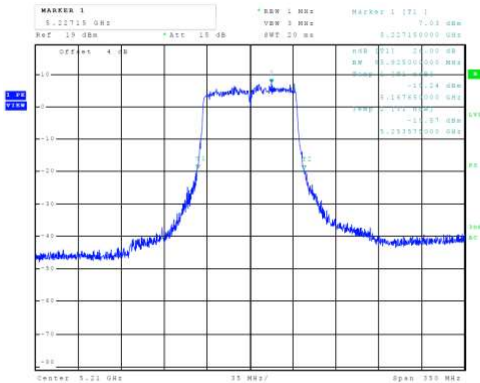
Figure 87 Plot of Transmitter Emissions Chain 2 (5150-5250 MHz Band, 802.11ac, 26 dB OBW)
