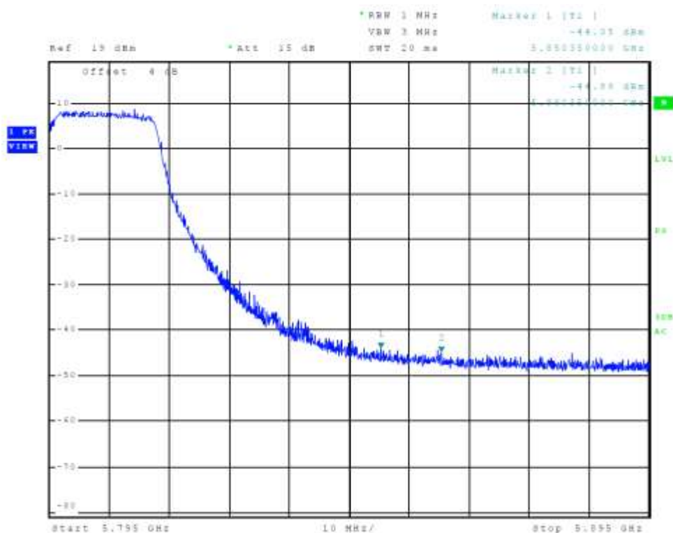
Figure 25 Plot of Transmitter High Band Edge Chain 0 (5725-5850 MHz Band, 802.11n40)
