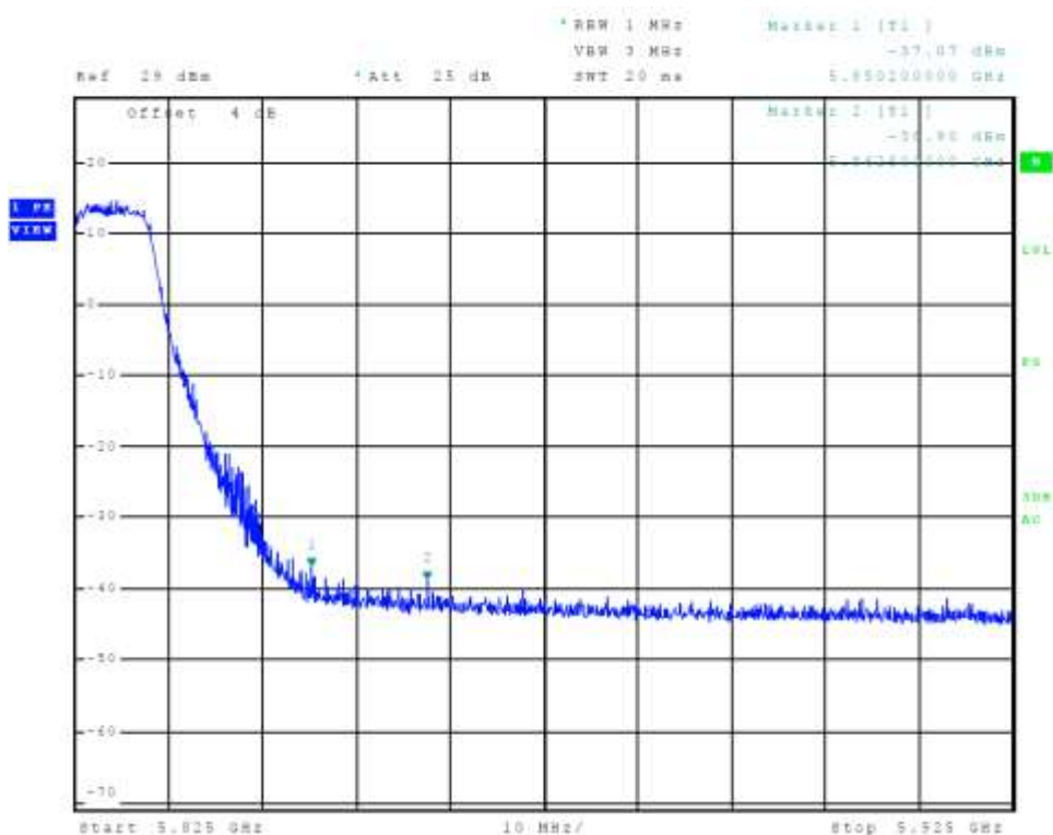
Figure 94 Plot of Transmitter High Band Edge Chain 2 (5725-5850 MHz Band, 802.11a)
