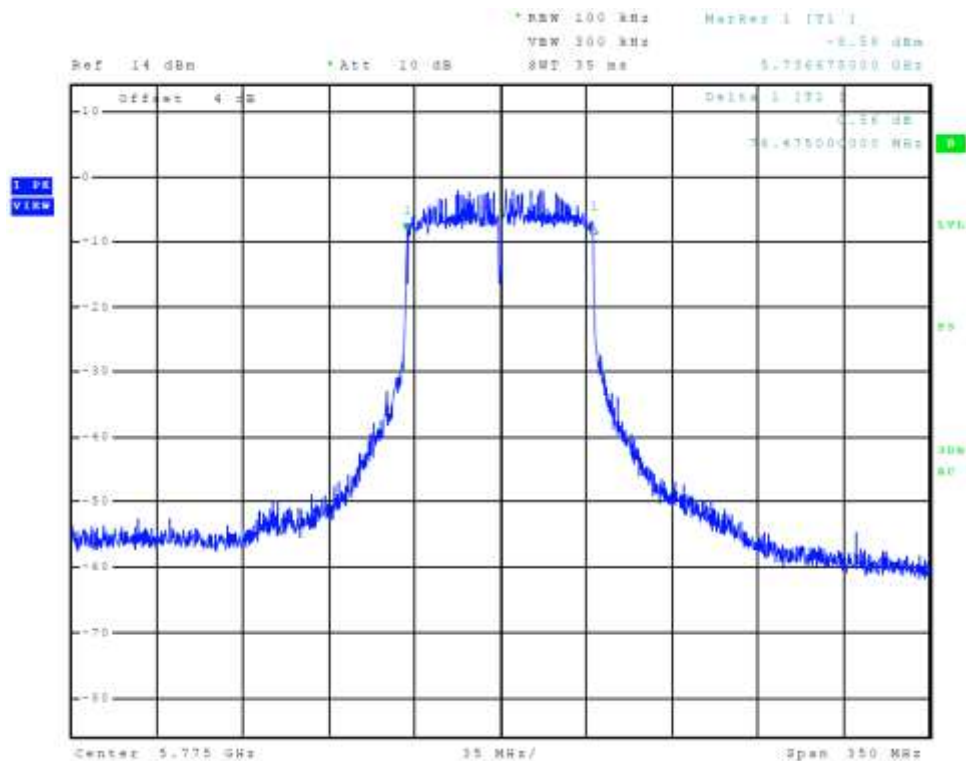
Figure 102 Plot of Transmitter Emissions Chain 2 (5725-5850 MHz Band, 802.11ac, 6-dB OBW)
