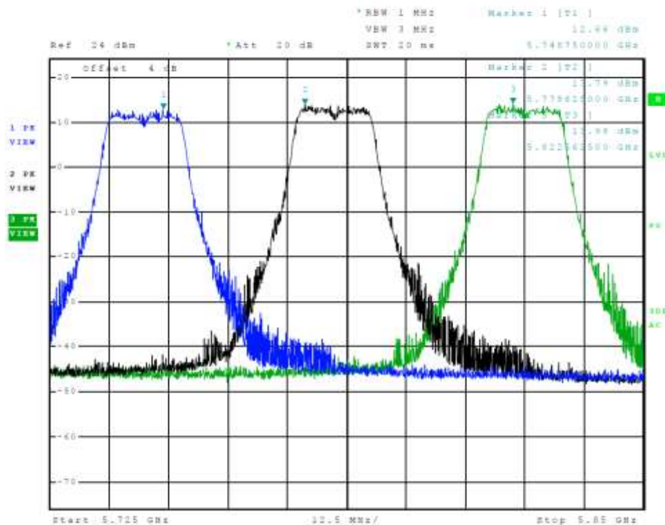
Figure 48 Plot of Transmitter Emissions Chain 1 (Across 5725-5850 MHz Band, 802.11a)
