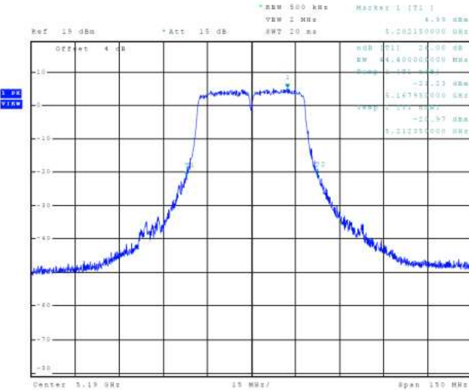
Figure 15 Plot of Transmitter Emissions Chain 0 (5150-5250 MHz Band, 802.11n40, 26 dB OBW)
