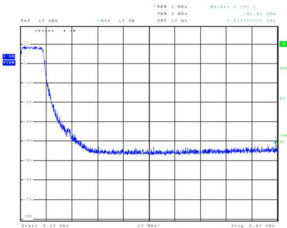
Figure 10 Plot of Transmitter High Band Edge Chain 0 (5150-5250 MHz Band, 802.11n40)
