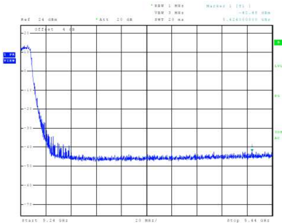
Figure 39 Plot of Transmitter High Band Edge Chain 1 (5150-5250 MHz Band, 802.11a)
