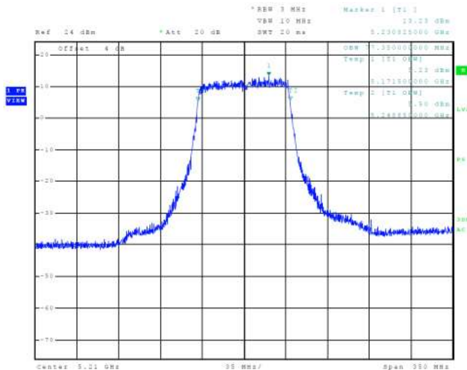
Figure 86 Plot of Transmitter Emissions Chain 2 (5150-5250 MHz Band, 802.11ac, 99% OBW)
