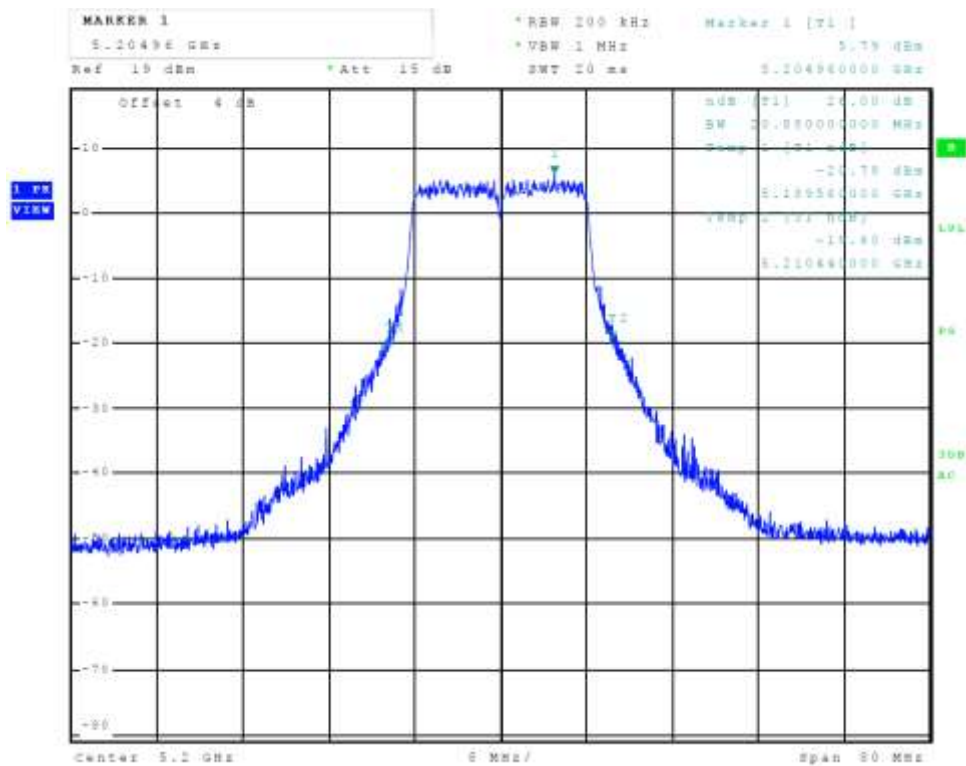
Figure 83 Plot of Transmitter Emissions Chain 2 (5150-5250 MHz Band, 802.11a, 26 dB OBW)
