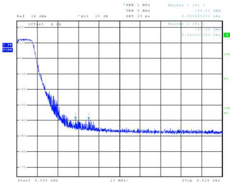
Figure 24 Plot of Transmitter High Band Edge Chain 0 (5725-5850 MHz Band, 802.11a)
