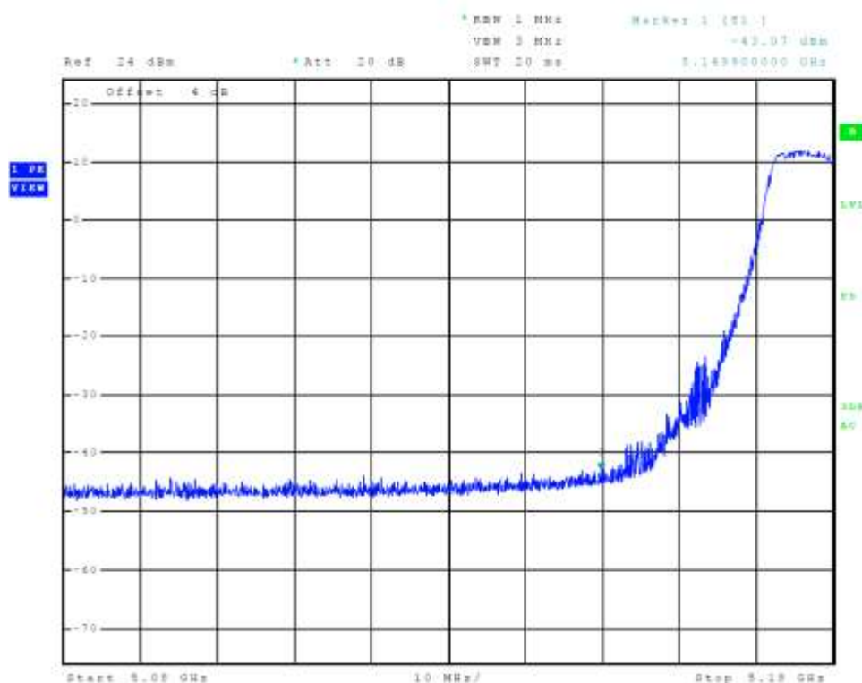
Figure 6 Plot of Transmitter Low Band Edge Chain 0 (5150-5250 MHz Band, 802.11a)
