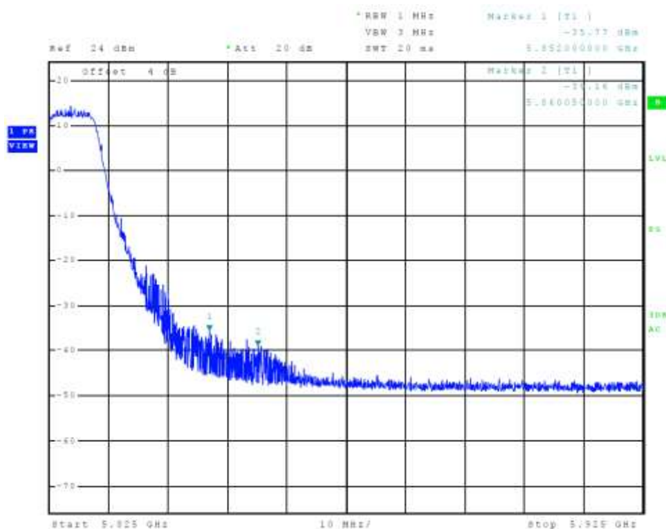
Figure 54 Plot of Transmitter High Band Edge Chain 1 (5725-5850 MHz Band, 802.11a)
