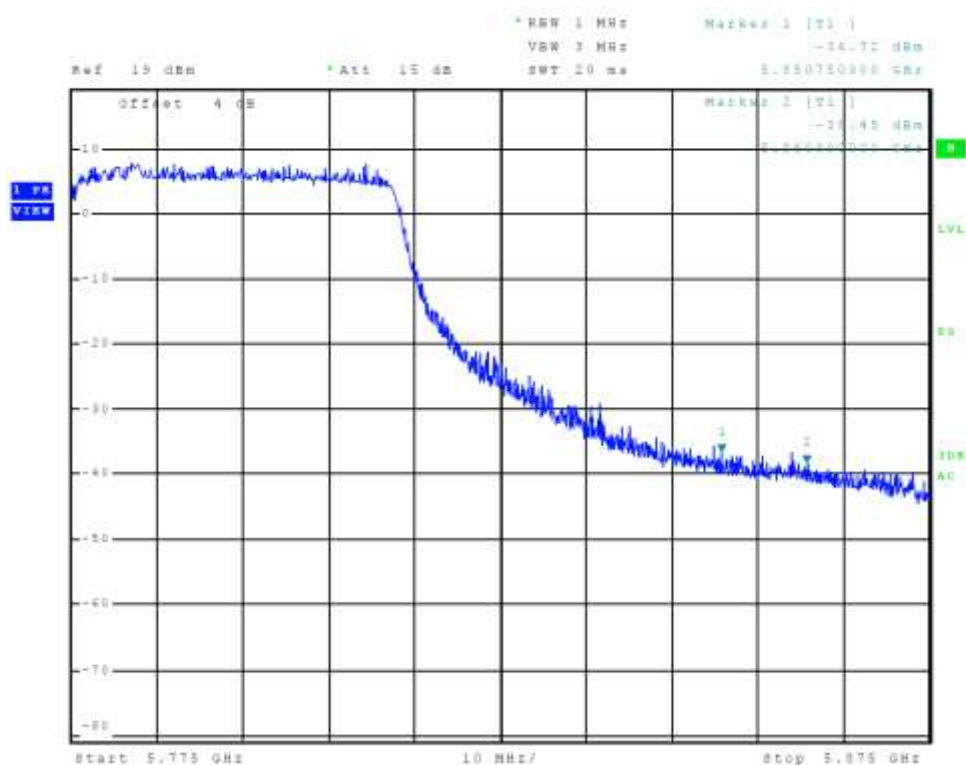
Figure 96 Plot of Transmitter High Band Edge Chain 2 (5725-5850 MHz Band, 802.11ac)
