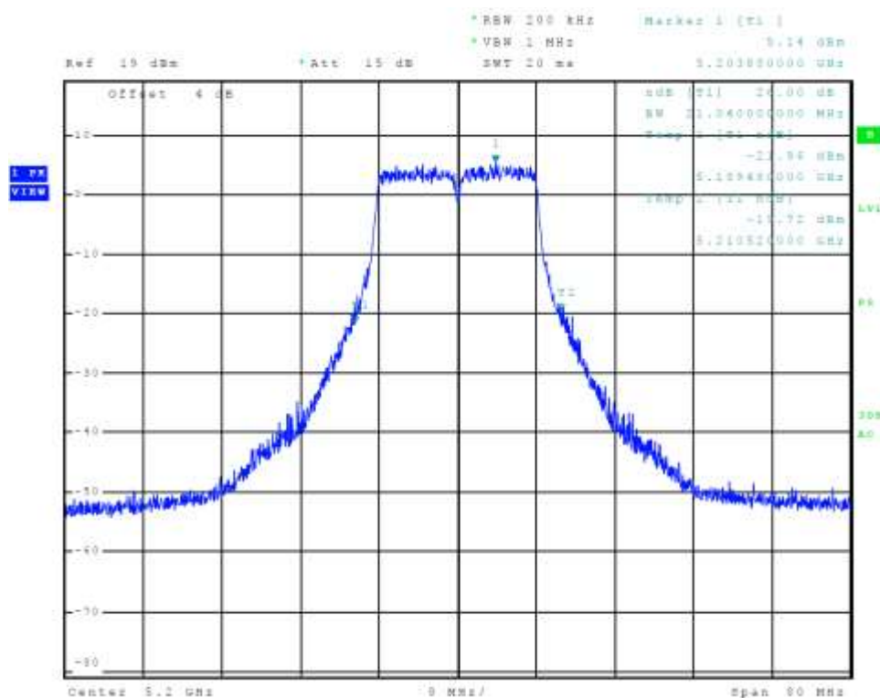
Figure 13 Plot of Transmitter Emissions Chain 0 (5150-5250 MHz Band, 802.11a, 26 dB OBW)
