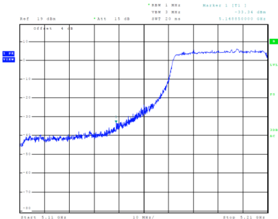
Figure 8 Plot of Transmitter Low Band Edge Chain 0 (5150-5250 MHz Band, 802.11ac)
