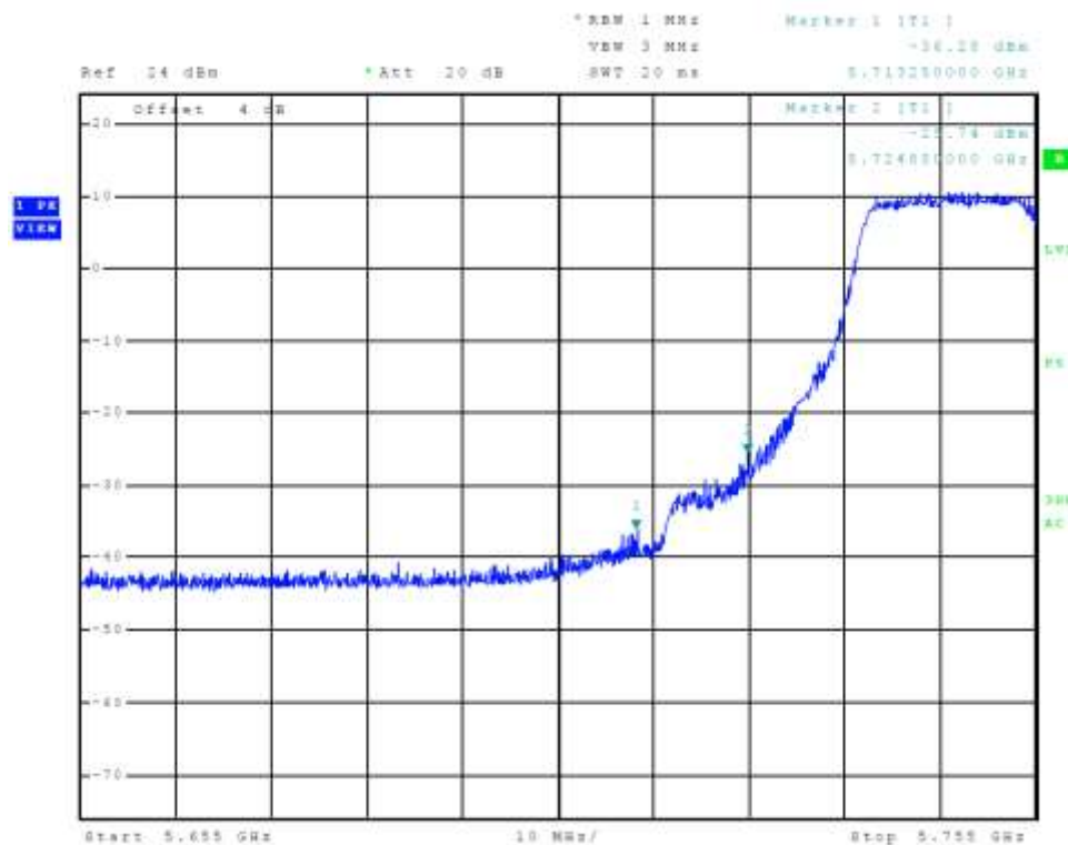
Figure 92 Plot of Transmitter Low Band Edge Chain 2 (5725-5850 MHz Band, 802.11n40)
