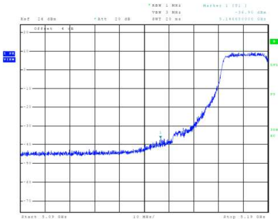
Figure 77 Plot of Transmitter Low Band Edge Chain 2 (5150-5250 MHz Band, 802.11n40)
