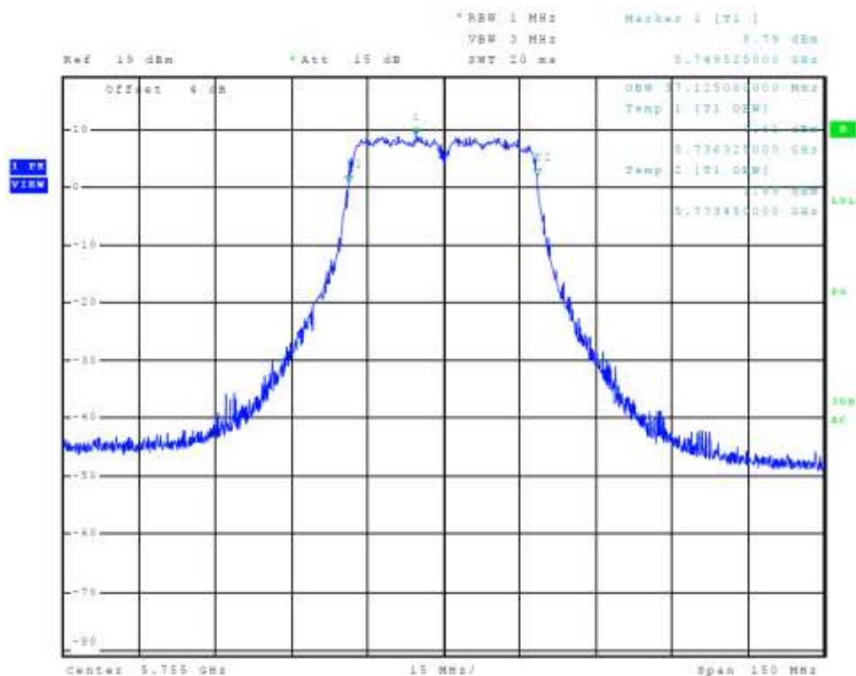
Figure 59 Plot of Transmitter Emissions Chain 1 (5725-5850 MHz Band, 802.11n40, 99% OBW)
