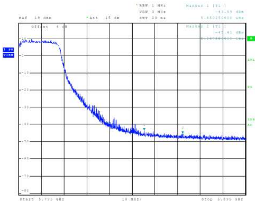
Figure 55 Plot of Transmitter High Band Edge Chain 1 (5725-5850 MHz Band, 802.11n40)
