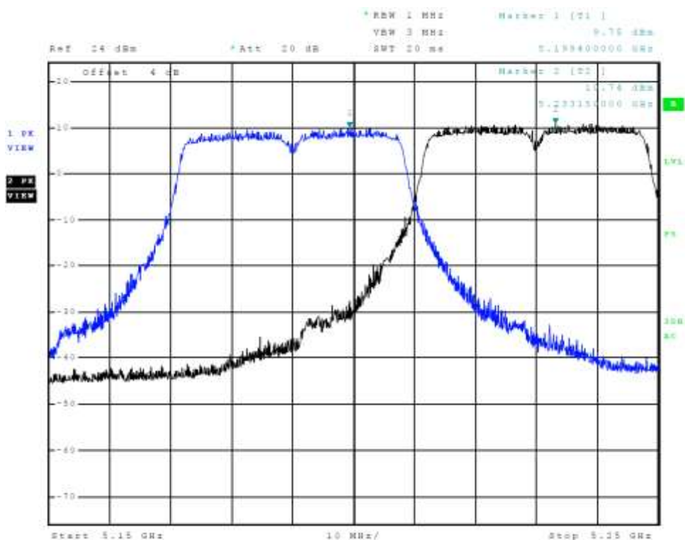
Figure 74 Plot of Transmitter Emissions Chain 2 (Across 5150-5250 MHz Band, 802.11n40)
