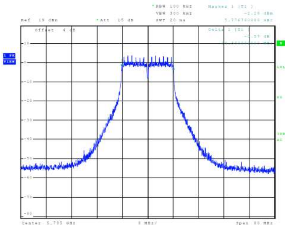
Figure 28 Plot of Transmitter Emissions Chain 0 (5725-5850 MHz Band, 802.11a, 6-dB OBW)
