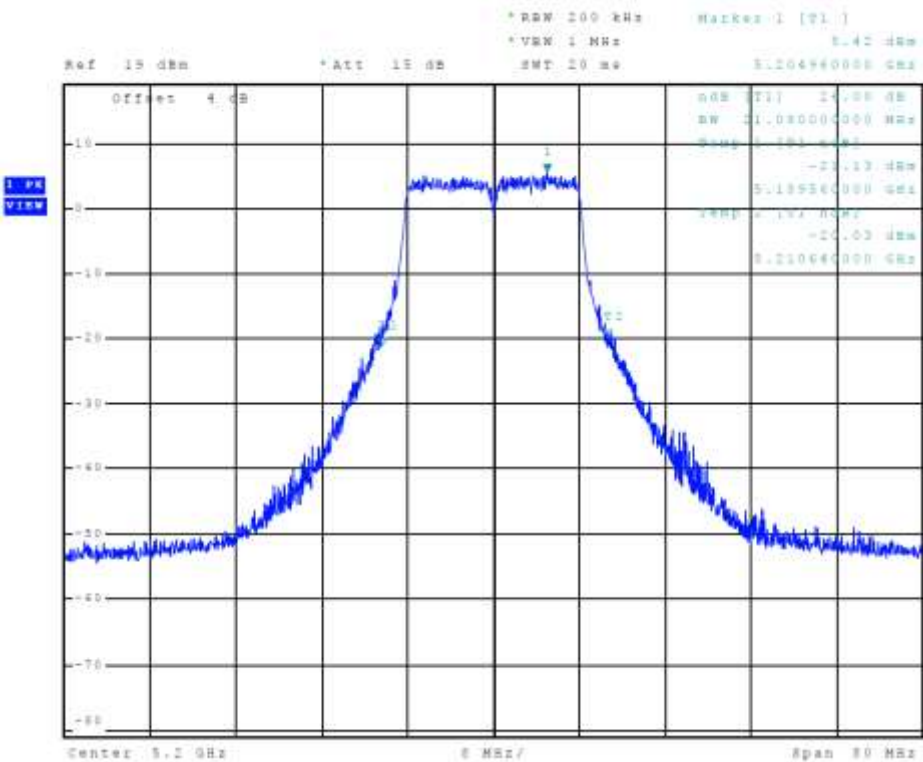
Figure 43 Plot of Transmitter Emissions Chain 1 (5150-5250 MHz Band, 802.11a, 26 dB OBW)
