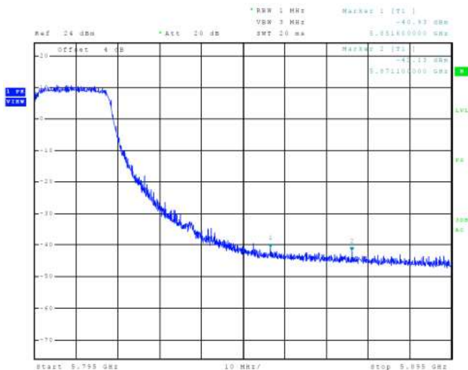
Figure 95 Plot of Transmitter High Band Edge Chain 2 (5725-5850 MHz Band, 802.11n40)
