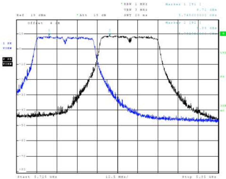
Figure 19 Plot of Transmitter Emissions Chain 0 (Across 5725-5850 MHz Band, 802.11n40)
