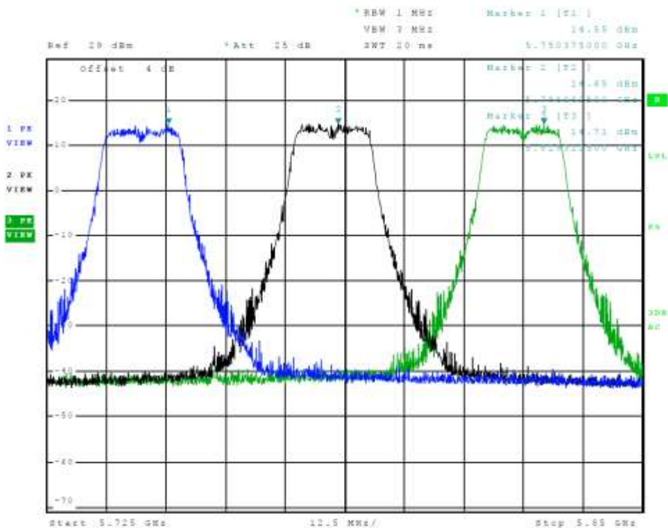
Figure 88 Plot of Transmitter Emissions Chain 2 (Across 5725-5850 MHz Band, 802.11a)
