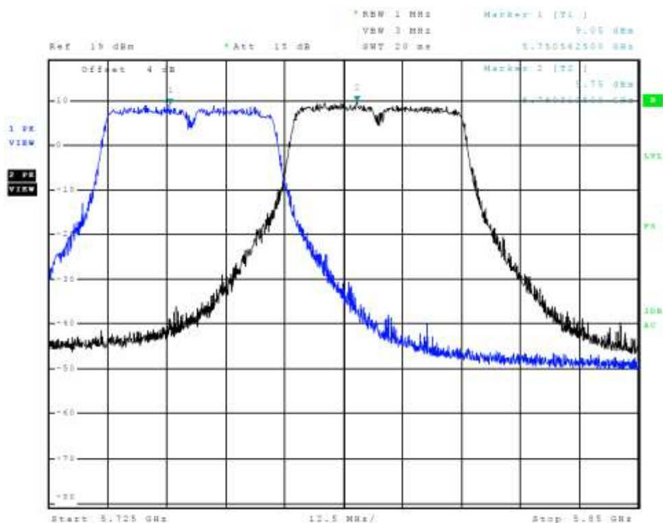
Figure 49 Plot of Transmitter Emissions Chain 1 (Across 5725-5850 MHz Band, 802.11n40)
