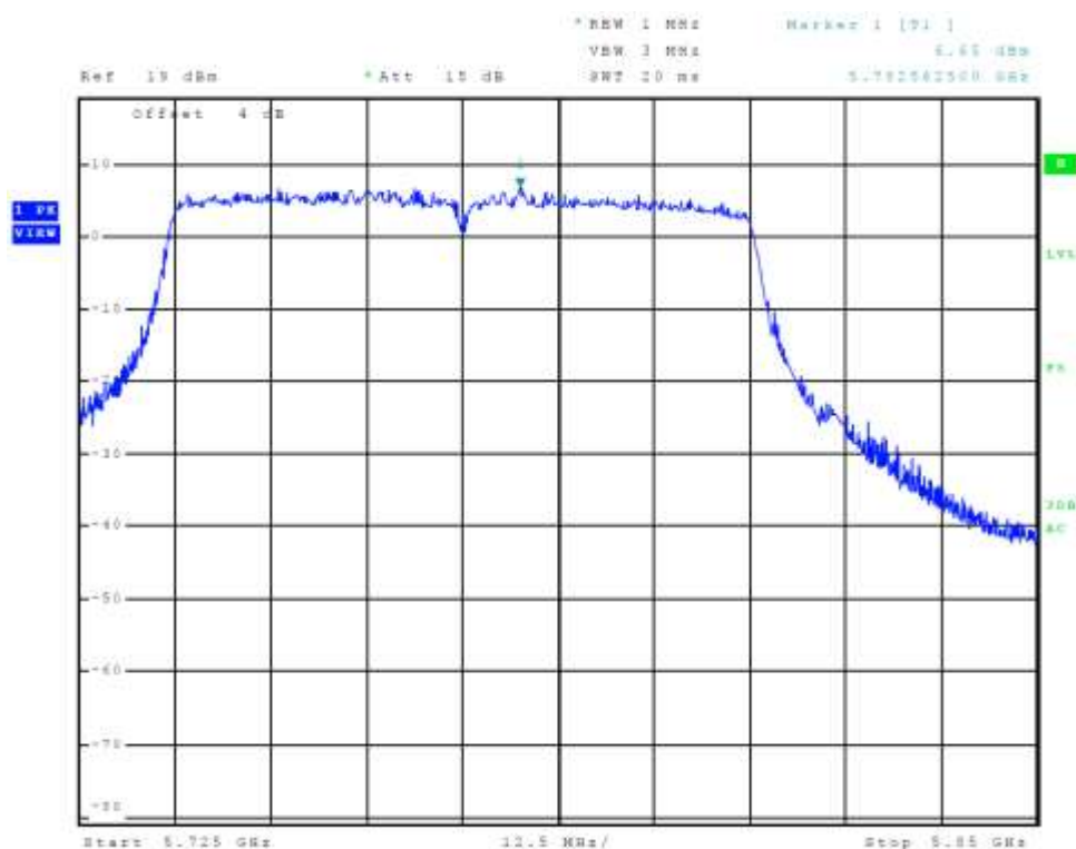
Figure 50 Plot of Transmitter Emissions Chain 1 (Across 5725-5850 MHz Band, 802.11ac)
