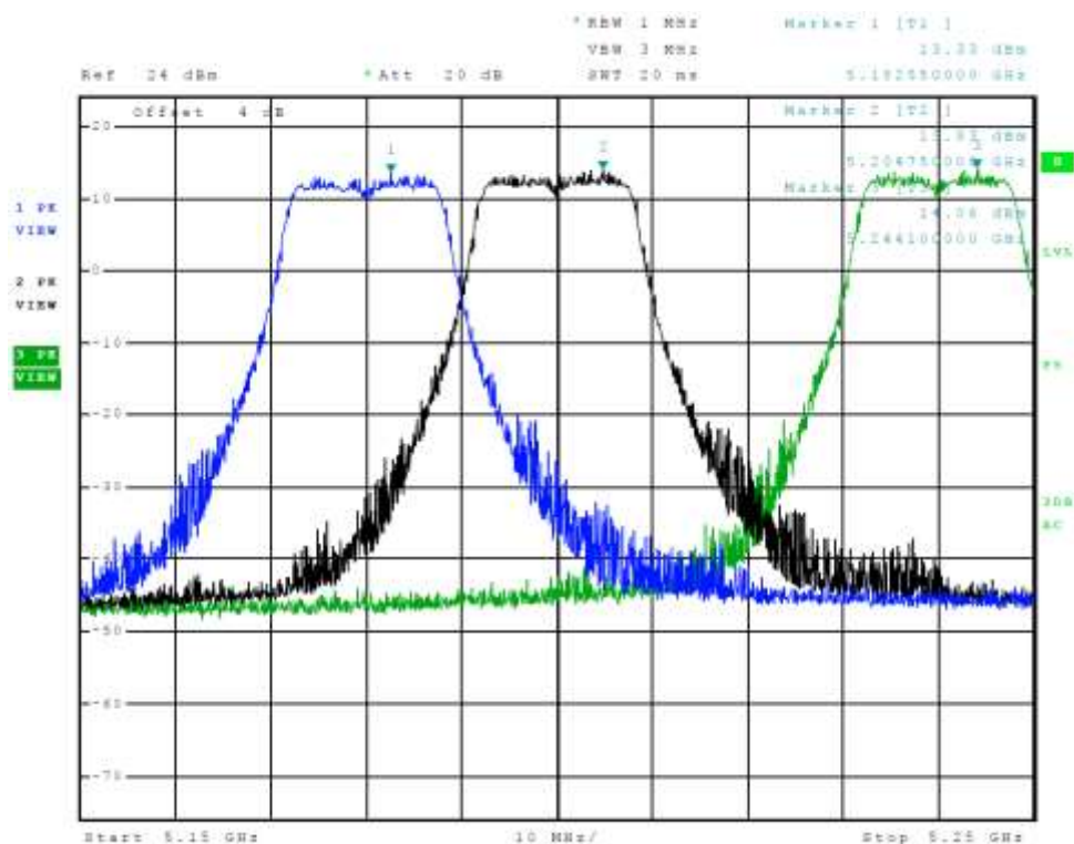
Figure 33 Plot of Transmitter Emissions Chain 1 (Across 5150-5250 MHz Band, 802.11a)
