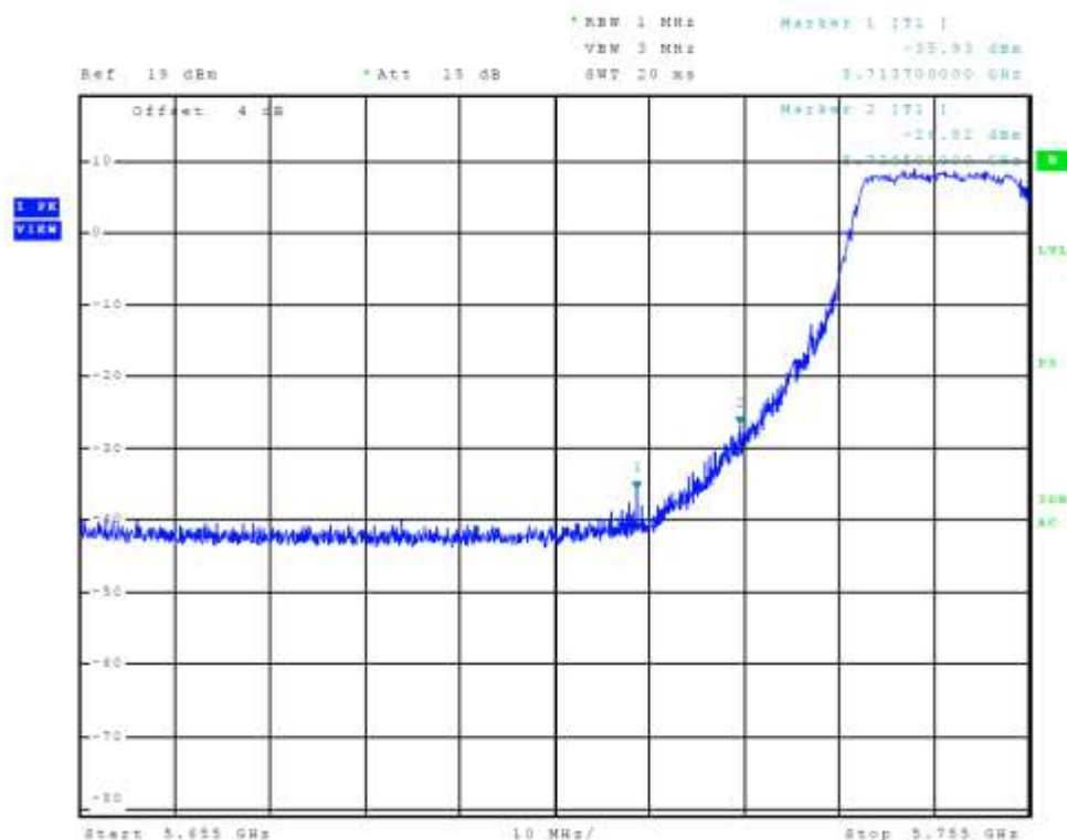
Figure 22 Plot of Transmitter Low Band Edge Chain 0 (5725-5850 MHz Band, 802.11n40)
