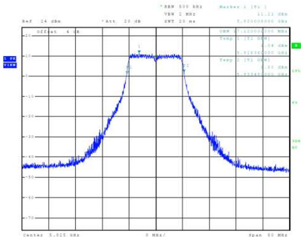
Figure 97 Plot of Transmitter Emissions Chain 2 (5725-5850 MHz Band, 802.11a, 99% OBW)
