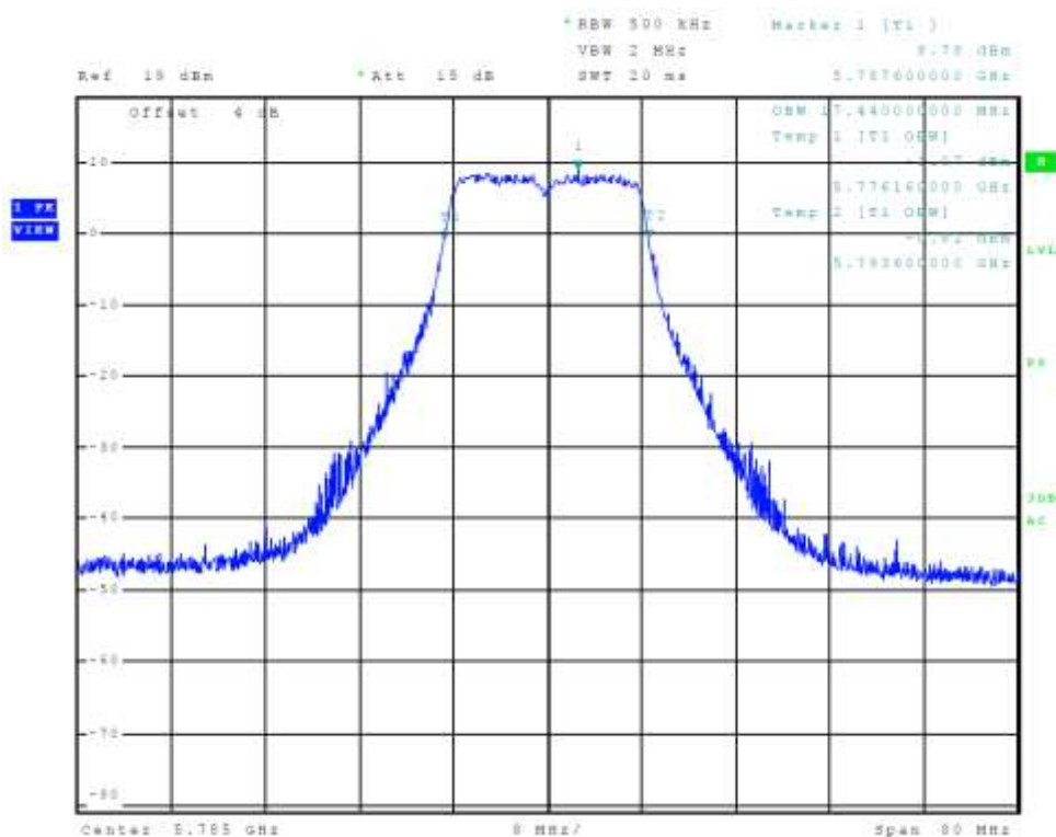
Figure 27 Plot of Transmitter Emissions Chain 0 (5725-5850 MHz Band, 802.11a, 99% OBW)
