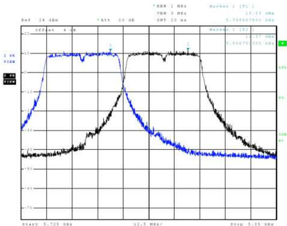
Figure 89 Plot of Transmitter Emissions Chain 2 (Across 5725-5850 MHz Band, 802.11n40)
