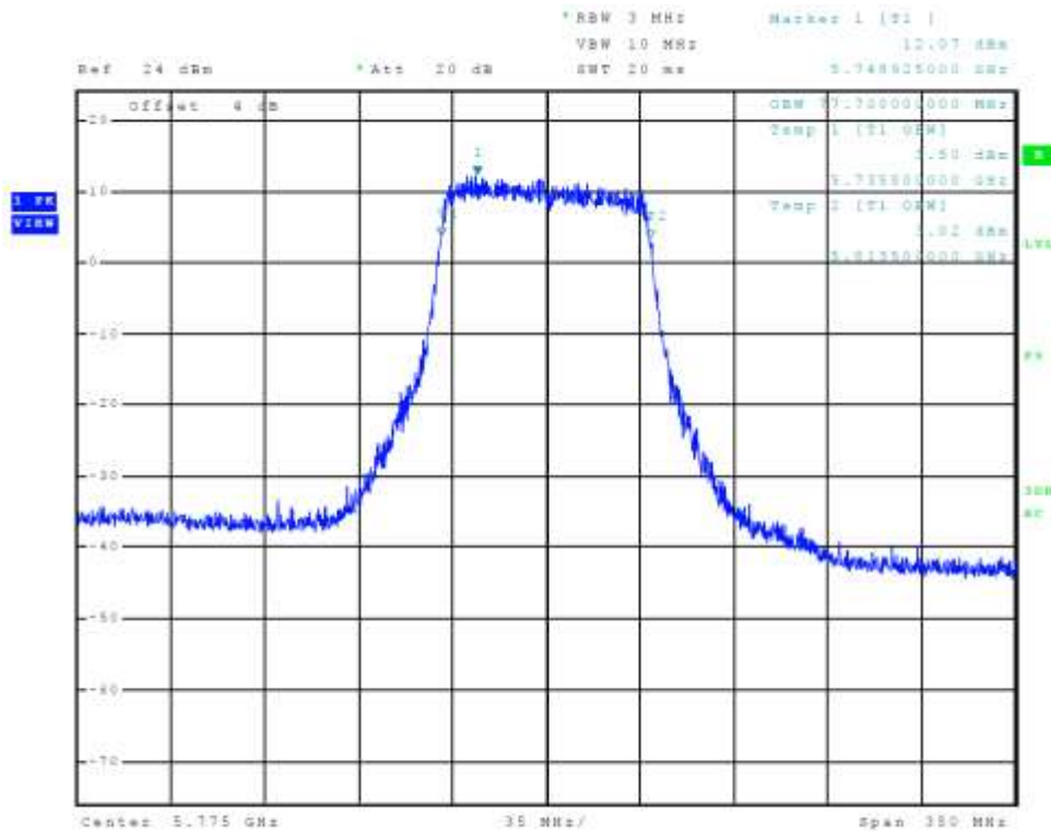
Figure 31 Plot of Transmitter Emissions Chain 0 (5725-5850 MHz Band, 802.11ac, 99% OBW)
