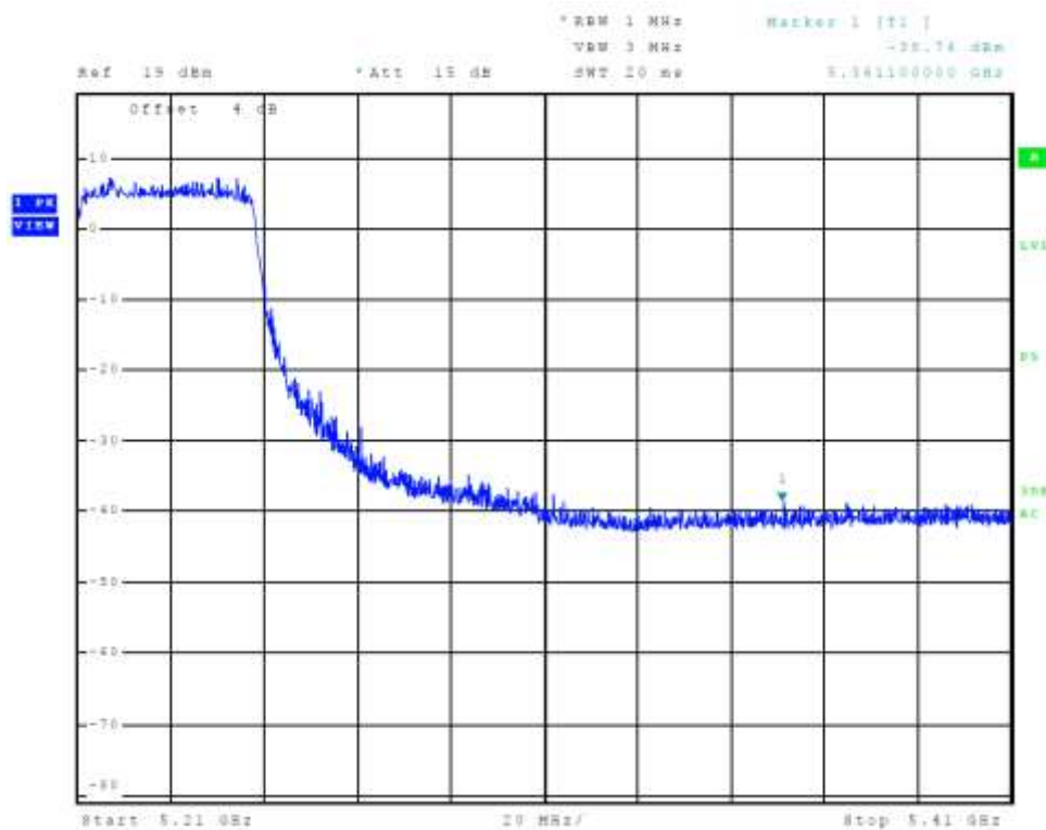
Figure 81 Plot of Transmitter High Band Edge Chain 2 (5150-5250 MHz Band, 802.11ac)
