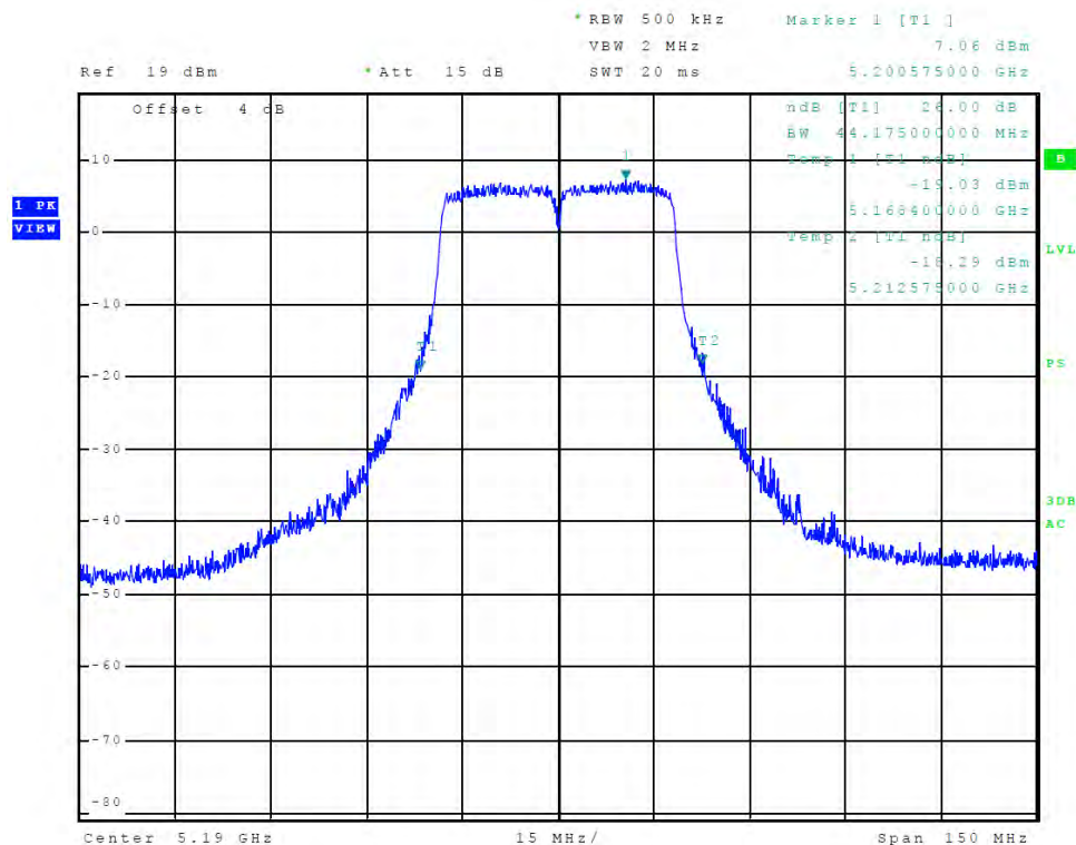
Figure 40 Plot of Transmitter Emissions (Chain 1, 5150-5250 MHz Band, 802.11n40, 26 dB OBW)
