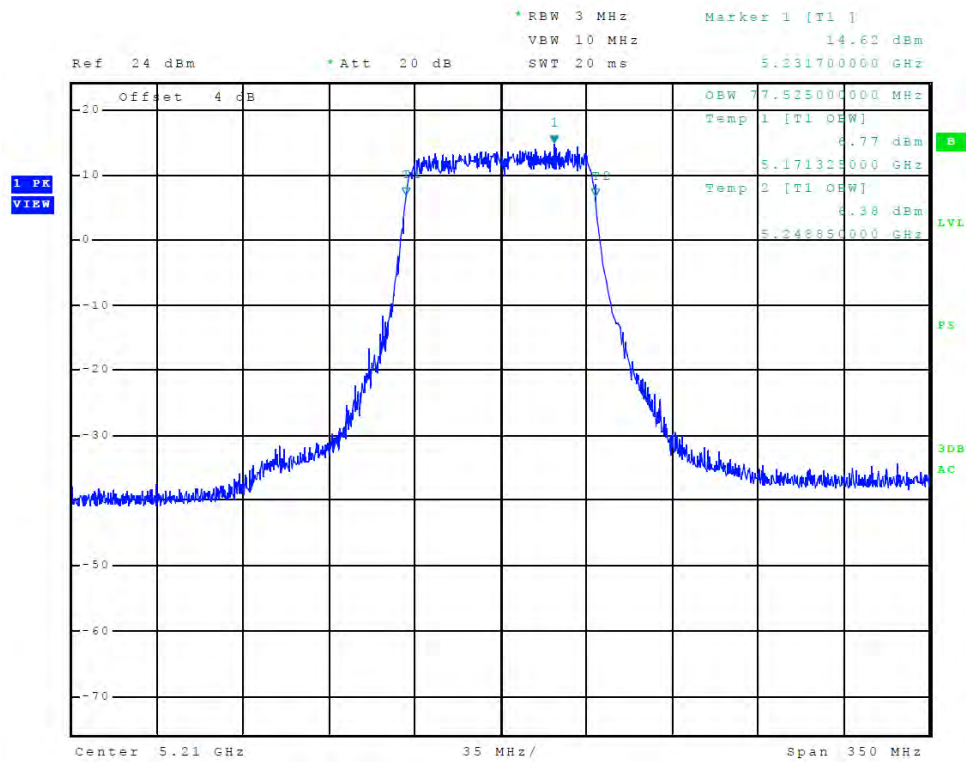
Figure 43 Plot of Transmitter Emissions (Chain 1, 5150-5250 MHz Band, 802.11ac, 99% OBW)
