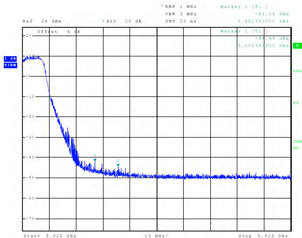
Figure 686 Plot of Transmitter High Band Edge (Chain 2, 5725-5850 MHz Band, 802.11a)
