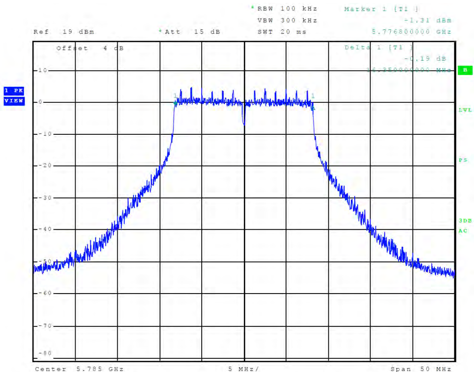
Figure 78 Plot of Transmitter Emissions (Chain 0, 5725-5850 MHz Band, 802.11a, 6-dB OBW)
