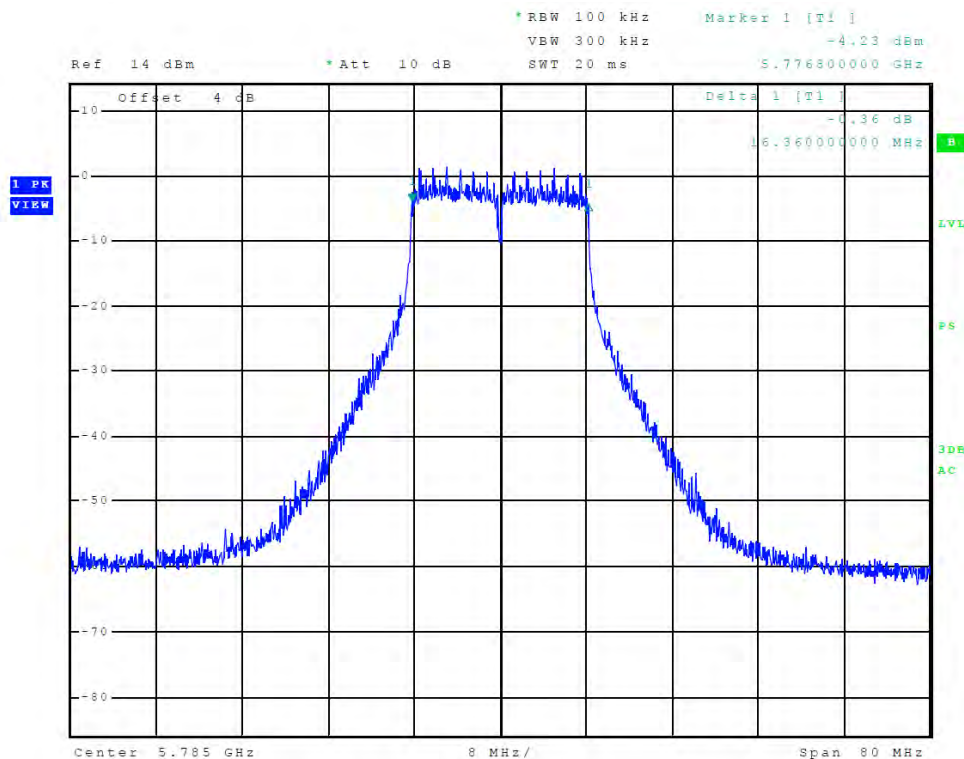
Figure 80 Plot of Transmitter Emissions (Chain 2, 5725-5850 MHz Band, 802.11a, 6-dB OBW)
