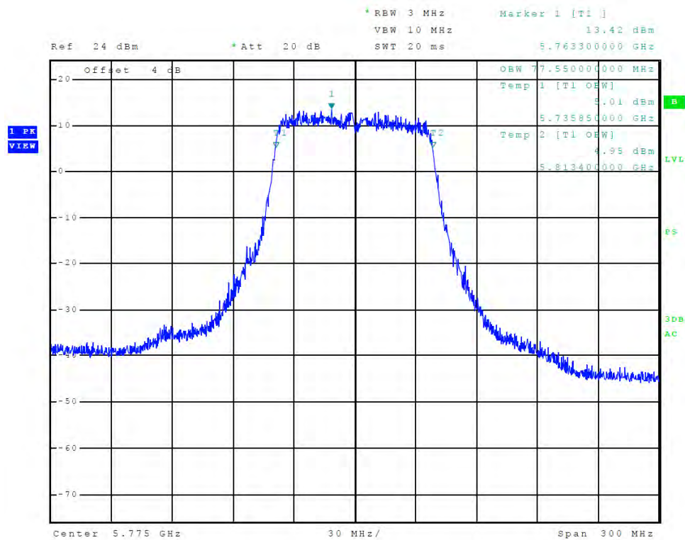
Figure 87 Plot of Transmitter Emissions (Chain 0, 5725-5850 MHz Band, 802.11ac, 99% OBW)
