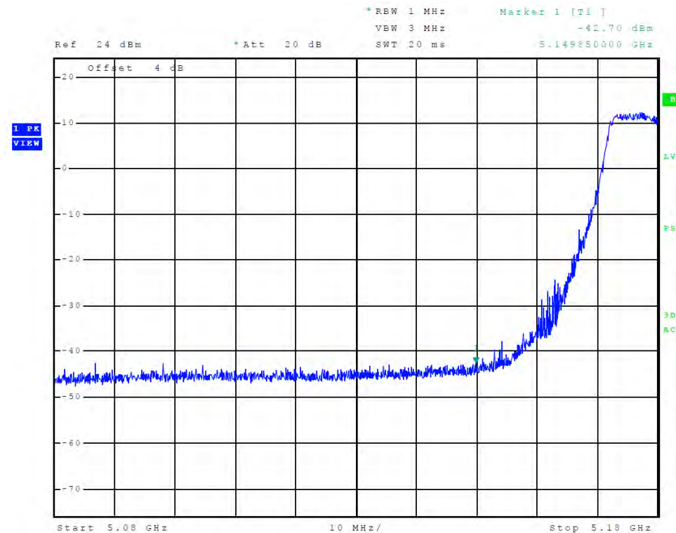
Figure 14 Plot of Transmitter Low Band Edge (Chain 2, 5150-5250 MHz Band, 802.11a)
