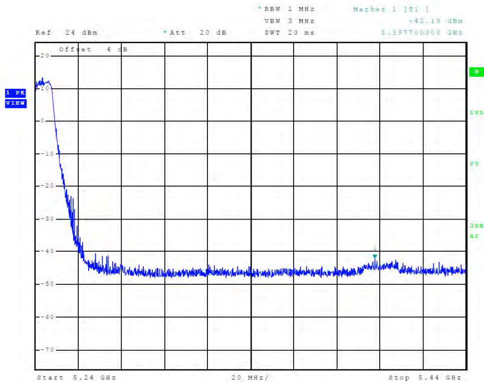
Figure 23 Plot of Transmitter High Band Edge (Chain 2, 5150-5250 MHz Band, 802.11a)
