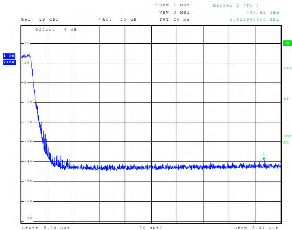
Figure 22 Plot of Transmitter High Band Edge (Chain 1, 5150-5250 MHz Band, 802.11a)
