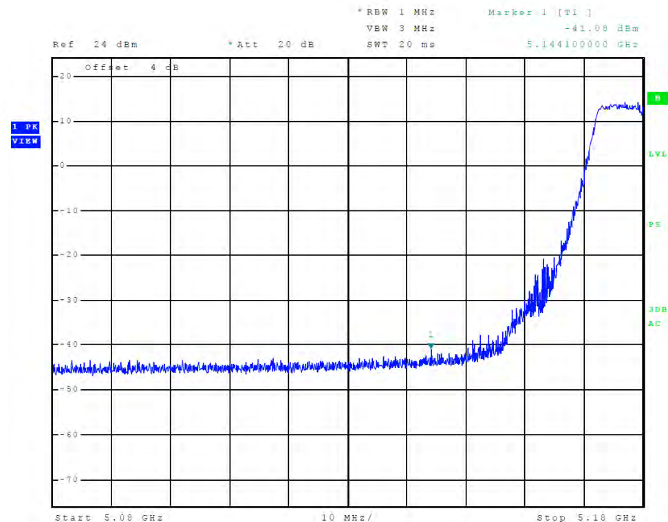
Figure 12 Plot of Transmitter Low Band Edge (Chain 0, 5150-5250 MHz Band, 802.11a)
