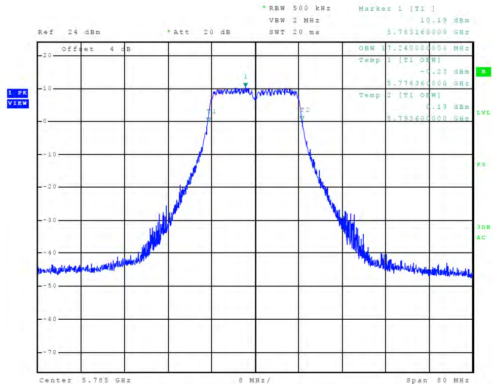
Figure 76 Plot of Transmitter Emissions (Chain 1, 5725-5850 MHz Band, 802.11a, 99% OBW)
