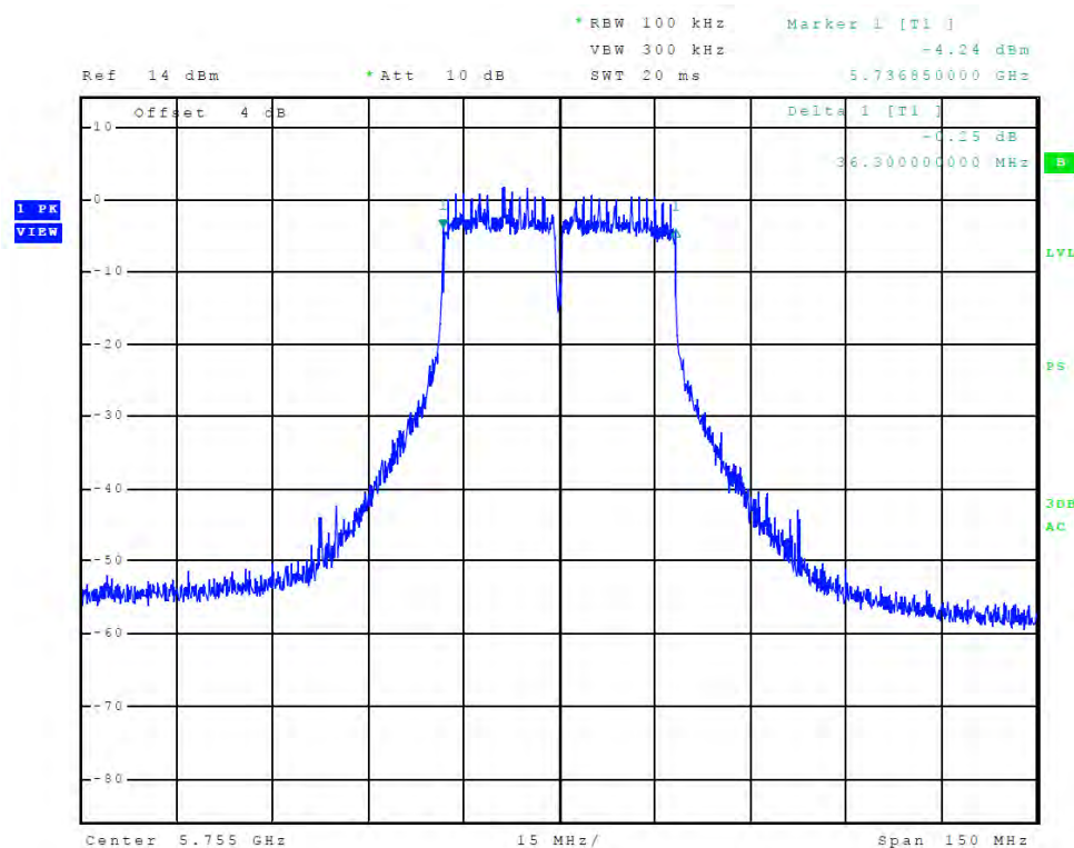
Figure 86 Plot of Transmitter Emissions (Chain 2, 5725-5850 MHz Band, 802.11n40, 6-dB OBW)
