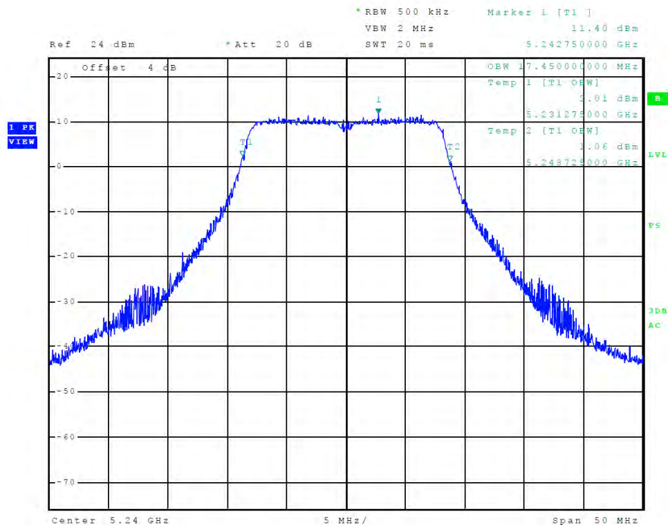
Figure 30 Plot of Transmitter Emissions (Chain 0, 5150-5250 MHz Band, 802.11a, 99% OBW)
