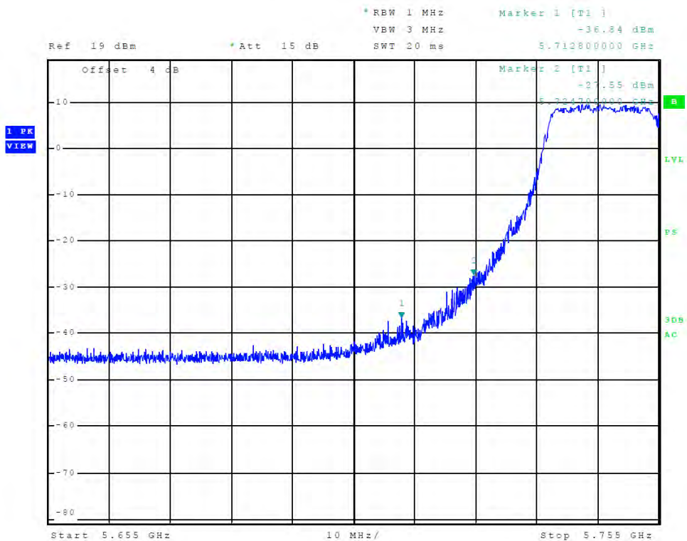
Figure 60 Plot of Transmitter Low Band Edge (Chain 0, 5725-5850 MHz Band, 802.11n40)
