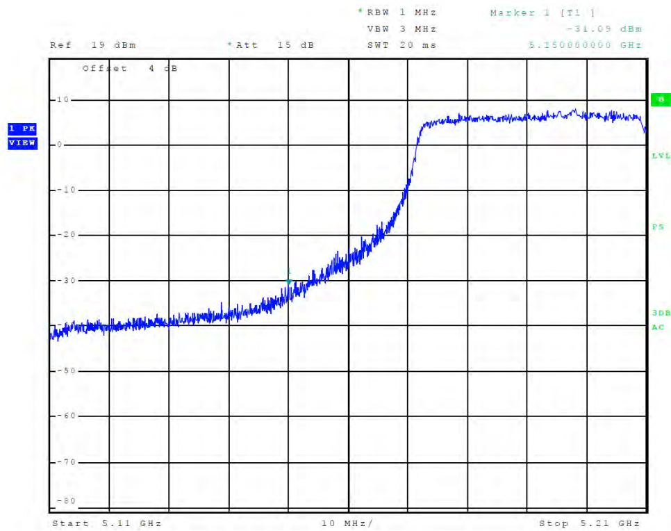
Figure 19 Plot of Transmitter Low Band Edge (Chain 1, 5150-5250 MHz Band, 802.11ac)
