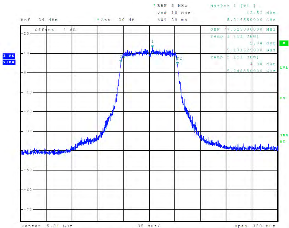
Figure 44 Plot of Transmitter Emissions (Chain 2, 5150-5250 MHz Band, 802.11ac, 99% OBW)
