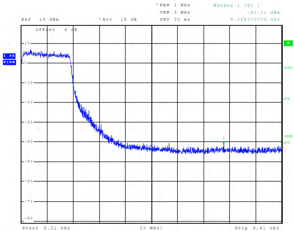
Figure 29 Plot of Transmitter High Band Edge (Chain 2, 5150-5250 MHz Band, 802.11ac)
