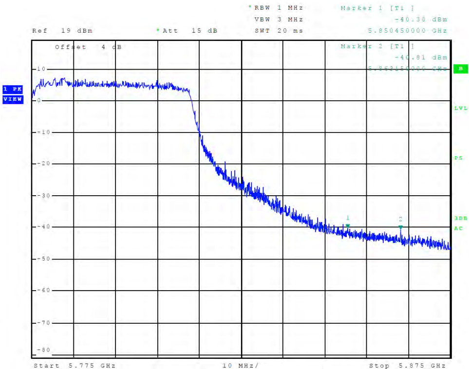
Figure 74 Plot of Transmitter High Band Edge (Chain 2, 5725-5850 MHz Band, 802.11ac)
