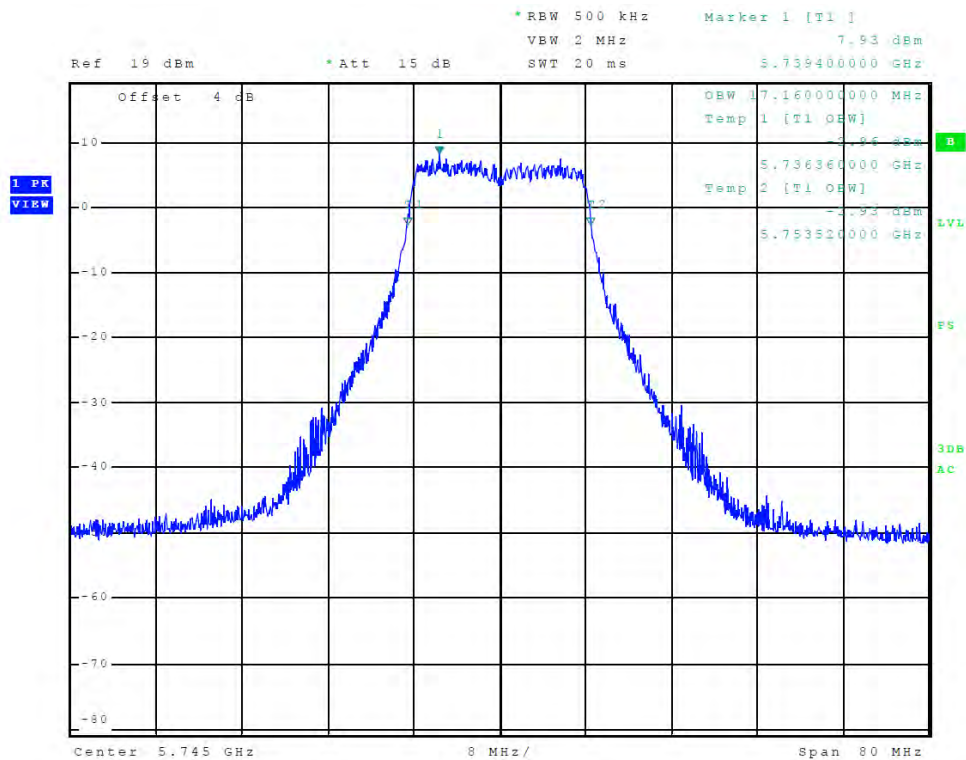
Figure 77 Plot of Transmitter Emissions (Chain 2, 5725-5850 MHz Band, 802.11a, 99% OBW)
