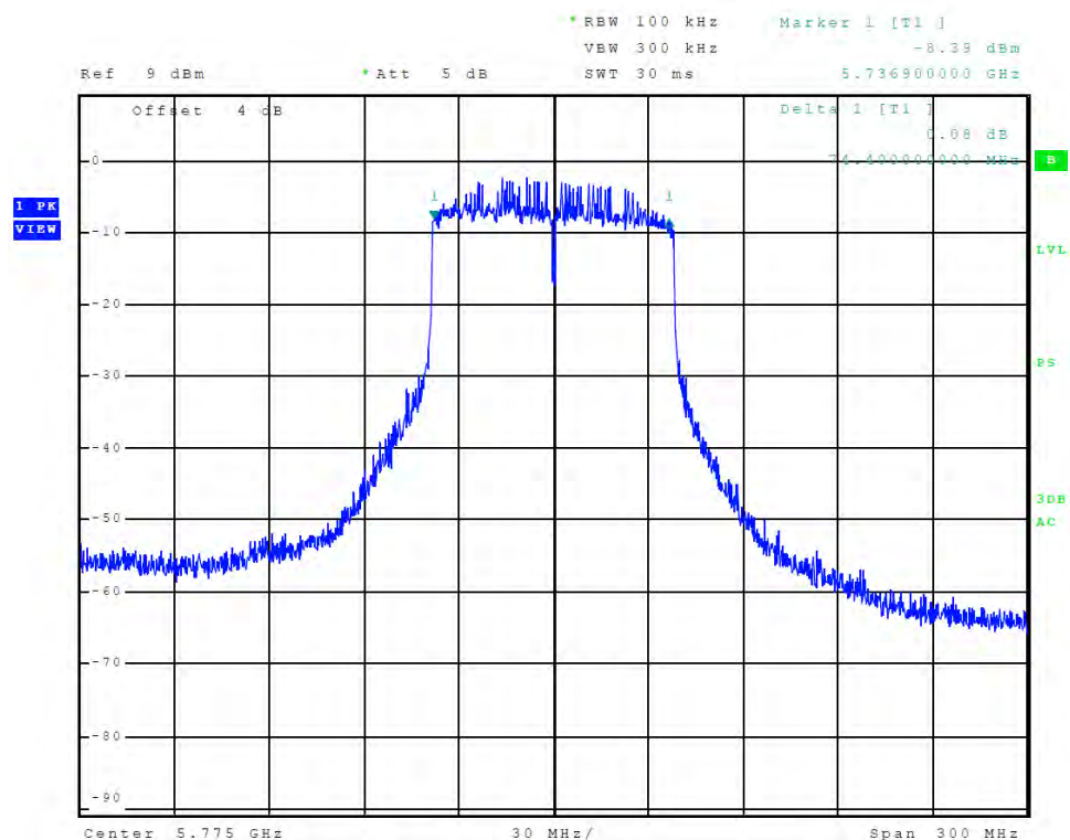
Figure 90 Plot of Transmitter Emissions (Chain 0, 5725-5850 MHz Band, 802.11ac, 6-dB OBW)
