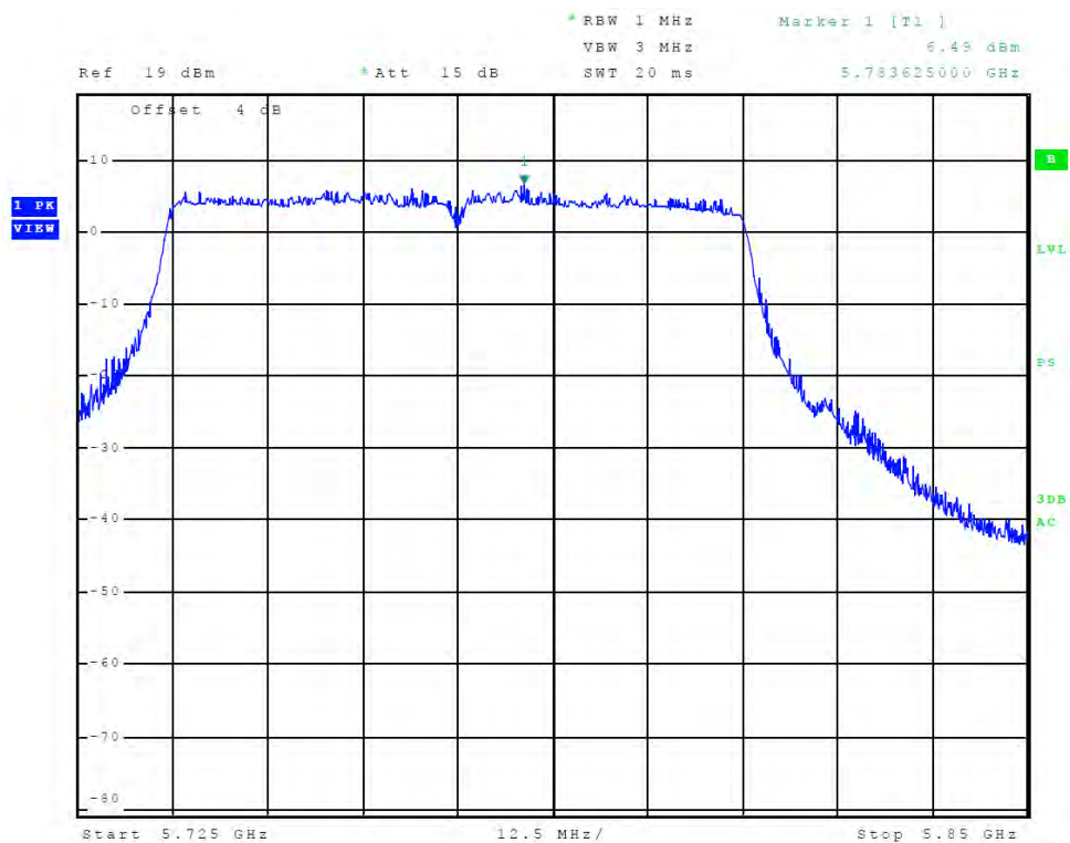
Figure 55 Plot of Transmitter Emissions (Chain 1, Across 5725-5850 MHz Band, 802.11ac)
