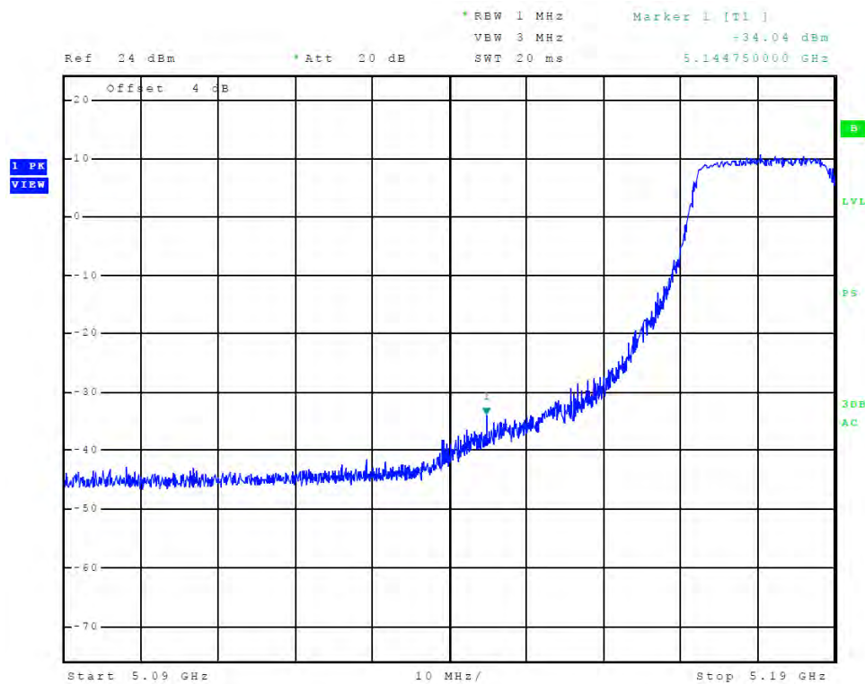
Figure 15 Plot of Transmitter Low Band Edge (Chain 0, 5150-5250 MHz Band, 802.11n40)
