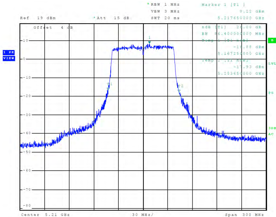
Figure 45 Plot of Transmitter Emissions (Chain 0, 5150-5250 MHz Band, 802.11ac, 26 dB OBW)
