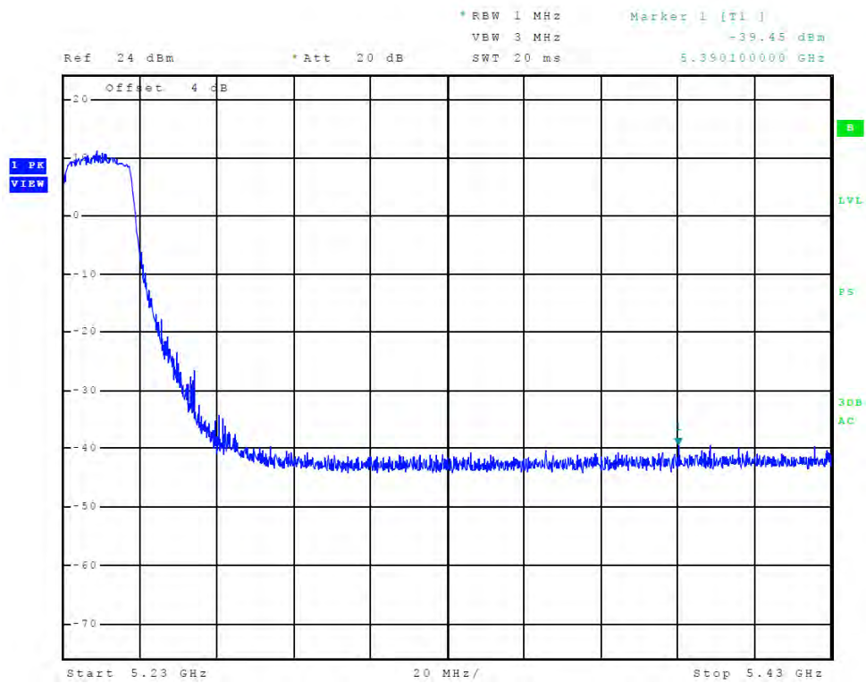
Figure 25 Plot of Transmitter High Band Edge (Chain 1, 5150-5250 MHz Band, 802.11n40)
