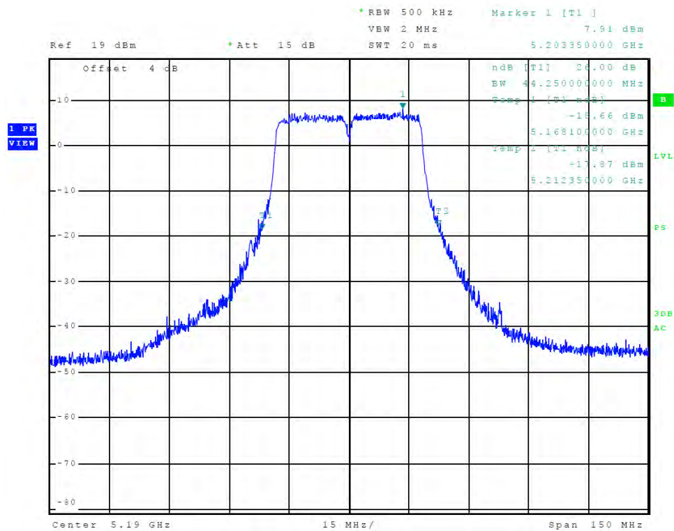
Figure 39 Plot of Transmitter Emissions (Chain 0, 5150-5250 MHz Band, 802.11n40, 26 dB OBW)
