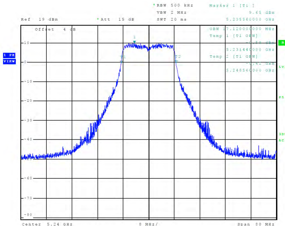
Figure 32 Plot of Transmitter Emissions (Chain 2, 5150-5250 MHz Band, 802.11a, 99% OBW)
