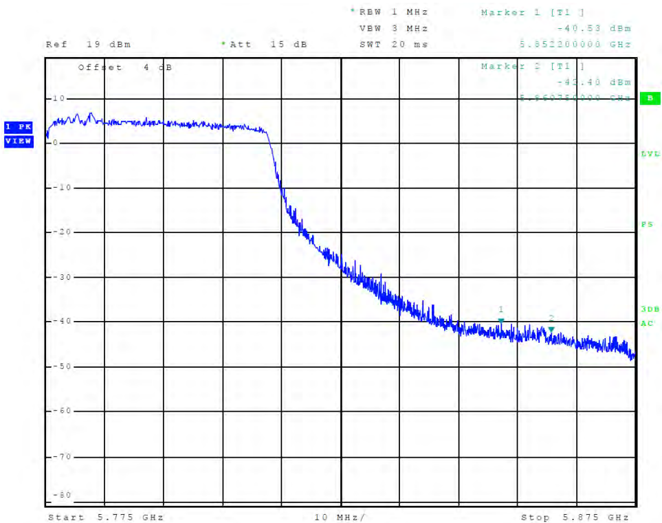
Figure 72 Plot of Transmitter High Band Edge (Chain 0, 5725-5850 MHz Band, 802.11ac)
