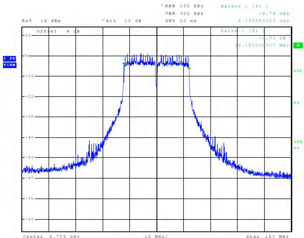
Figure 84 Plot of Transmitter Emissions (Chain 0, 5725-5850 MHz Band, 802.11n40, 6-dB OBW)
