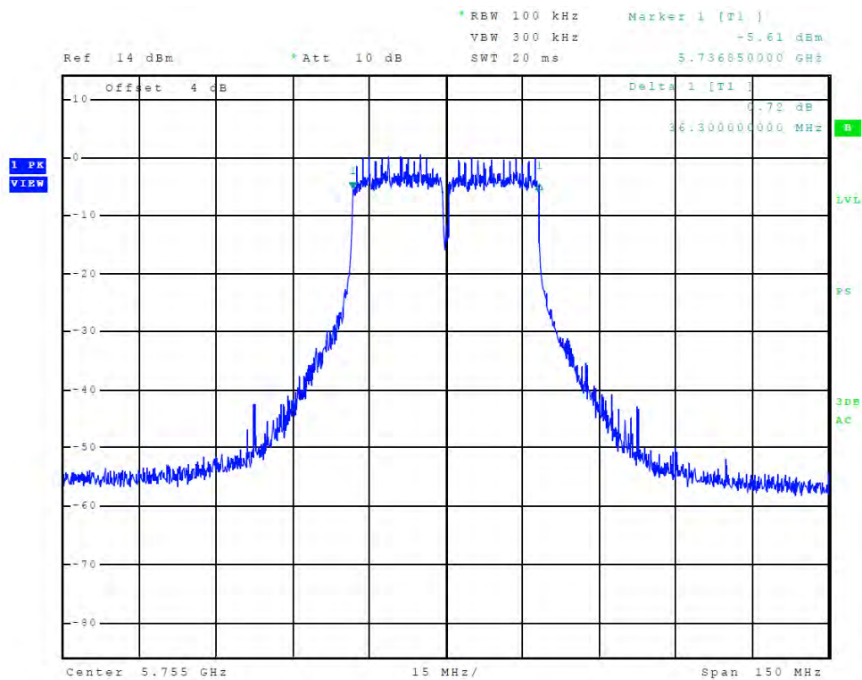
Figure 85 Plot of Transmitter Emissions (Chain 1, 5725-5850 MHz Band, 802.11n40, 6-dB OBW)
