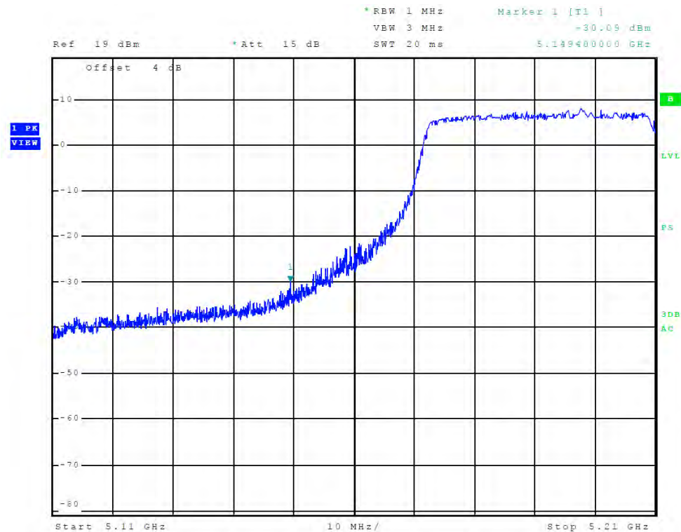
Figure 18 Plot of Transmitter Low Band Edge (Chain 0, 5150-5250 MHz Band, 802.11ac)
