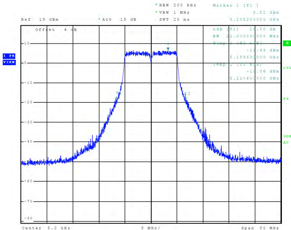
Figure 34 Plot of Transmitter Emissions (Chain 1, 5150-5250 MHz Band, 802.11a, 26 dB OBW)
