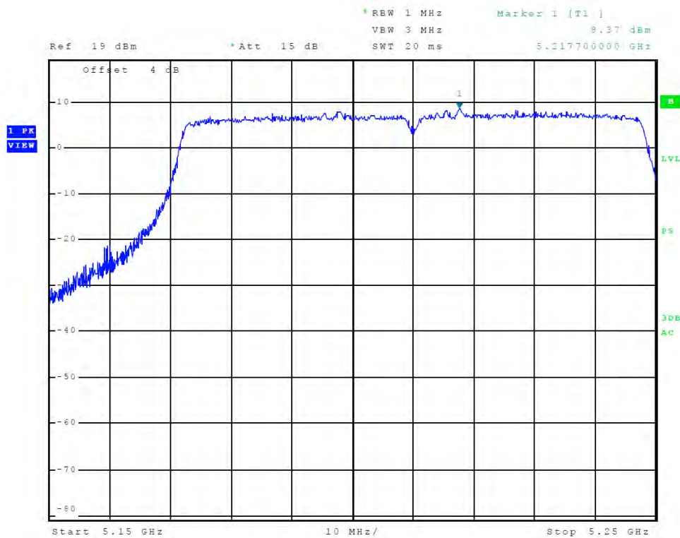
Figure 9 Plot of Transmitter Emissions (Chain 0, Across 5150-5250 MHz Band, 802.11ac)
