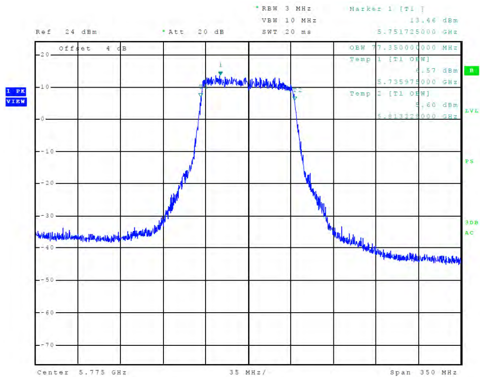
Figure 89 Plot of Transmitter Emissions (Chain 2, 5725-5850 MHz Band, 802.11ac, 99% OBW)
