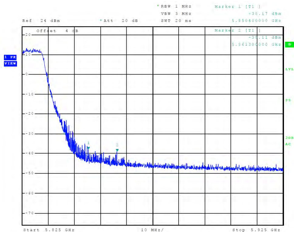
Figure 67 Plot of Transmitter High Band Edge (Chain 1, 5725-5850 MHz Band, 802.11a)
