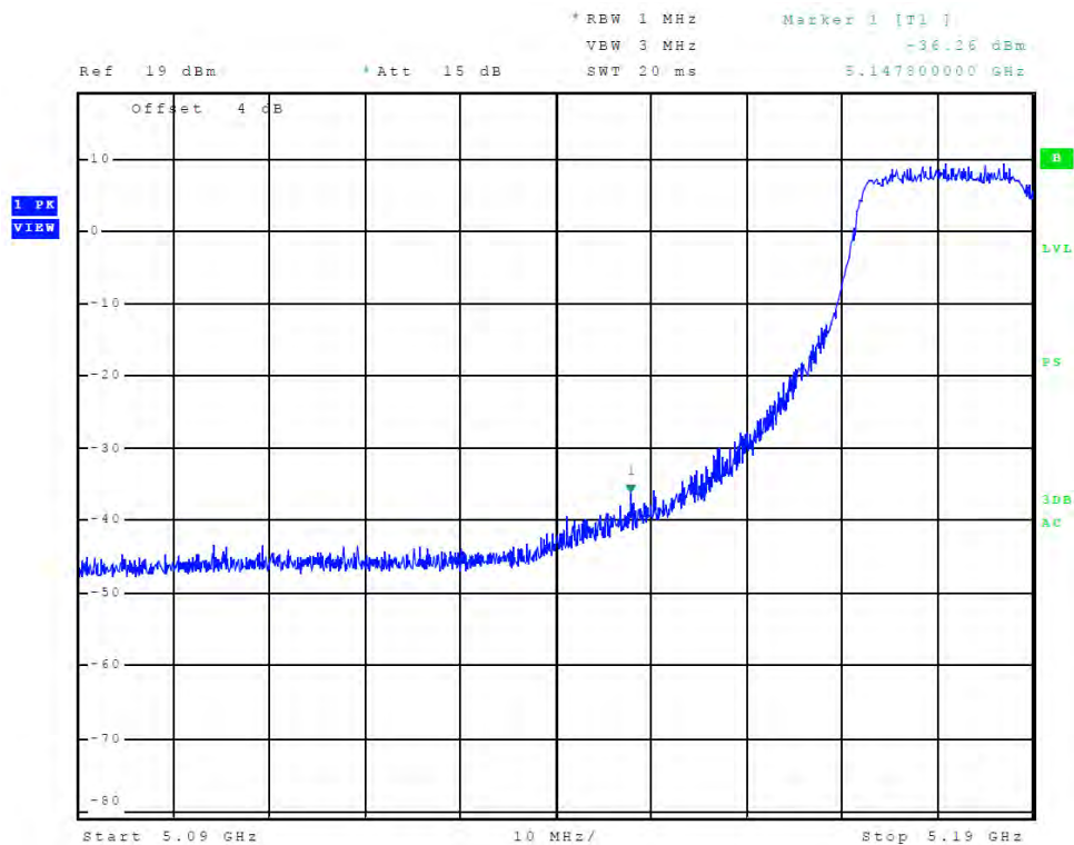
Figure 17 Plot of Transmitter Low Band Edge (Chain 2, 5150-5250 MHz Band, 802.11n40)
