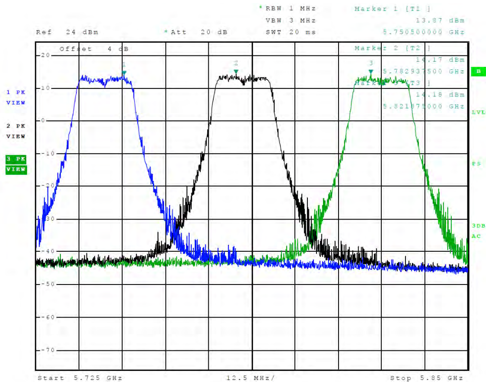
Figure 49 Plot of Transmitter Emissions (Chain 1, Across 5725-5850 MHz Band, 802.11a)
