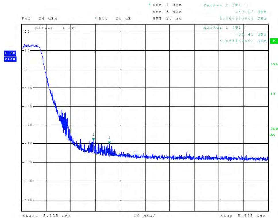
Figure 66 Plot of Transmitter High Band Edge (Chain 0, 5725-5850 MHz Band, 802.11a)
