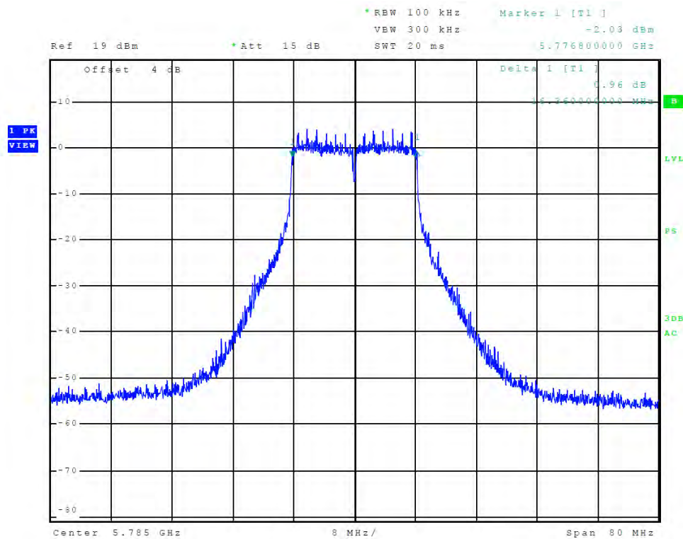
Figure 79 Plot of Transmitter Emissions (Chain 1, 5725-5850 MHz Band, 802.11a, 6-dB OBW)
