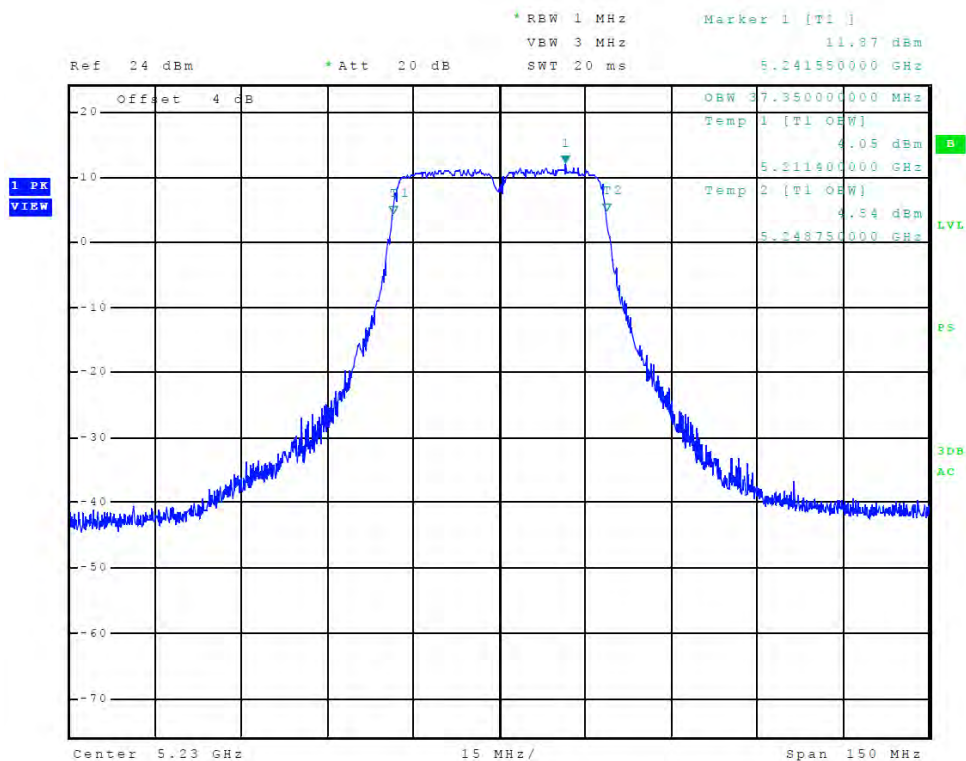
Figure 36 Plot of Transmitter Emissions (Chain 0, 5150-5250 MHz Band, 802.11n40, 99% OBW)
