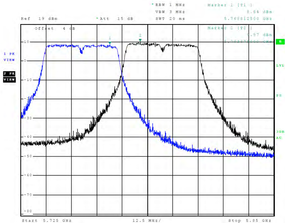
Figure 51 Plot of Transmitter Emissions (Chain 0, Across 5725-5850 MHz Band, 802.11n40)
