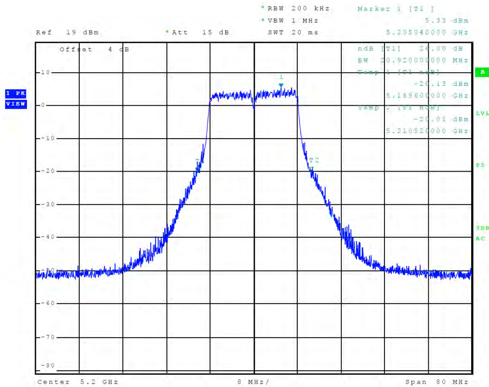
Figure 35 Plot of Transmitter Emissions (Chain 2, 5150-5250 MHz Band, 802.11a, 26 dB OBW)
