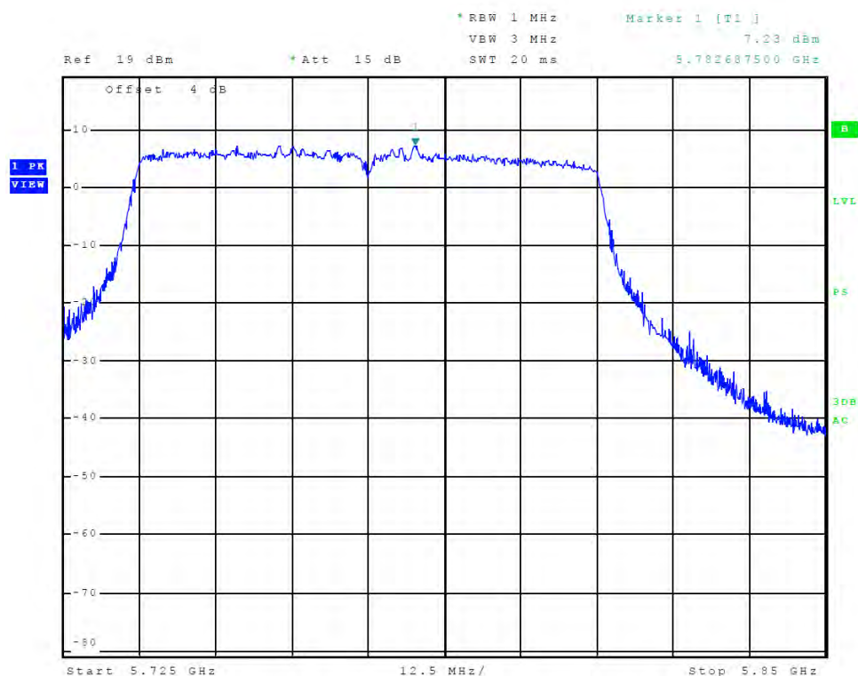
Figure 54 Plot of Transmitter Emissions (Chain 0, Across 5725-5850 MHz Band, 802.11ac)
