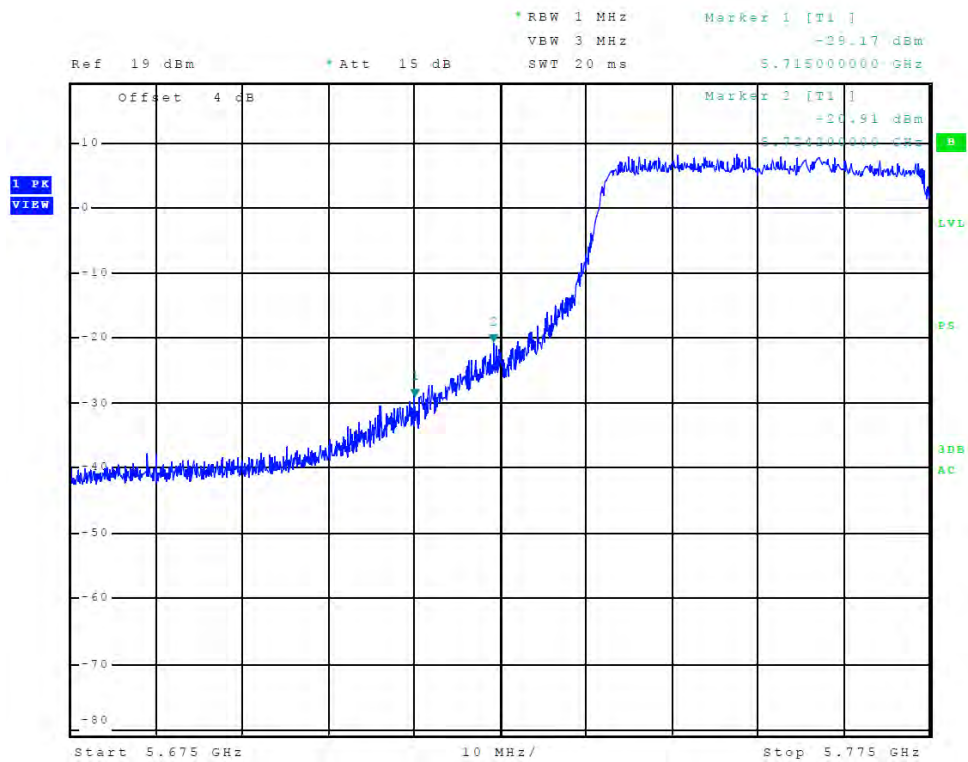
Figure 65 Plot of Transmitter Low Band Edge (Chain 2, 5725-5850 MHz Band, 802.11ac)
