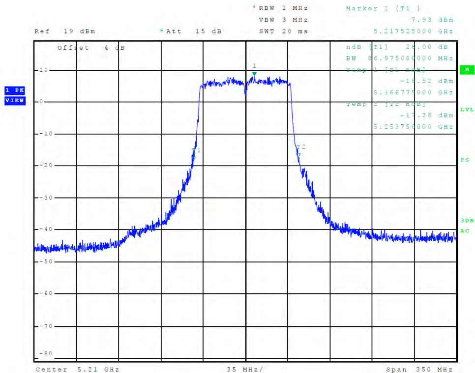
Figure 46 Plot of Transmitter Emissions (Chain 1, 5150-5250 MHz Band, 802.11ac, 26 dB OBW)
