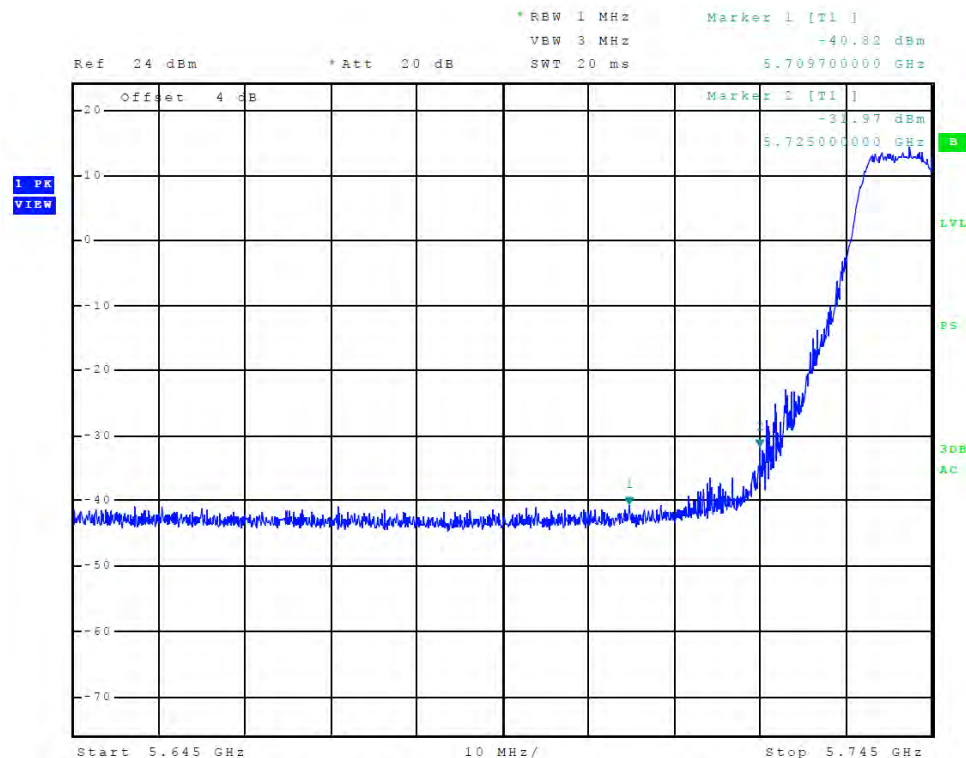
Figure 58 Plot of Transmitter Low Band Edge (Chain 1, 5725-5850 MHz Band, 802.11a)
