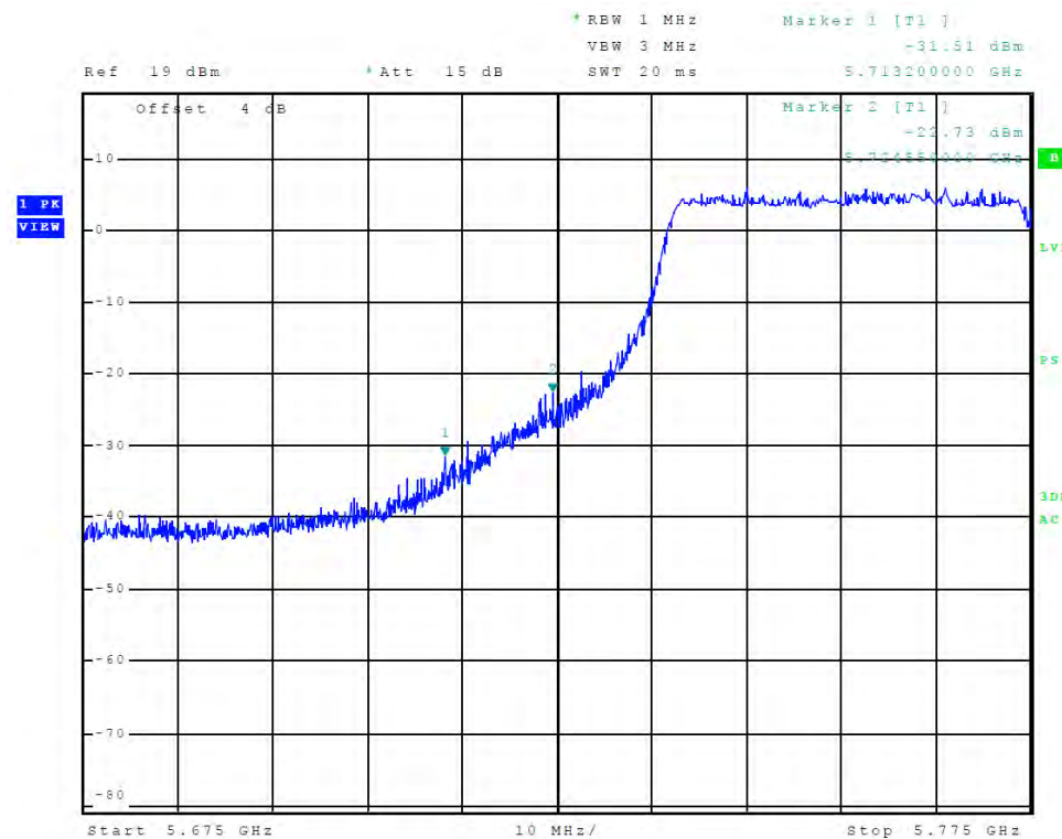
Figure 64 Plot of Transmitter Low Band Edge (Chain 1, 5725-5850 MHz Band, 802.11ac)
