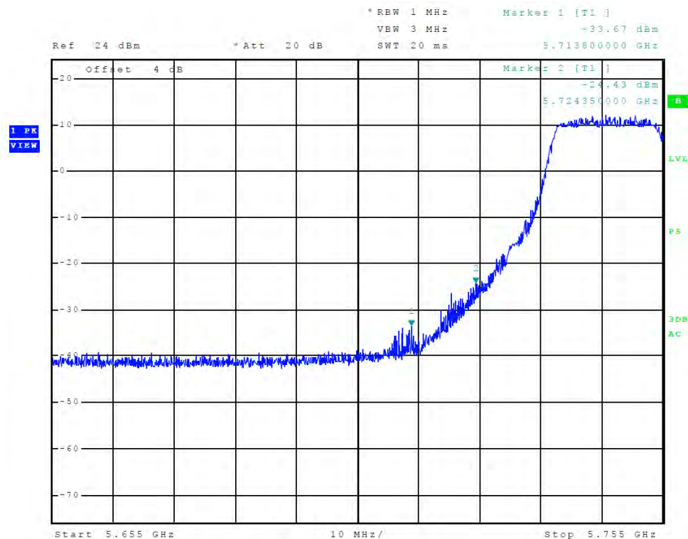
Figure 62 Plot of Transmitter Low Band Edge (Chain 2, 5725-5850 MHz Band, 802.11n40)
