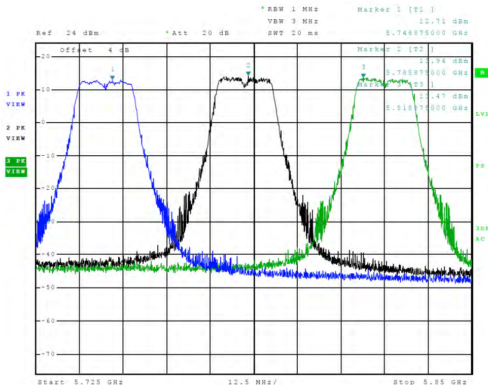
Figure 48 Plot of Transmitter Emissions (Chain 0, Across 5725-5850 MHz Band, 802.11a)
