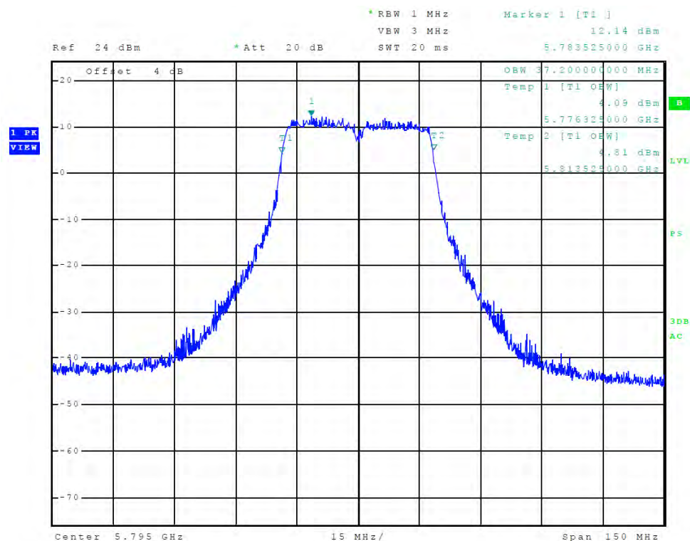
Figure 83 Plot of Transmitter Emissions (Chain 2, 5725-5850 MHz Band, 802.11n40, 99% OBW)
