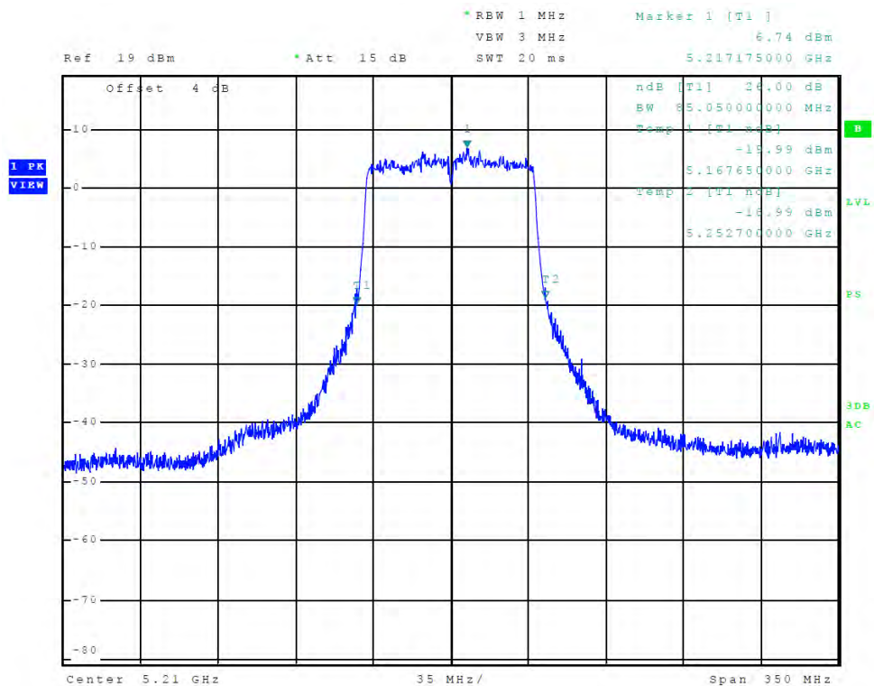
Figure 47 Plot of Transmitter Emissions (Chain 2, 5150-5250 MHz Band, 802.11ac, 26 dB OBW)
