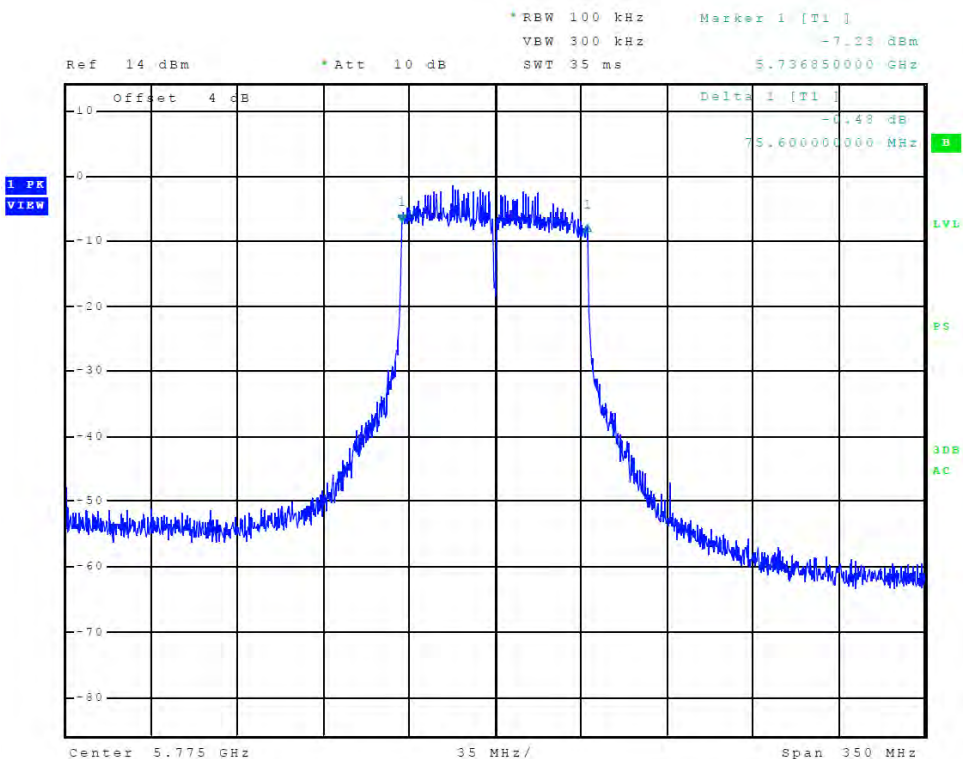
Figure 92 Plot of Transmitter Emissions (Chain 2, 5725-5850 MHz Band, 802.11ac, 6-dB OBW)
