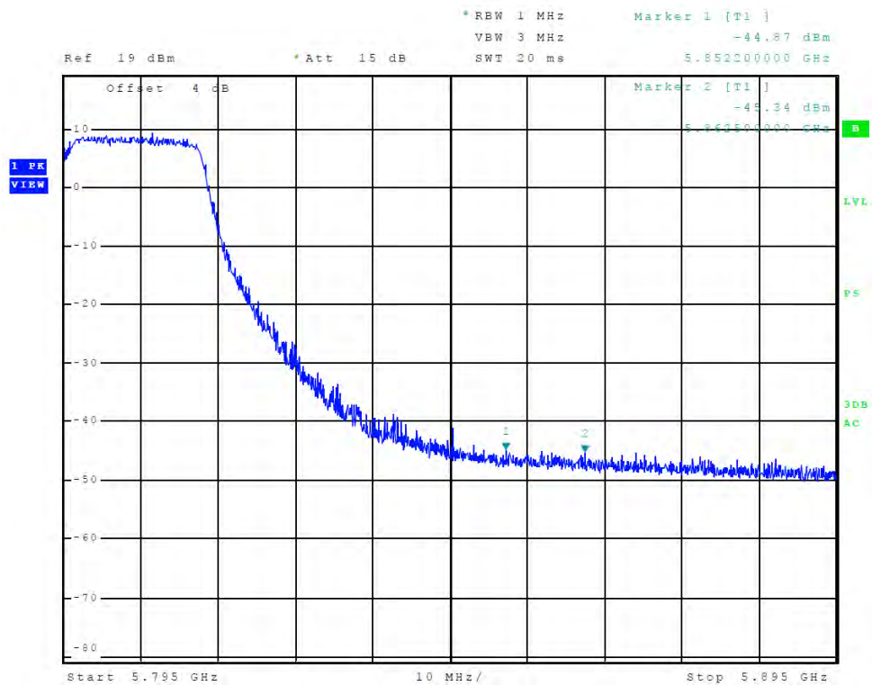
Figure 69 Plot of Transmitter High Band Edge (Chain 0, 5725-5850 MHz Band, 802.11n40)
