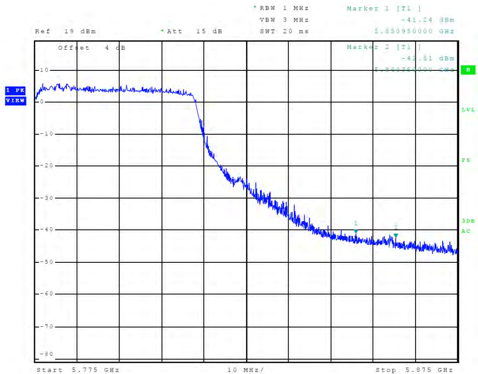
Figure 73 Plot of Transmitter High Band Edge (Chain 1, 5725-5850 MHz Band, 802.11ac)
