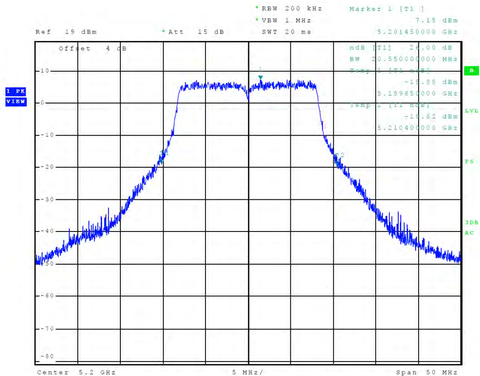
Figure 33 Plot of Transmitter Emissions (Chain 0, 5150-5250 MHz Band, 802.11a, 26 dB OBW)
