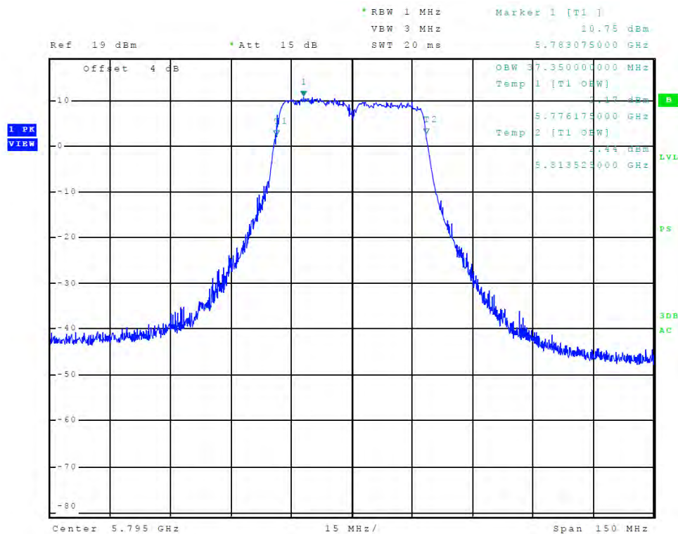
Figure 81 Plot of Transmitter Emissions (Chain 0, 5725-5850 MHz Band, 802.11n40, 99% OBW)
