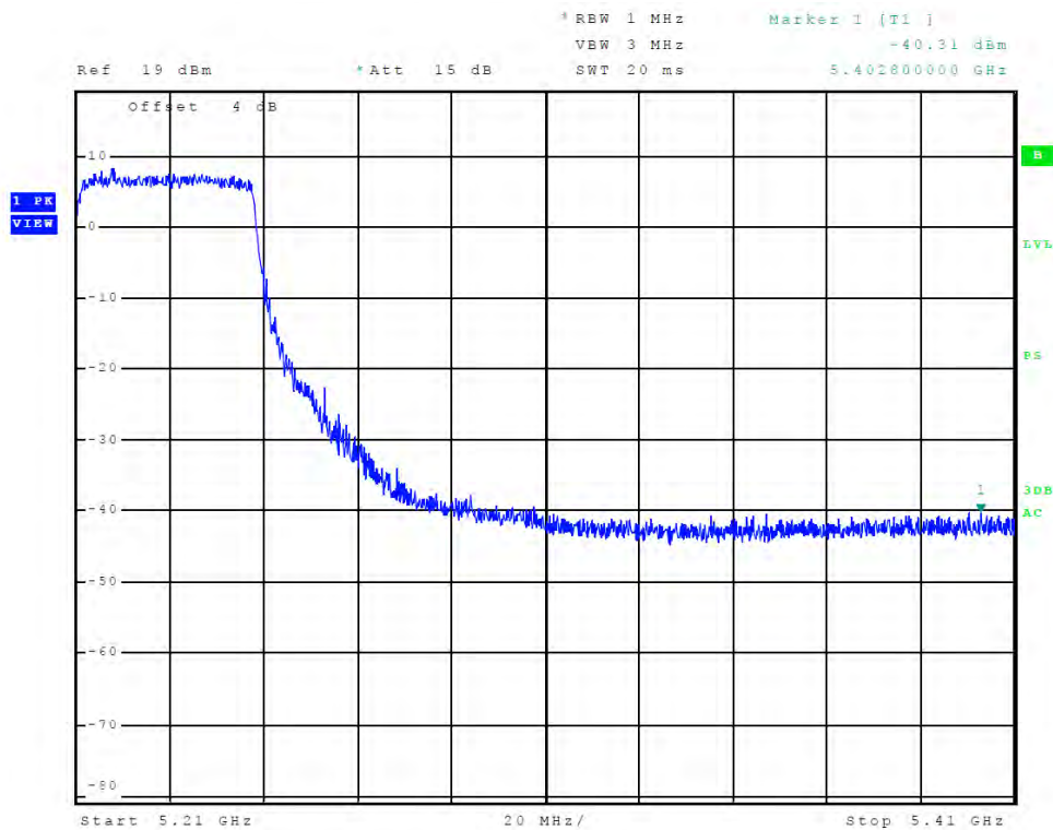
Figure 27 Plot of Transmitter High Band Edge (Chain 0, 5150-5250 MHz Band, 802.11ac)
