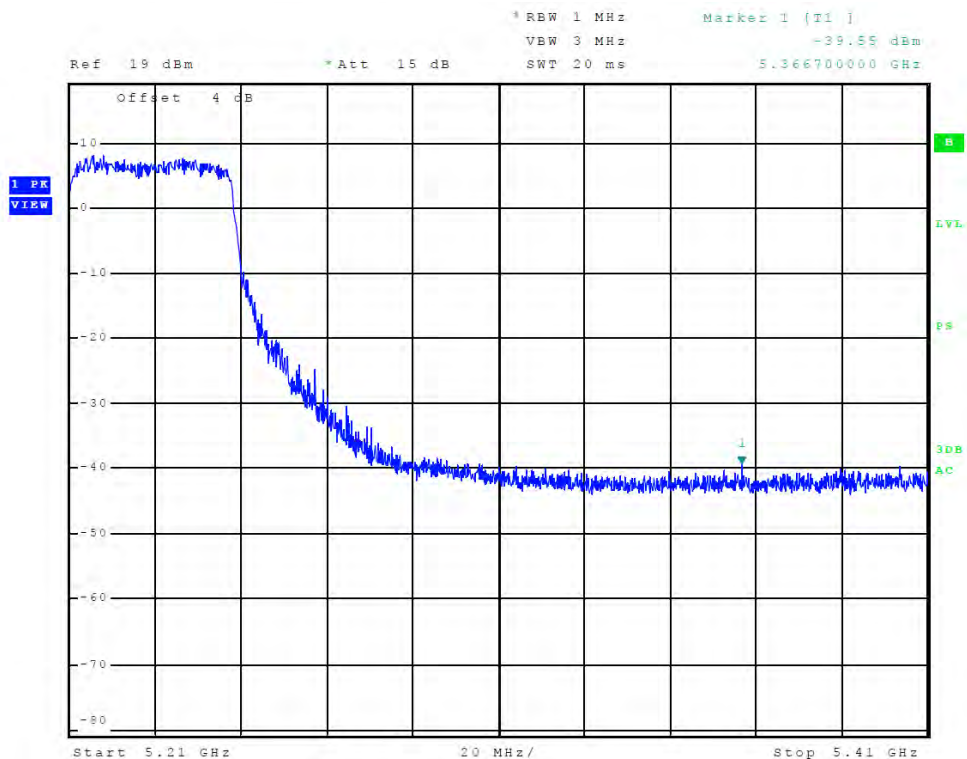
Figure 28 Plot of Transmitter High Band Edge (Chain 1, 5150-5250 MHz Band, 802.11ac)
