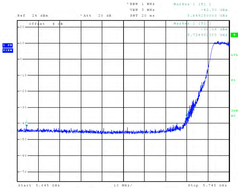
Figure 59 Plot of Transmitter Low Band Edge (Chain 2, 5725-5850 MHz Band, 802.11a)
