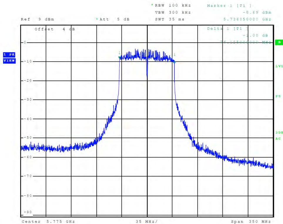
Figure 91 Plot of Transmitter Emissions (Chain 1, 5725-5850 MHz Band, 802.11ac, 6-dB OBW)
