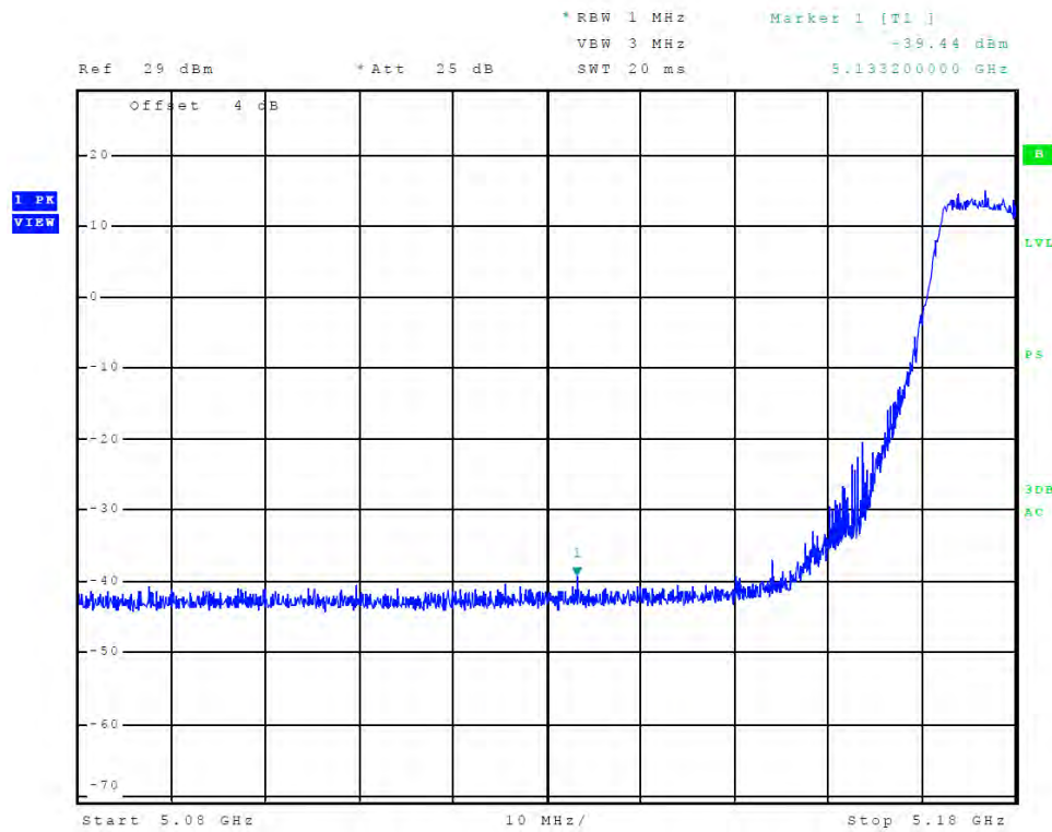
Figure 13 Plot of Transmitter Low Band Edge (Chain 1, 5150-5250 MHz Band, 802.11a)
