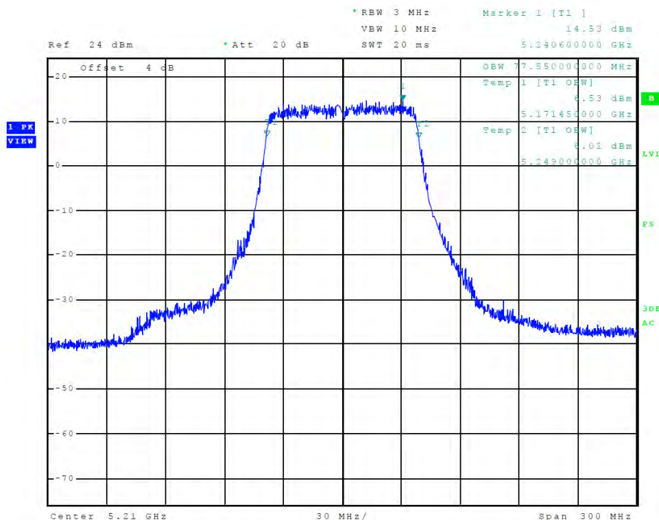
Figure 42 Plot of Transmitter Emissions (Chain 0, 5150-5250 MHz Band, 802.11ac, 99% OBW)
