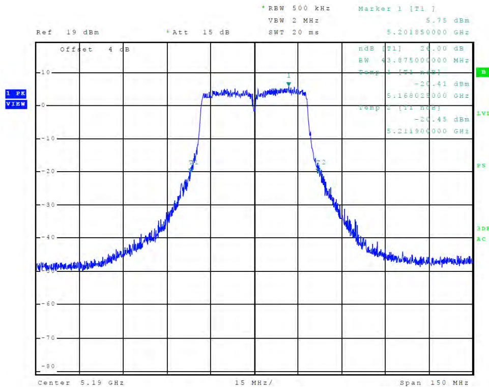
Figure 41 Plot of Transmitter Emissions (Chain 2, 5150-5250 MHz Band, 802.11n40, 26 dB OBW)
