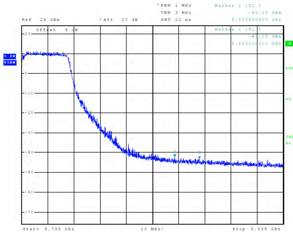
Figure 71 Plot of Transmitter High Band Edge (Chain 2, 5725-5850 MHz Band, 802.11n40)
