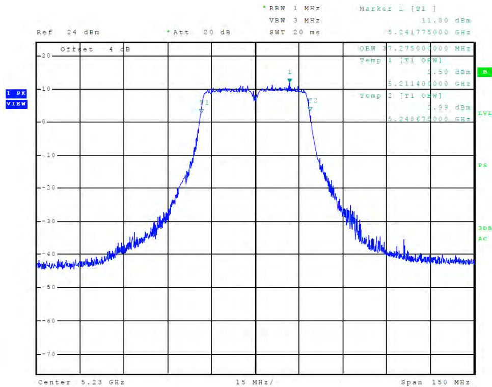
Figure 37 Plot of Transmitter Emissions (Chain 1, 5150-5250 MHz Band, 802.11n40, 99% OBW)
