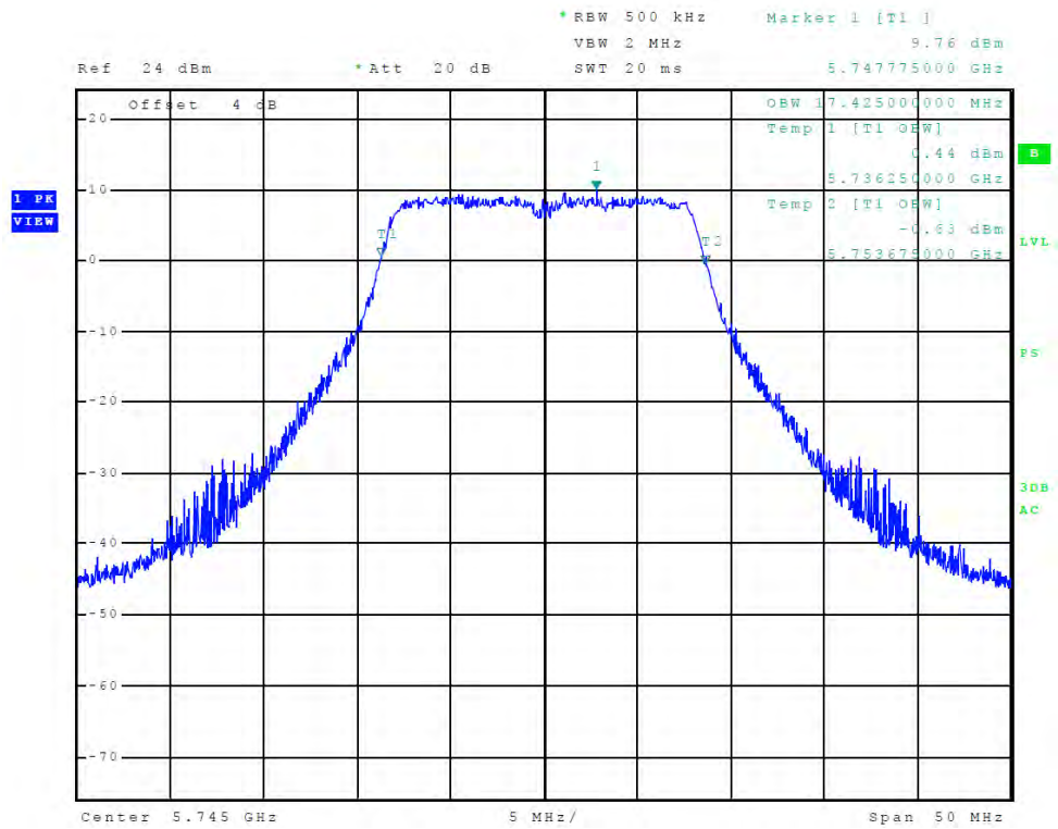
Figure 75 Plot of Transmitter Emissions (Chain 0, 5725-5850 MHz Band, 802.11a, 99% OBW)
