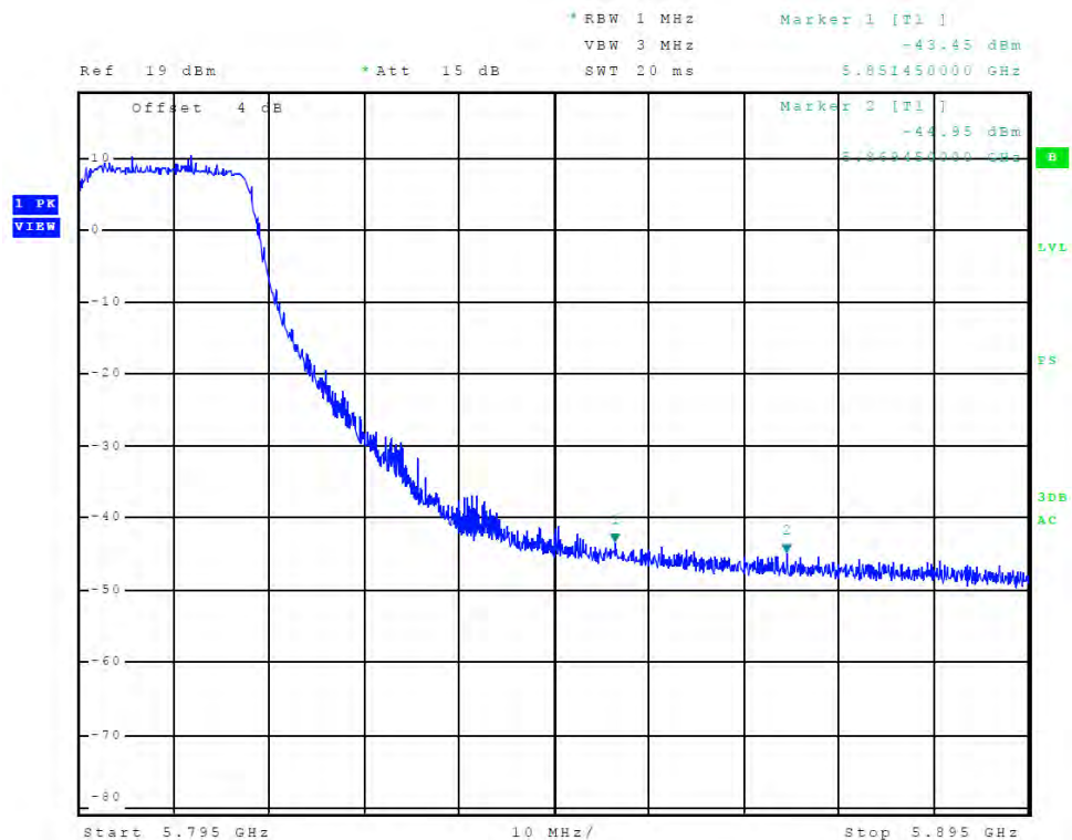
Figure 70 Plot of Transmitter High Band Edge (Chain 1, 5725-5850 MHz Band, 802.11n40)
