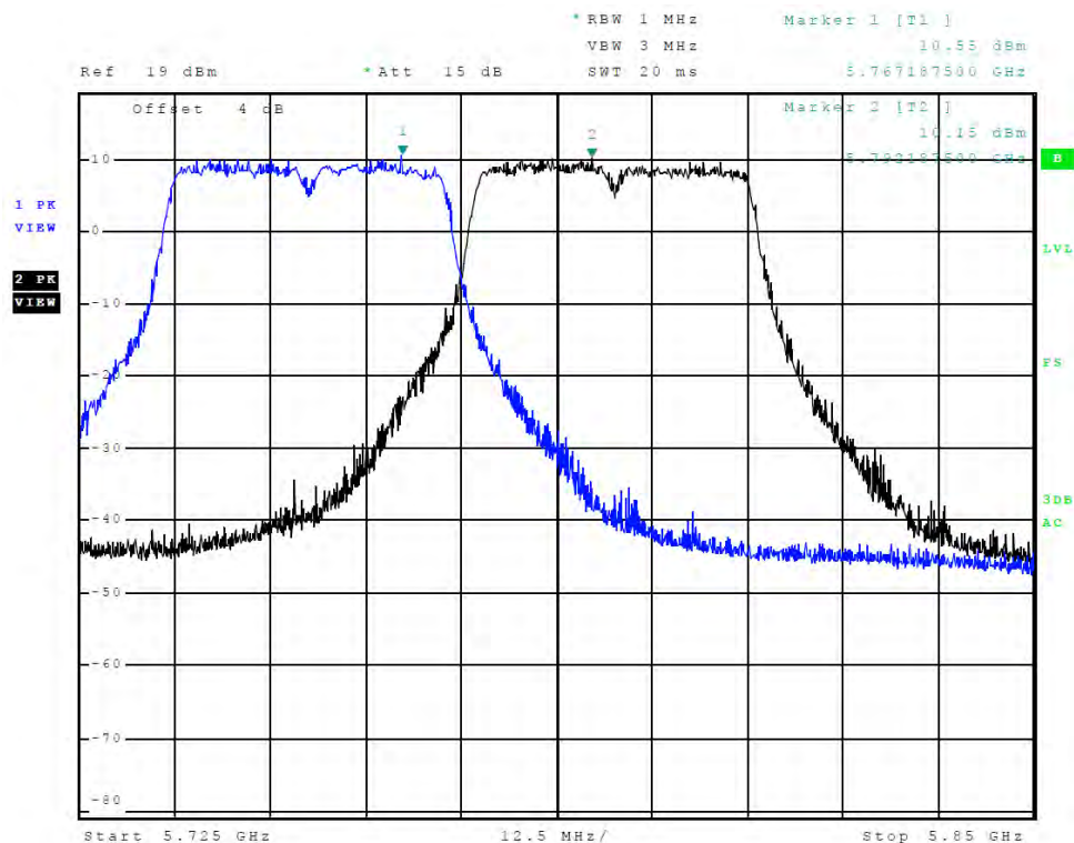
Figure 52 Plot of Transmitter Emissions (Chain 1, Across 5725-5850 MHz Band, 802.11n40)
