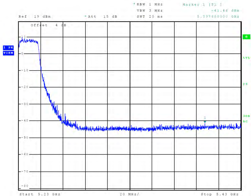
Figure 26 Plot of Transmitter High Band Edge (Chain 2, 5150-5250 MHz Band, 802.11n40)
