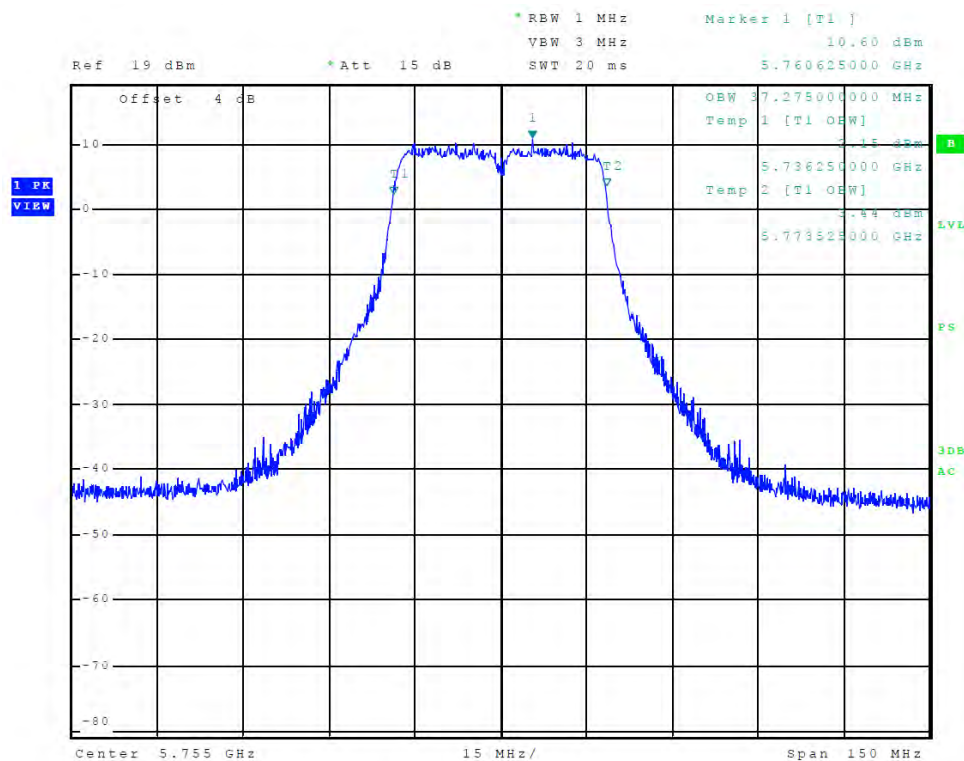
Figure 82 Plot of Transmitter Emissions (Chain 1, 5725-5850 MHz Band, 802.11n40, 99% OBW)
