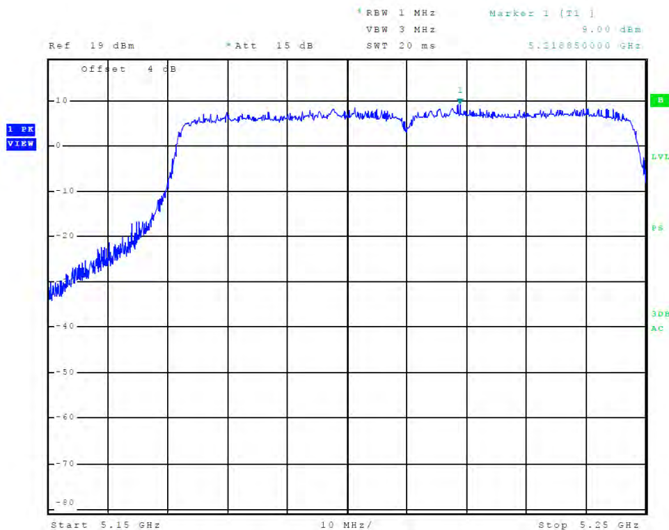
Figure 10 Plot of Transmitter Emissions (Chain 1, Across 5150-5250 MHz Band, 802.11ac)
