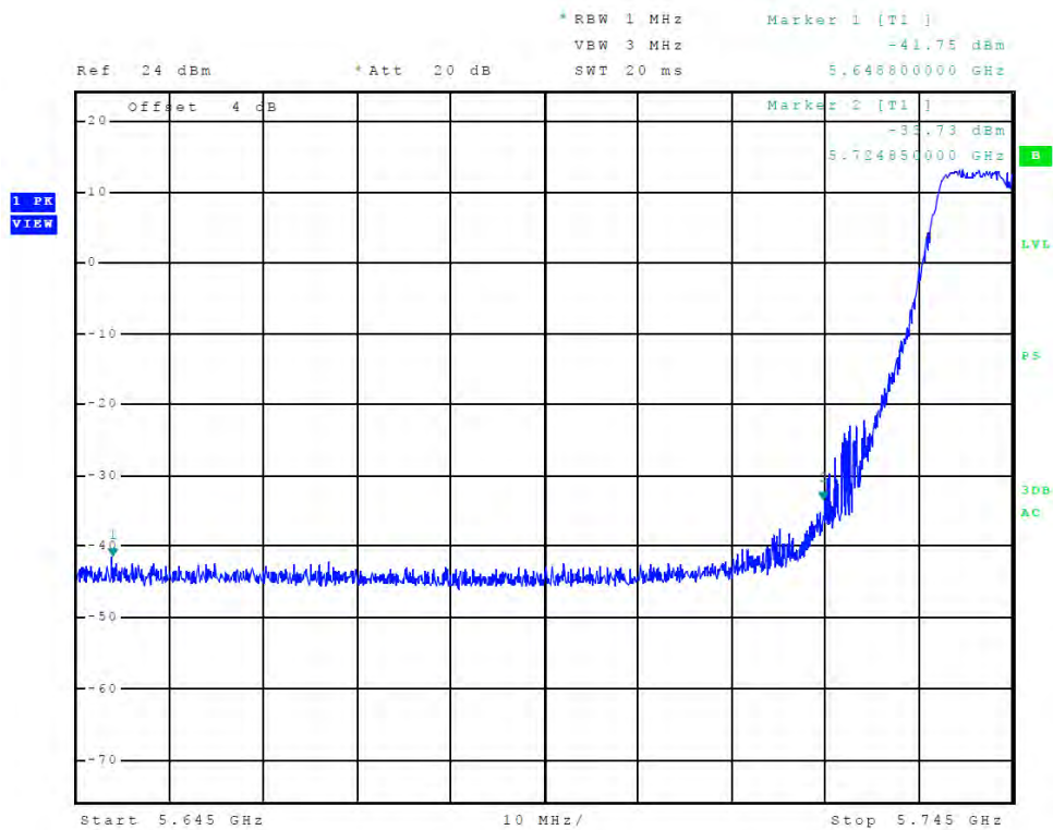
Figure 57 Plot of Transmitter Low Band Edge (Chain 0, 5725-5850 MHz Band, 802.11a)
