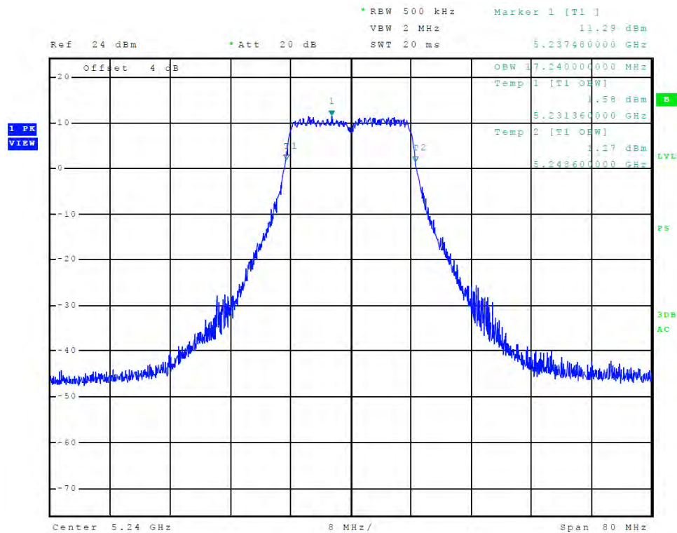
Figure 31 Plot of Transmitter Emissions (Chain 1, 5150-5250 MHz Band, 802.11a, 99% OBW)
