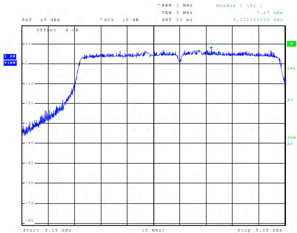
Figure 11 Plot of Transmitter Emissions (Chain 2, Across 5150-5250 MHz Band, 802.11ac)
