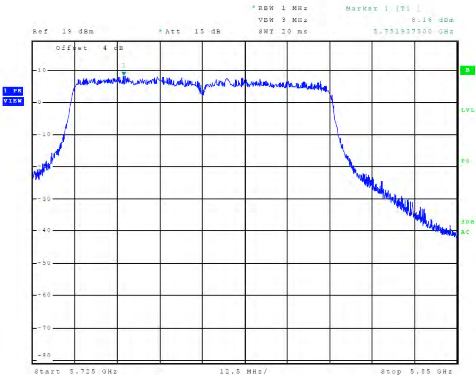
Figure 56 Plot of Transmitter Emissions (Chain 2, Across 5725-5850 MHz Band, 802.11ac)
