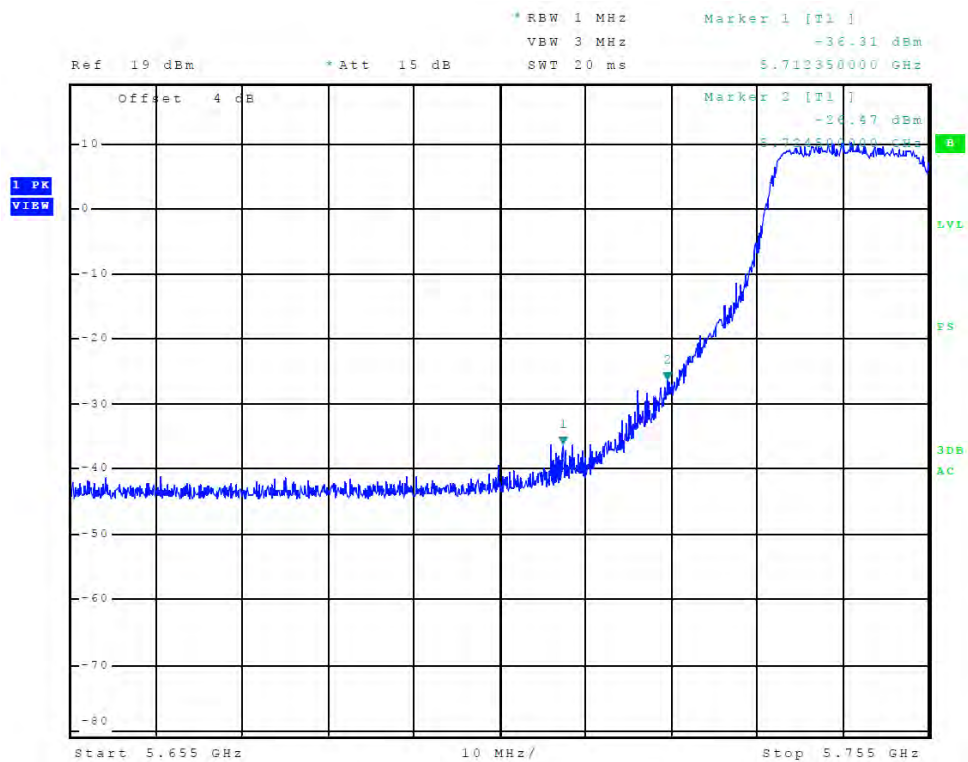
Figure 61 Plot of Transmitter Low Band Edge (Chain 1, 5725-5850 MHz Band, 802.11n40)
