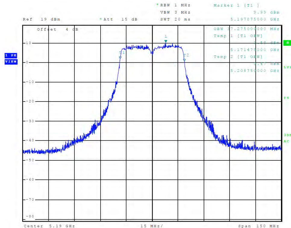
Figure 38 Plot of Transmitter Emissions (Chain 2, 5150-5250 MHz Band, 802.11n40, 99% OBW)
