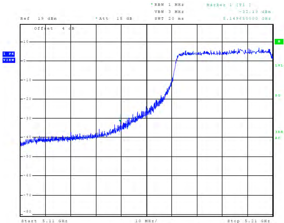
Figure 20 Plot of Transmitter Low Band Edge (Chain 2, 5150-5250 MHz Band, 802.11ac)
