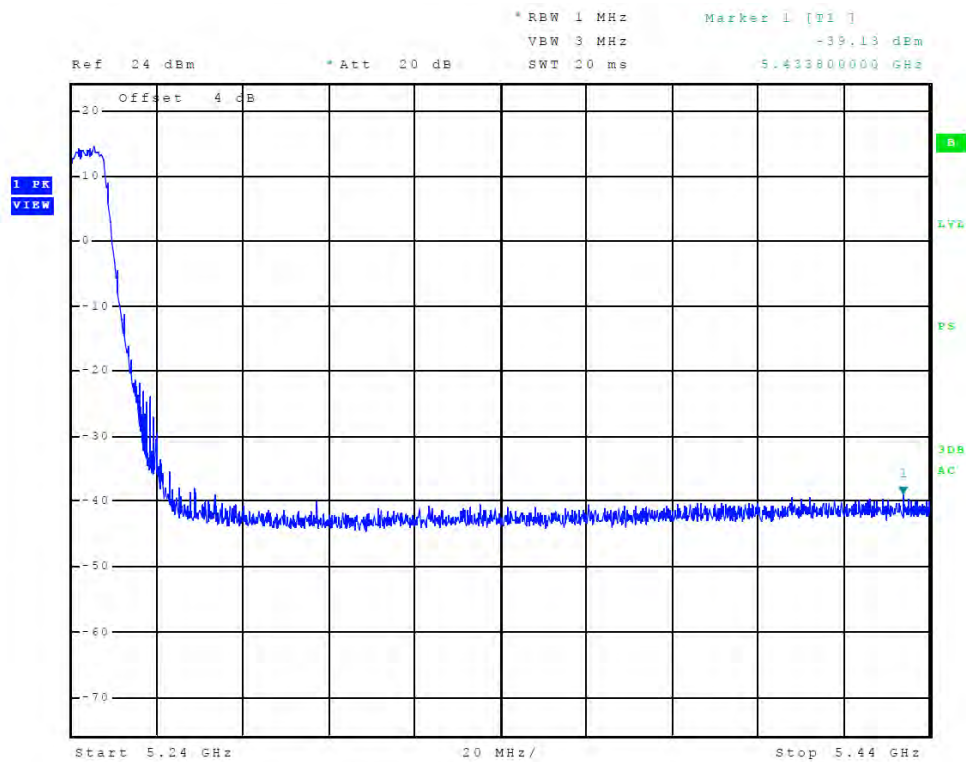
Figure 21 Plot of Transmitter High Band Edge (Chain 0, 5150-5250 MHz Band, 802.11a)
