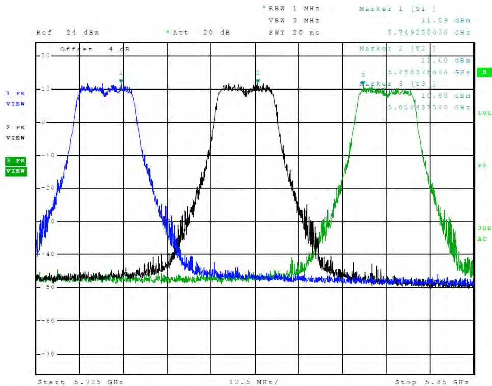
Figure 50 Plot of Transmitter Emissions (Chain 2, Across 5725-5850 MHz Band, 802.11a)
