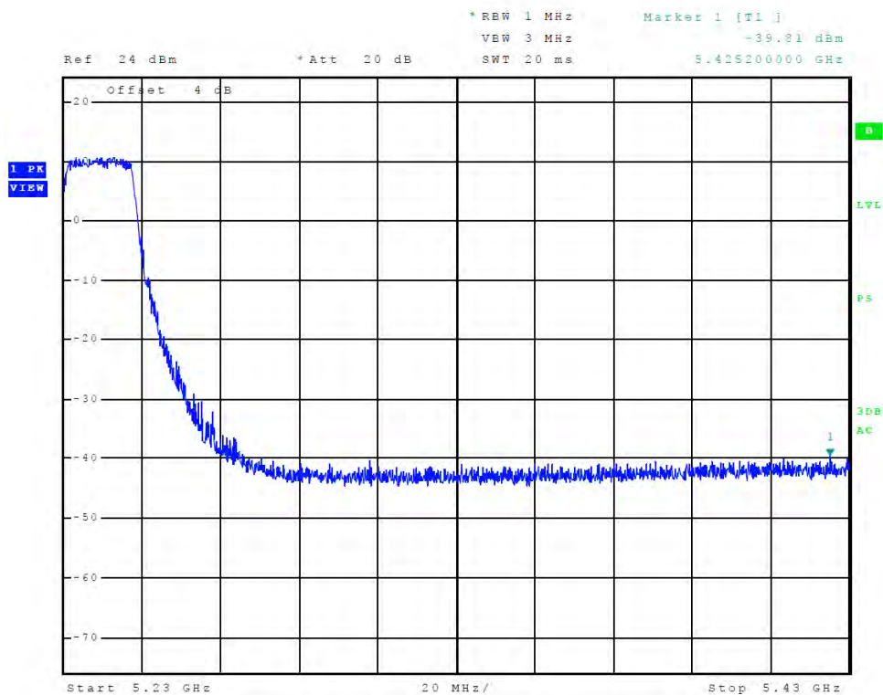
Figure 24 Plot of Transmitter High Band Edge (Chain 0, 5150-5250 MHz Band, 802.11n40)
