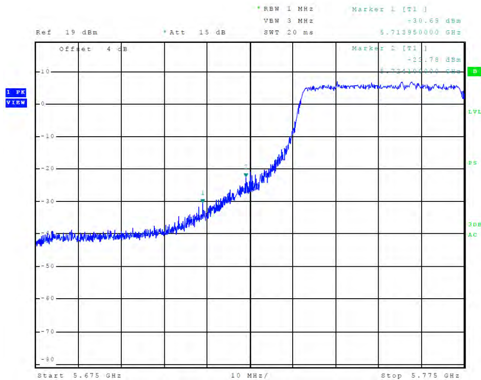
Figure 63 Plot of Transmitter Low Band Edge (Chain 0, 5725-5850 MHz Band, 802.11ac)
