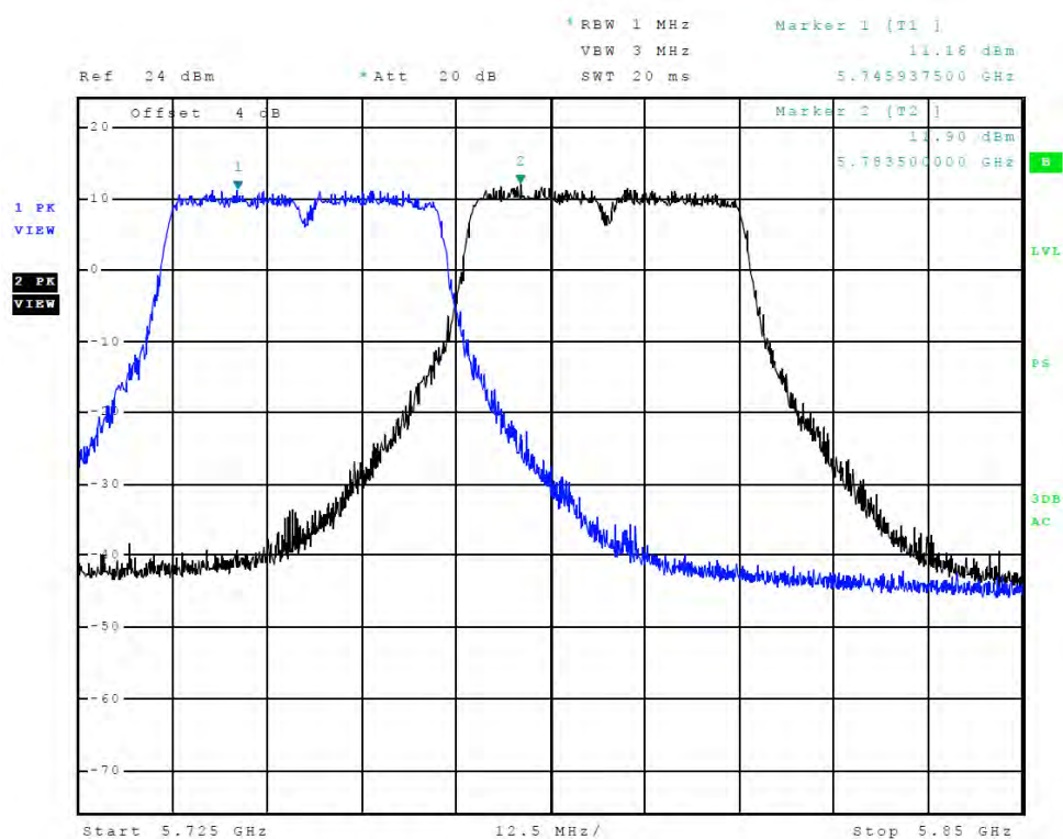
Figure 53 Plot of Transmitter Emissions (Chain 2, Across 5725-5850 MHz Band, 802.11n40)
