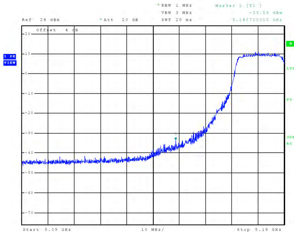
Figure 16 Plot of Transmitter Low Band Edge (Chain 1, 5150-5250 MHz Band, 802.11n40)
