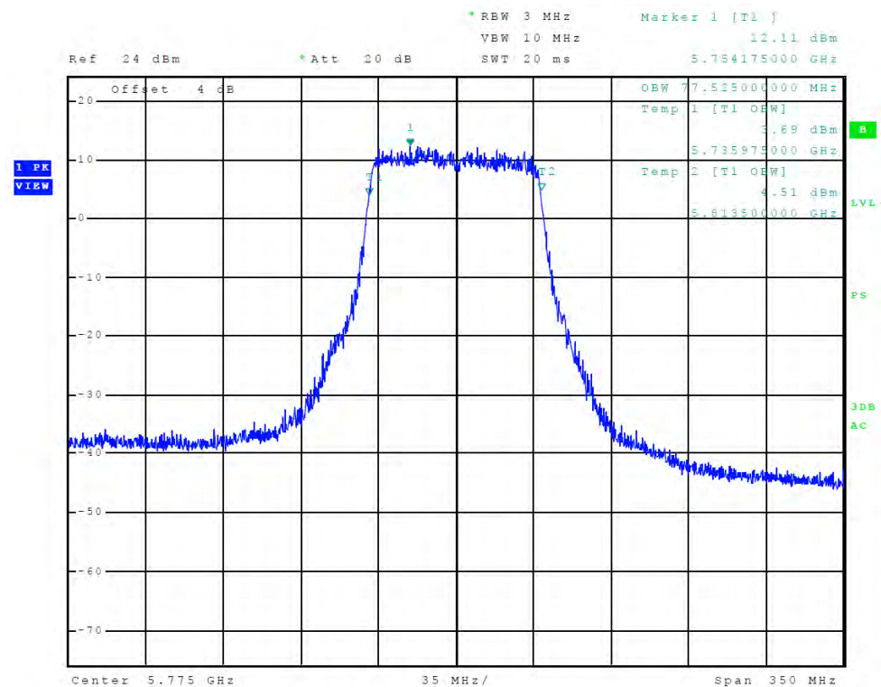
Figure 88 Plot of Transmitter Emissions (Chain 1, 5725-5850 MHz Band, 802.11ac, 99% OBW)
